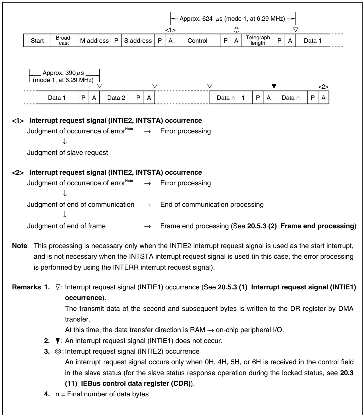
Figure 20-28. Slave Transmission
