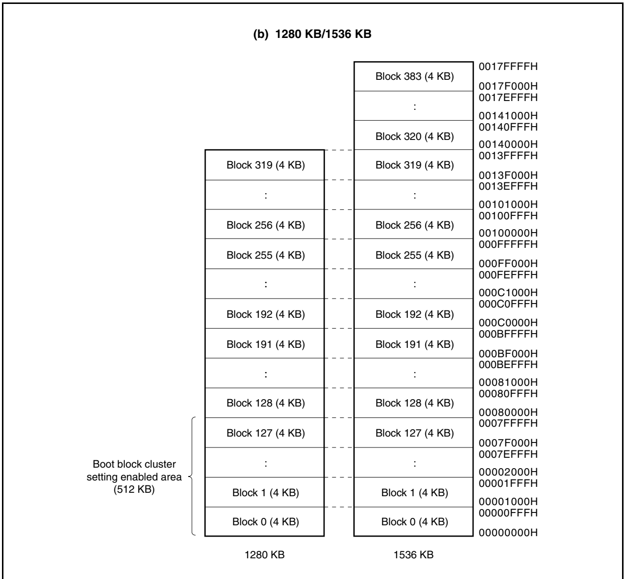
Figure 32-1. Flash Memory Mapping (2/2)
