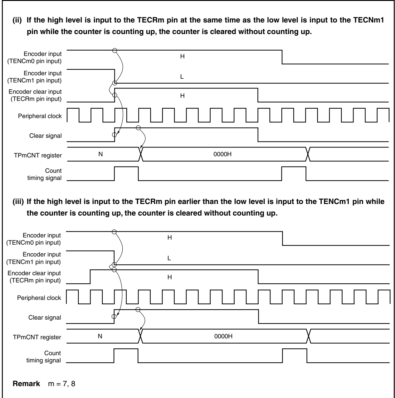
Figure 7-53. Operation Example (When TPmSCE Bit = 1, TPmZCL Bit = 1, TPmBCL Bit = 0, TPmACL Bit = 1, TPmUDS1 and TPmUDS0 Bits = 11, TECRm = High Level, TENCm1 = Low Level, and TENCm0 = High Level) (2/3)
