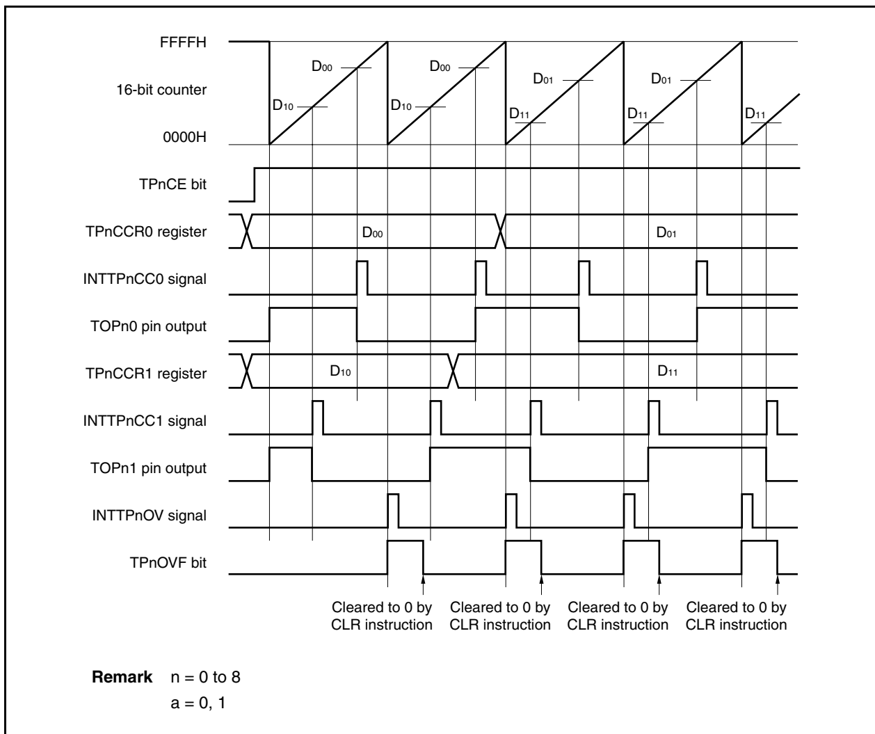
Figure 7-35. Basic Timing in Free-Running Timer Mode (Compare Function)
