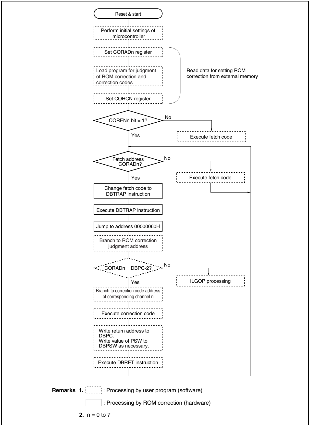
Figure 31-2. ROM Correction Operation and Program Flow
