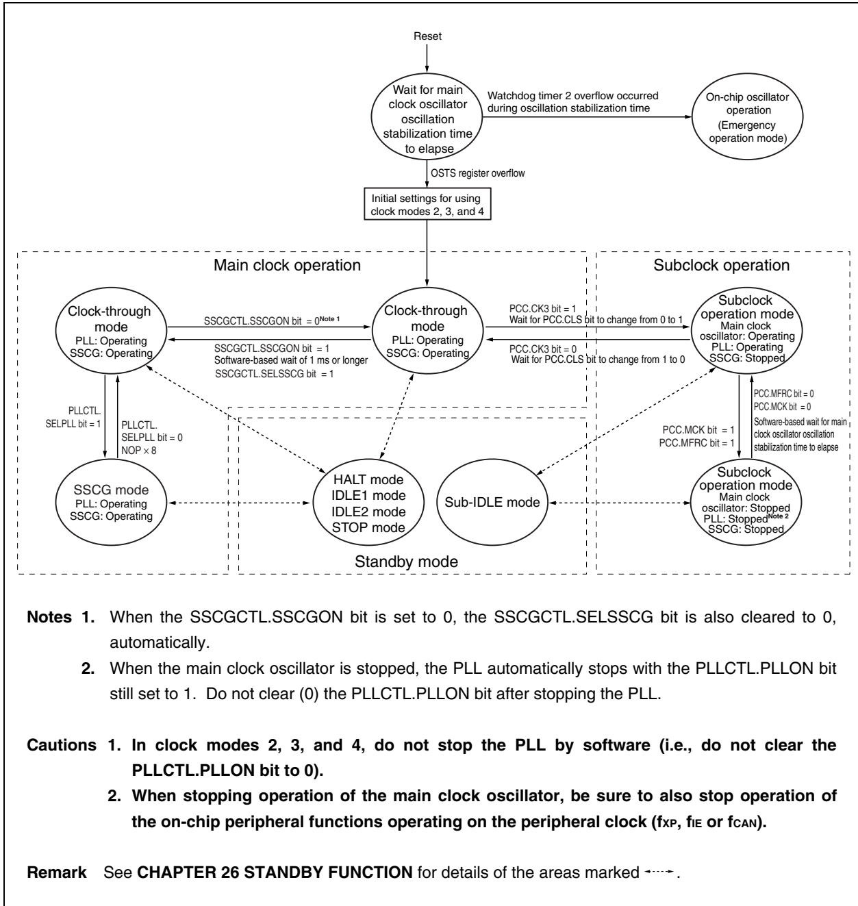
Figure 6-6. Procedure for Setting Clock Generation Function for Using Clock Modes 2, 3, and 4
