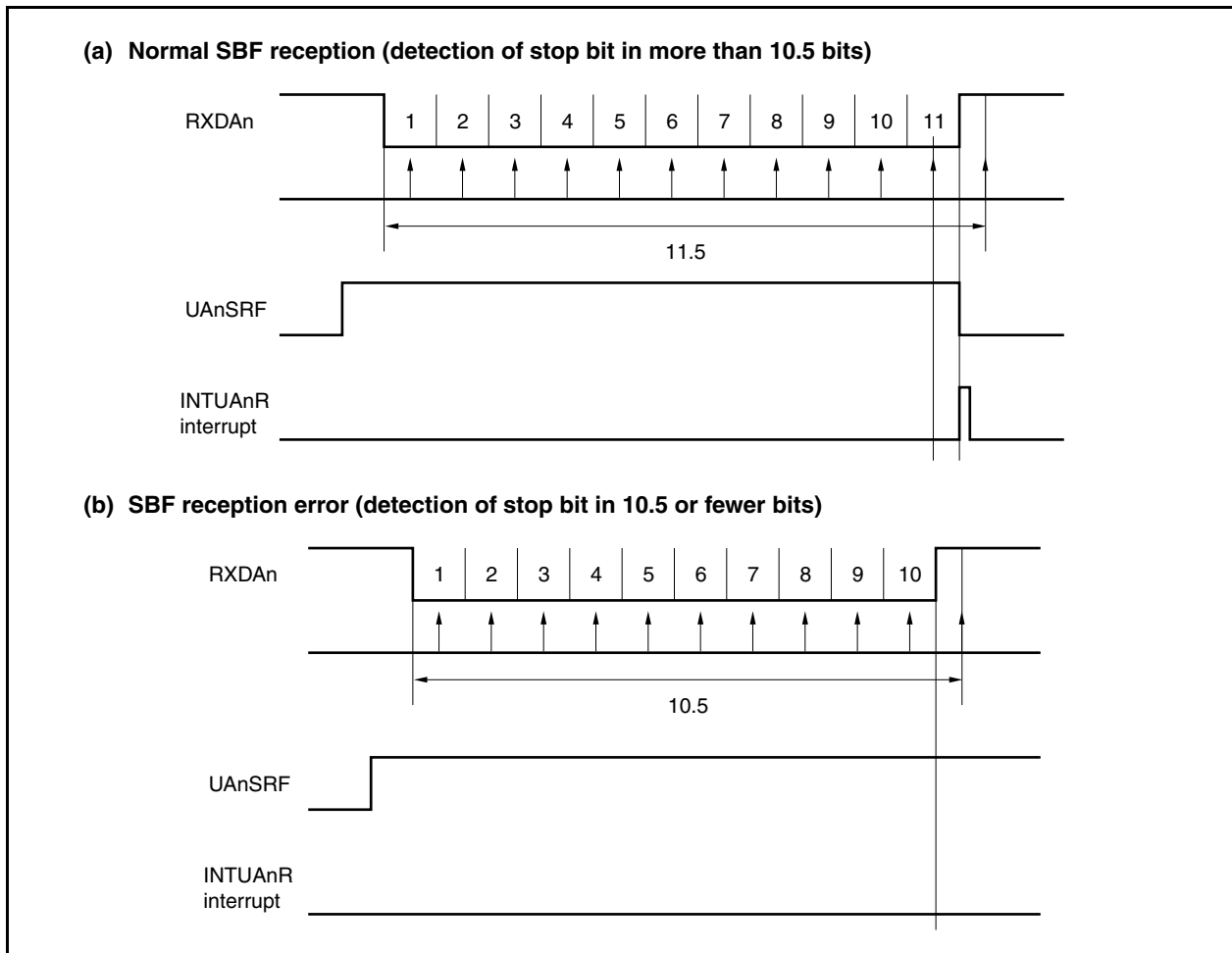
Figure 15-6. SBF Reception
