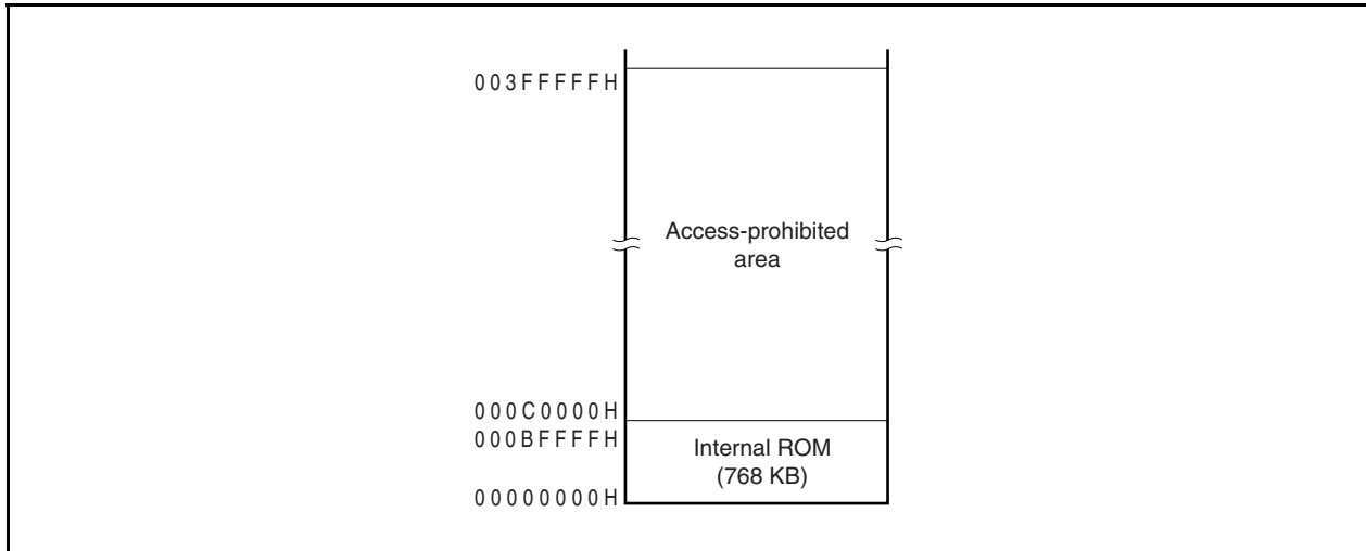
Figure 3-5. Internal ROM Area (768 KB)
