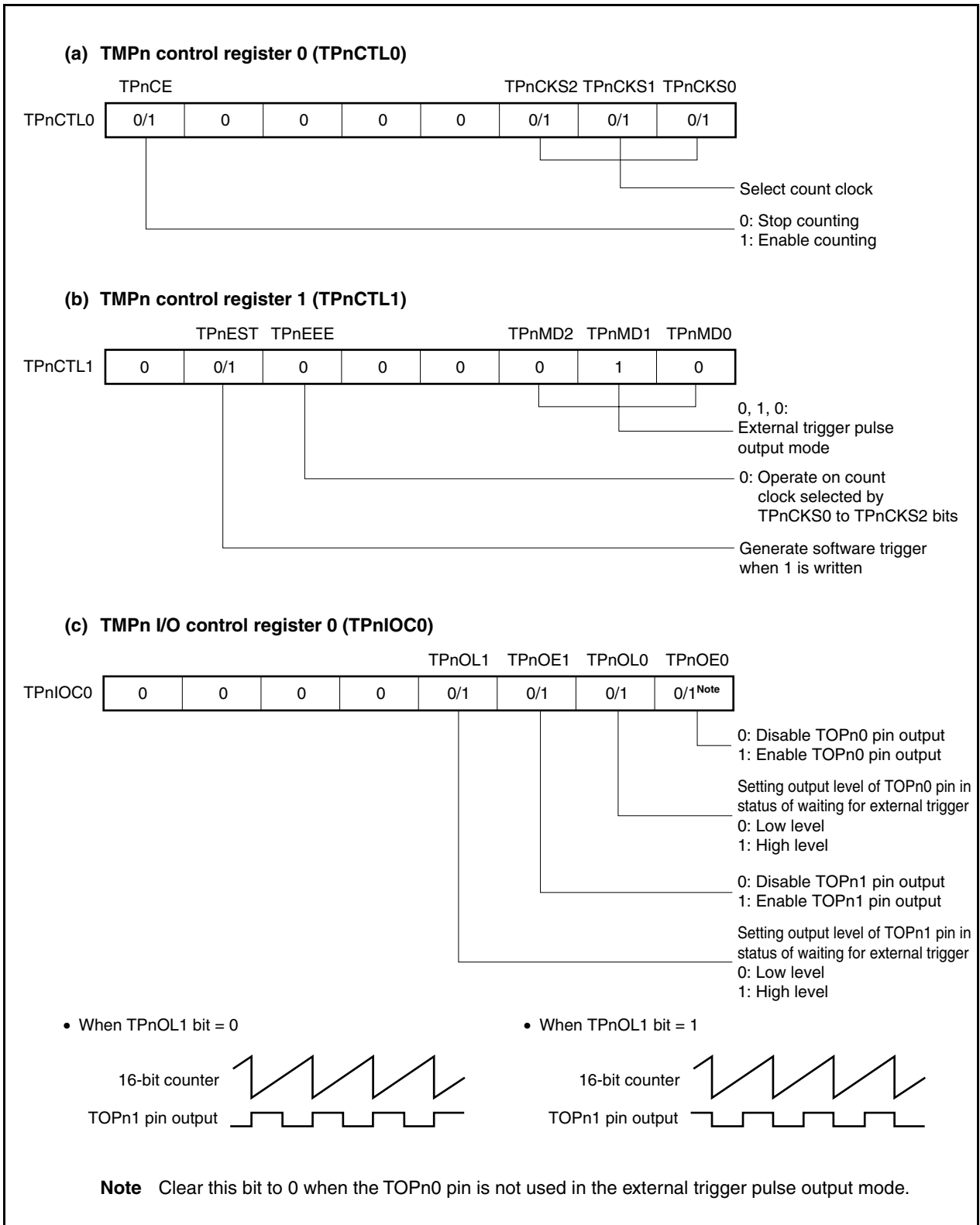
Figure 7-24. Setting of Registers in External Trigger Pulse Output Mode (1/2)
