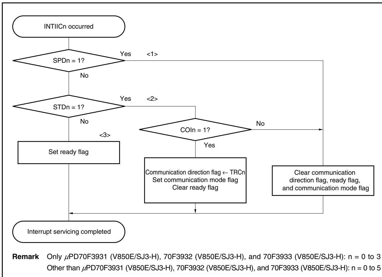
Figure 19-19. Slave Operation Flowchart (2)
