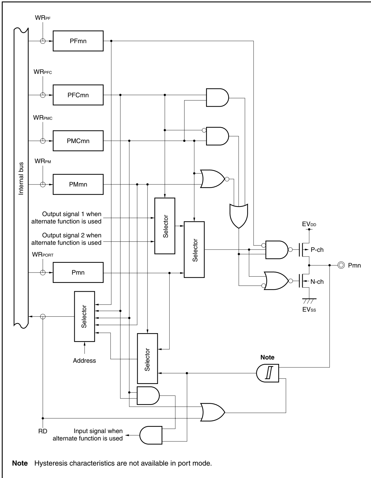
Figure 4-22. Block Diagram of Type G-6
