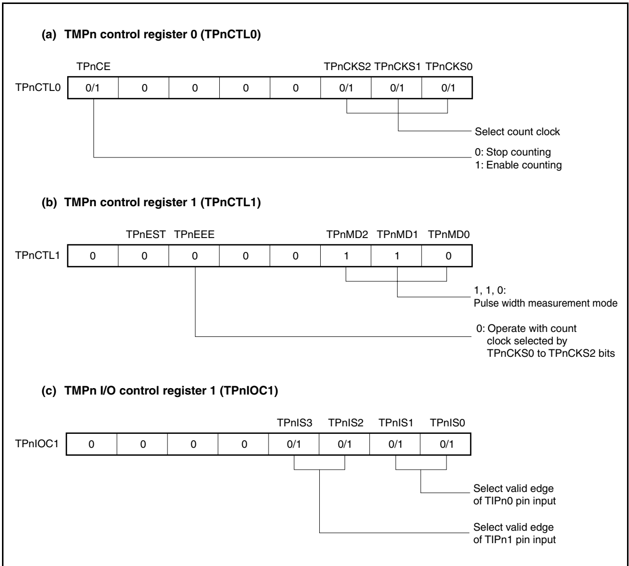
Figure 7-42. Register Setting in Pulse Width Measurement Mode (1/2)
