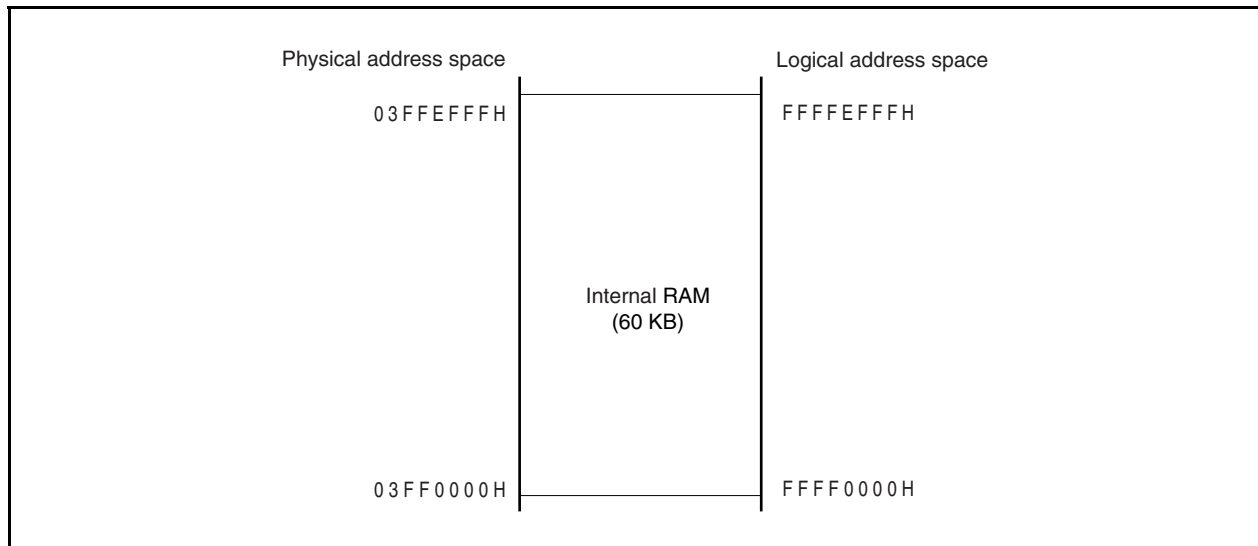
Figure 3-9. Internal RAM Area (60 KB)
