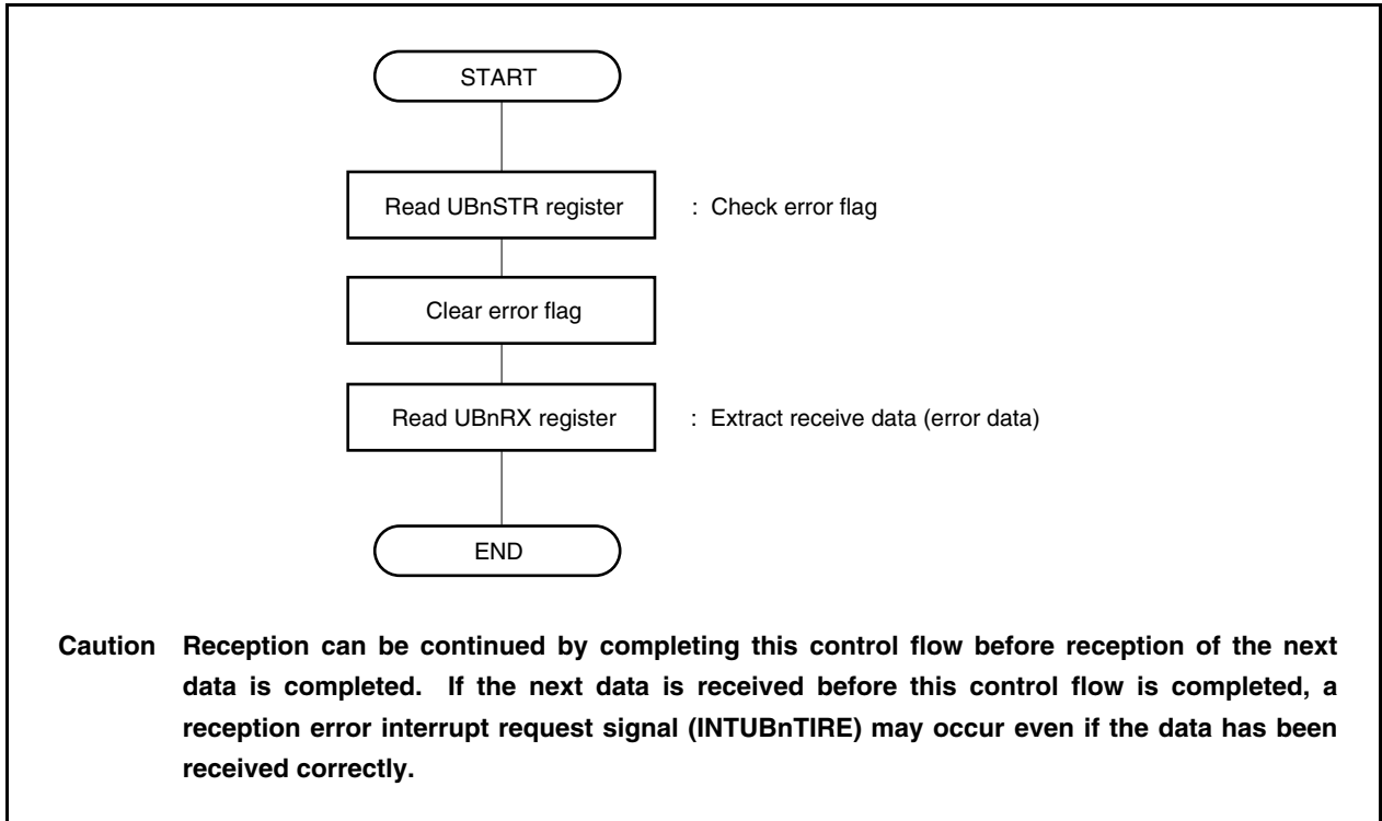
Figure 16-17. Example of Reception Error Processing Flow in Single Mode
