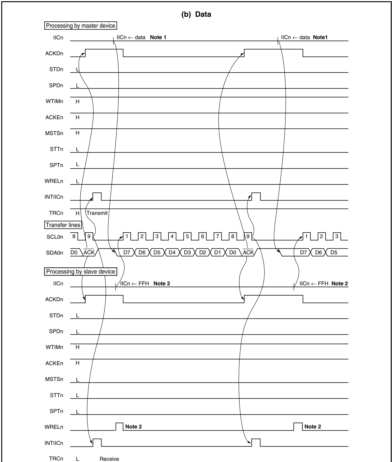
Figure 19-20. Example of Master to Slave Communication (When 9-Clock Wait Is Selected for Both Master and Slave) (2/3)
