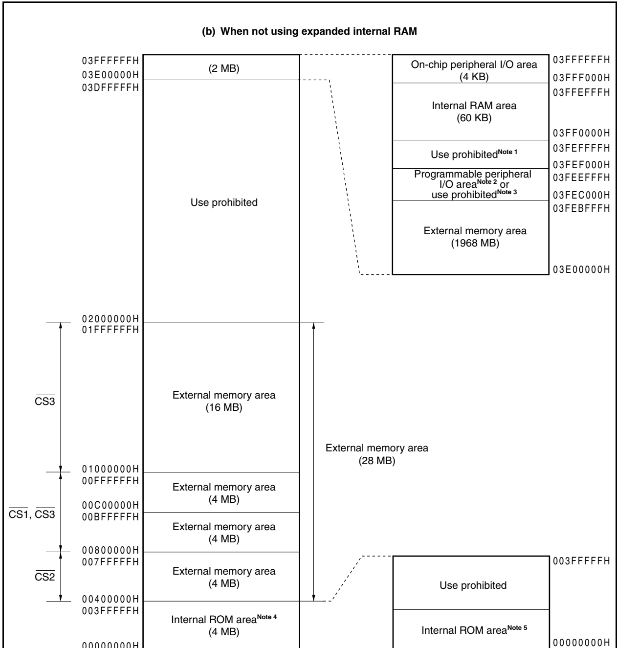
Figure 5-1. Data Memory Map: Physical Address (2/2)
