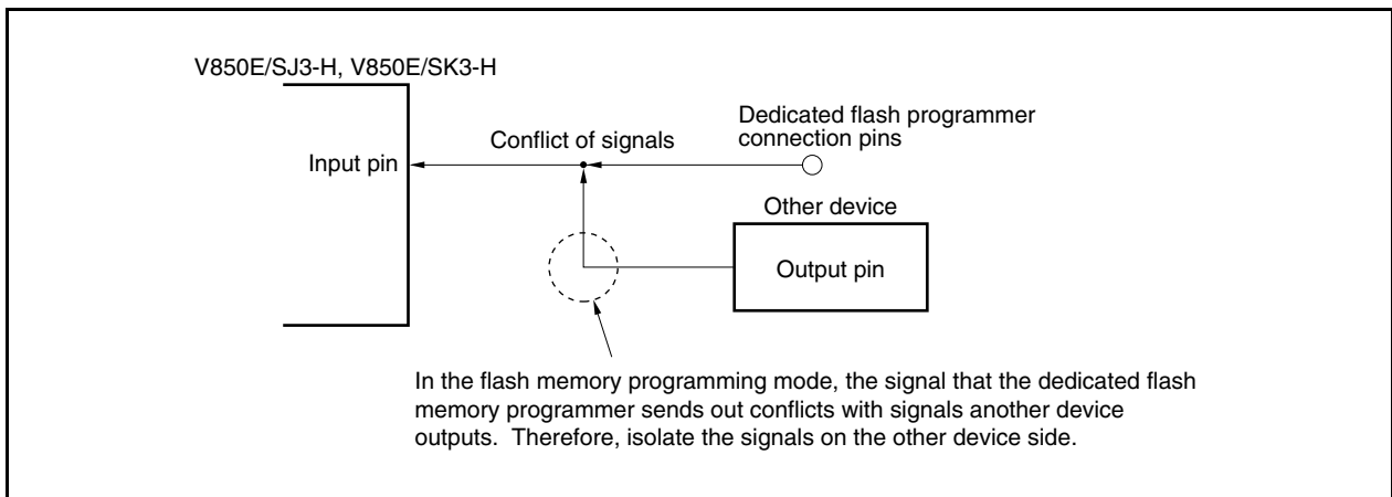
Figure 32-13. Conflict of Signals (Serial Interface Input Pin)
