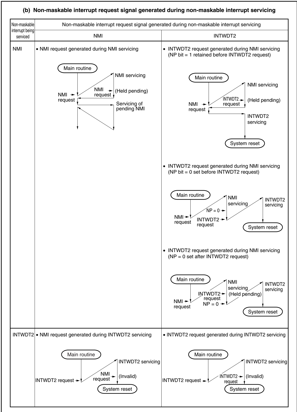
Figure 24-1. Non-Maskable Interrupt Request Signal Acknowledgment Operation (2/2)
