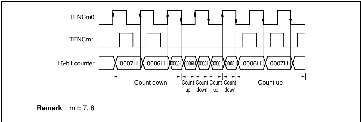
Figure 7-47. Operation Example (Count Operation When Valid Edges of TENCM0 and TENCM1 Pins Overlap)
