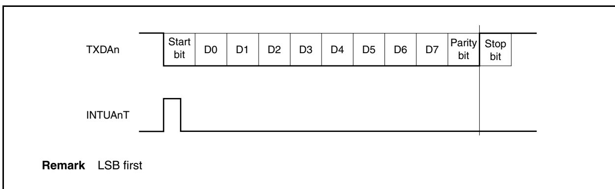
Figure 15-7. UART Transmission
