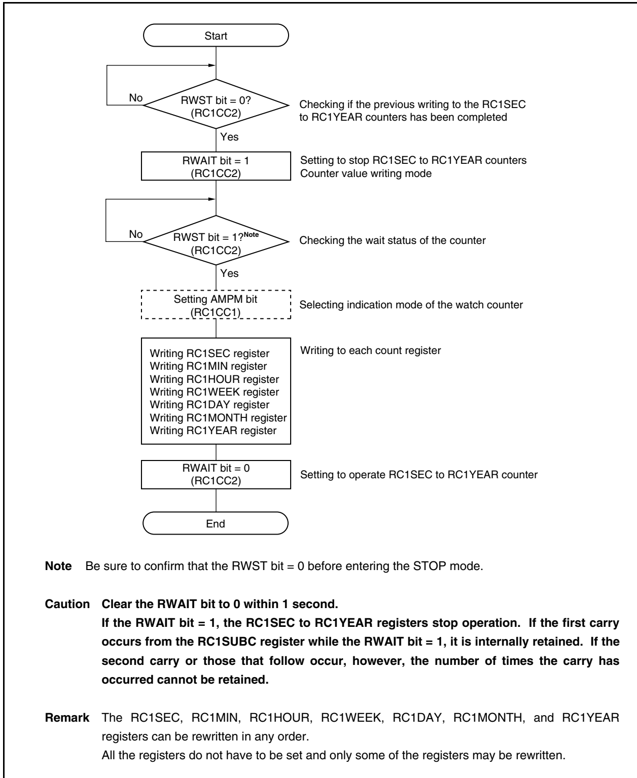
Figure 10-8. Rewriting Each Counter During Clock Operation
