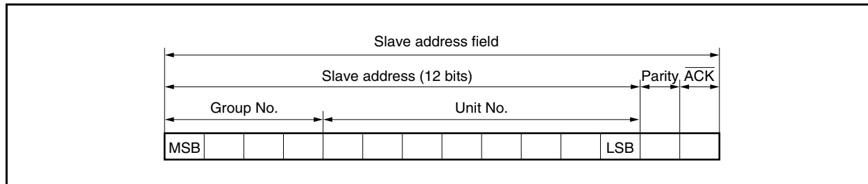
Figure 20-3. Slave Address Field
