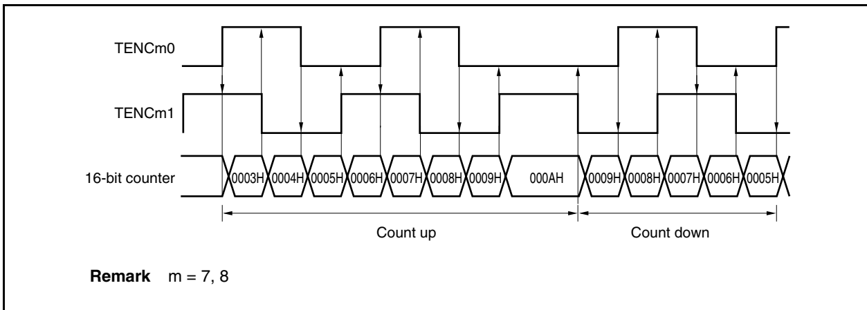
Figure 7-49. Operation Example (Count Operation When Valid Edges of TENCM0 and TENCM1 Pins Overlap)
