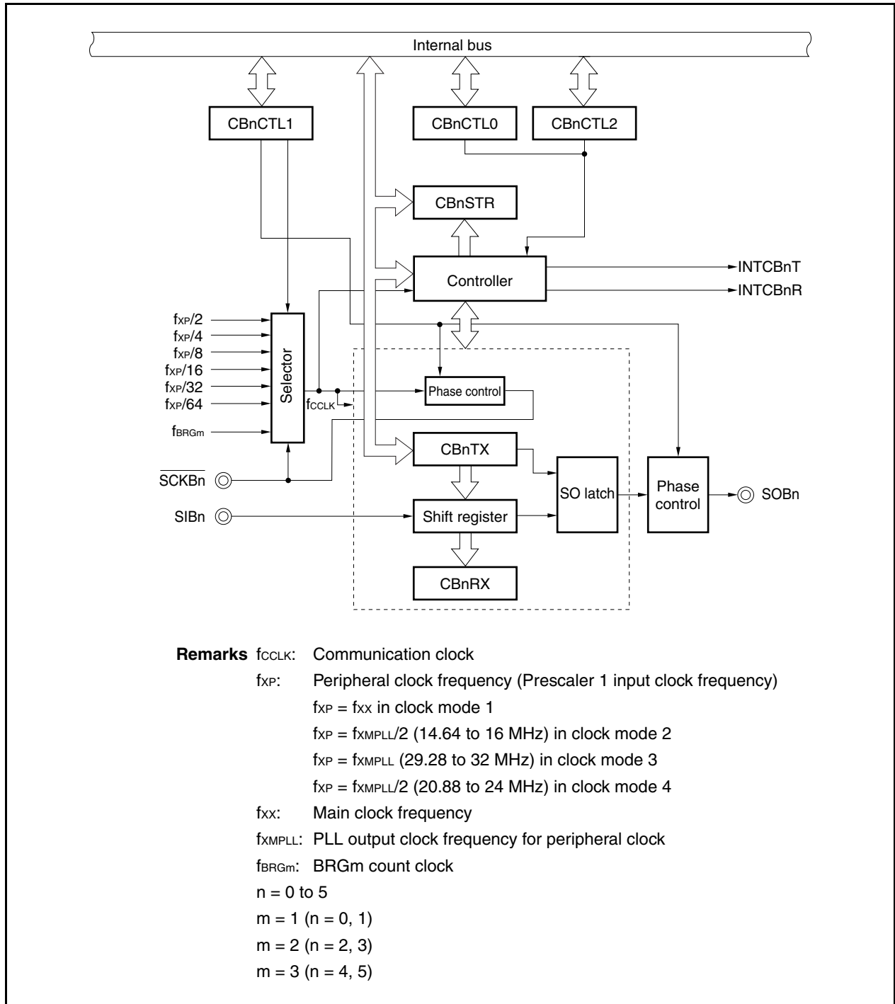
Figure 17-1. Block Diagram of CSIBn
