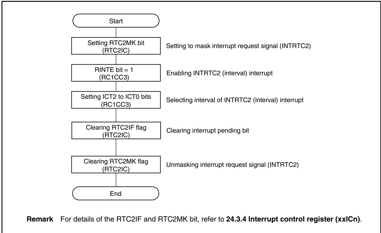
Figure 10-13. Changing Setting of INTRTC2 Interrupt During Clock Operation
