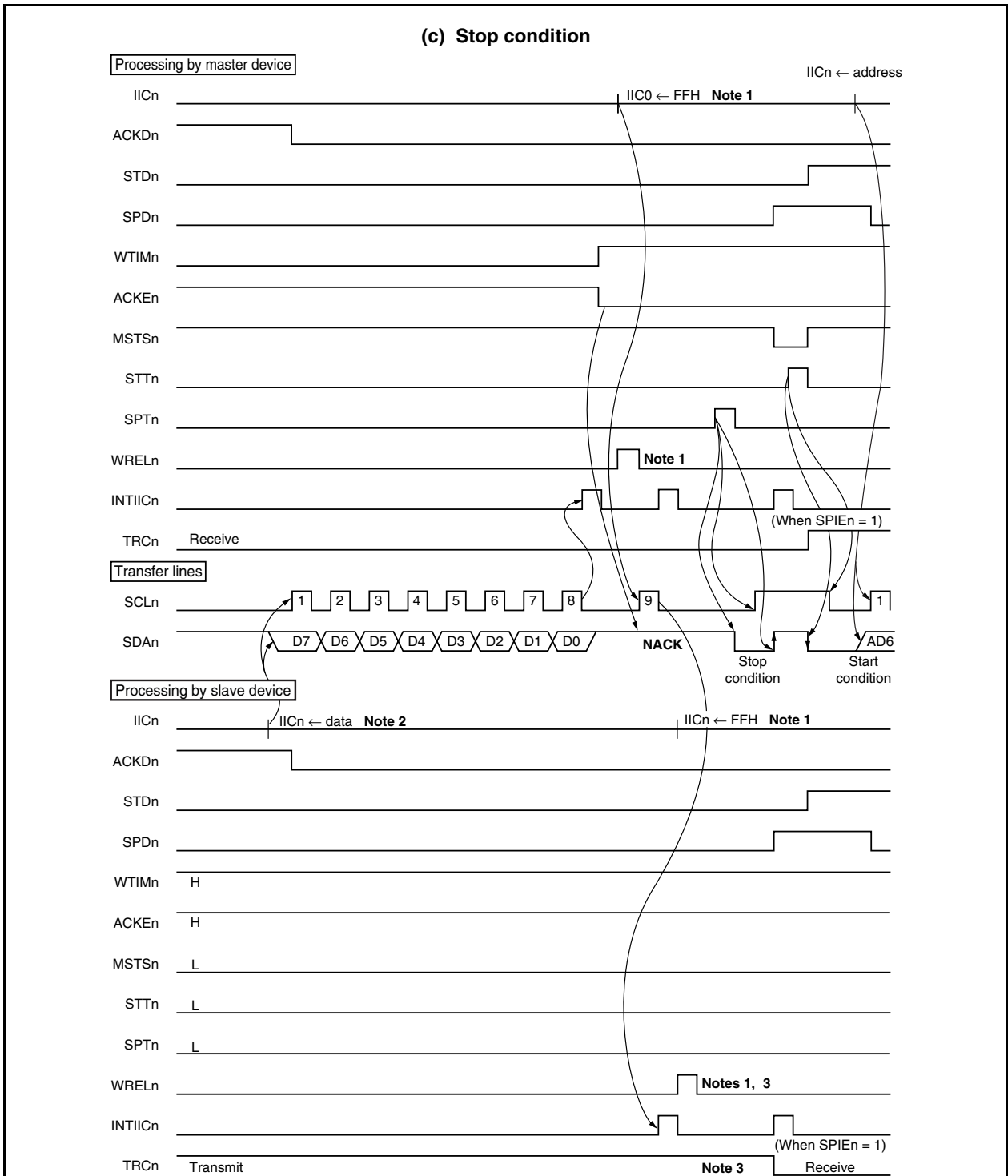
Figure 19-21. Example of Slave to Master Communication (When 8-Clock → 9-Clock Wait for Master and 9-Clock Wait for Slave Are Selected) (3/3)
