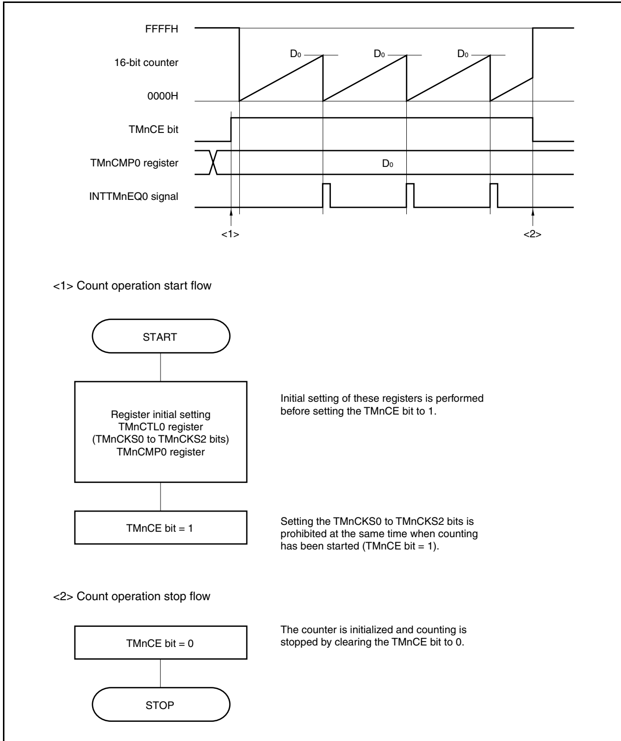
Figure 9-6. Software Processing Flow in Interval Timer Mode
