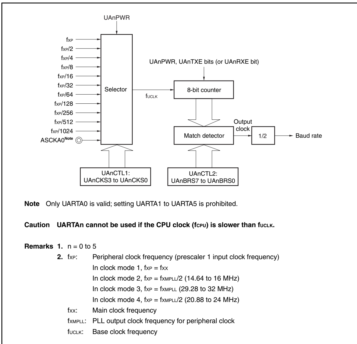
Figure 15-13. Configuration of Baud Rate Generator
