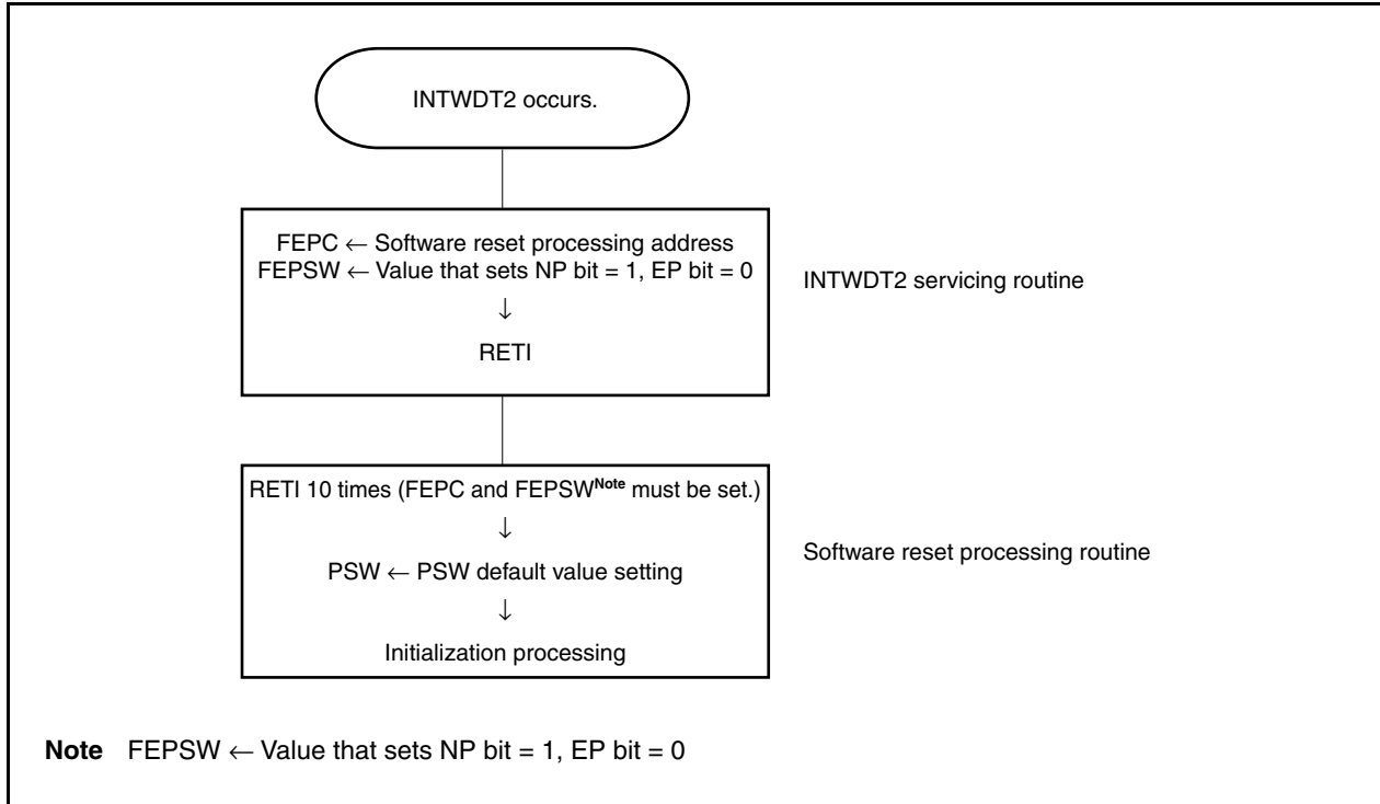
Figure 24-4. Software Reset Processing
