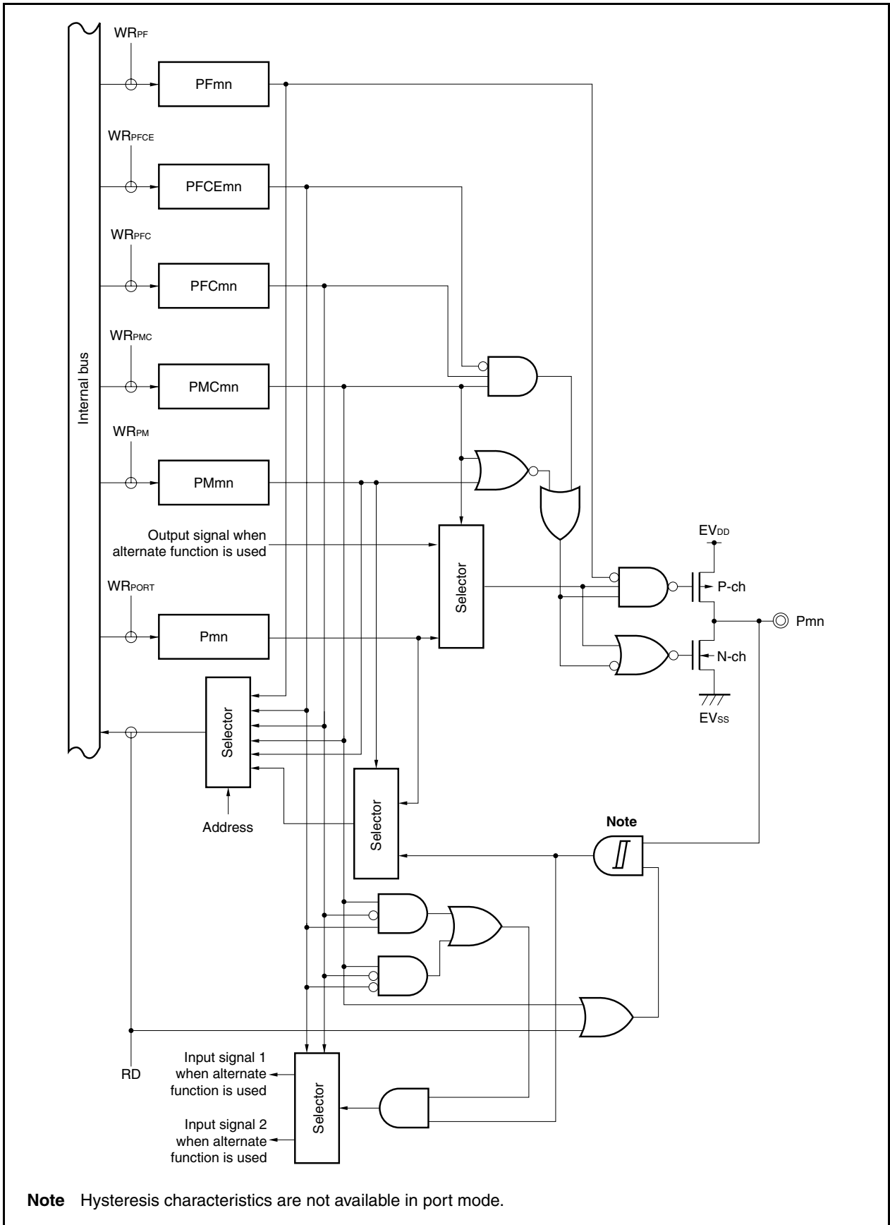
Figure 4-57. Block Diagram of Type U-29
