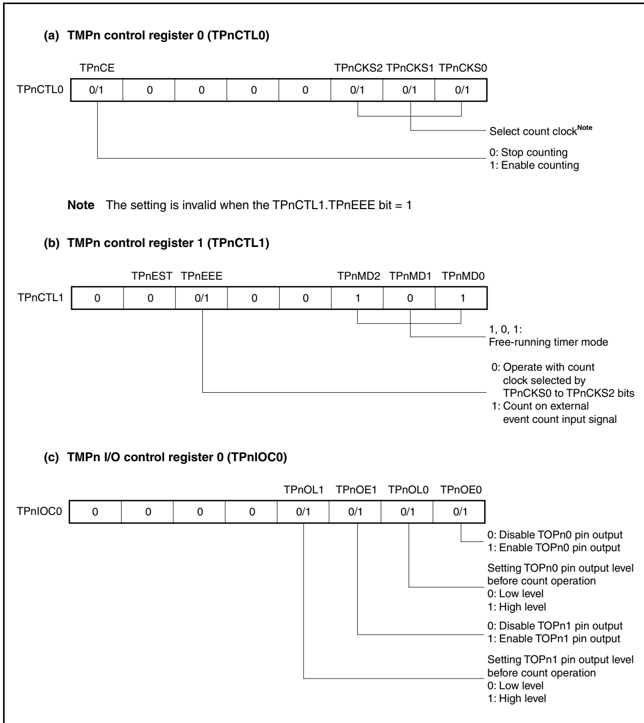
Figure 7-37. Register Setting in Free-Running Timer Mode (1/3)
