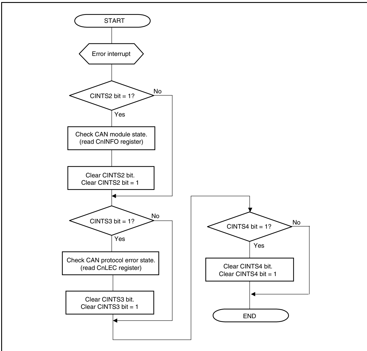
Figure 21-58. Error Handling
