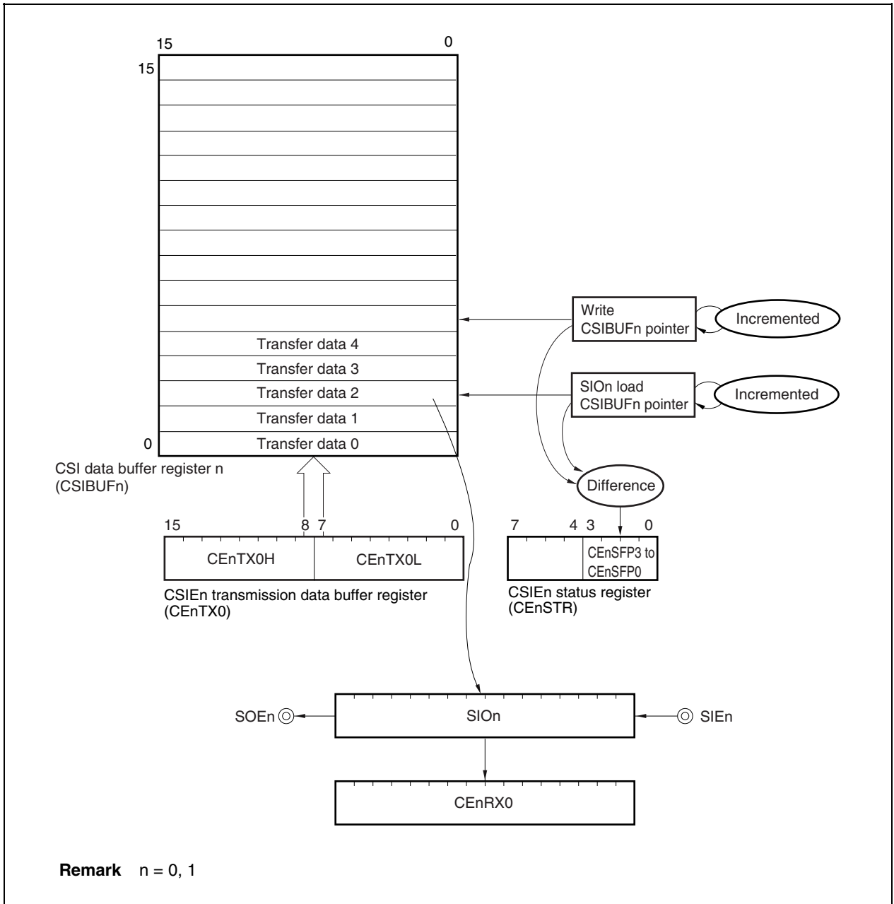
Figure 18-10. Single Mode
