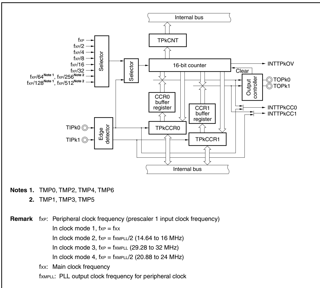
Figure 7-1. Block Diagram of TMPk
