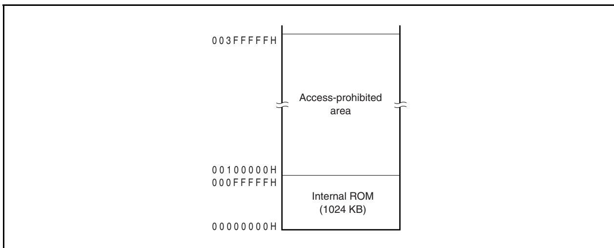
Figure 3-6. Internal ROM Area (1024 KB)
