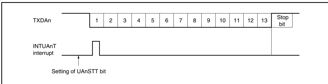
Figure 15-5. SBF Transmission
