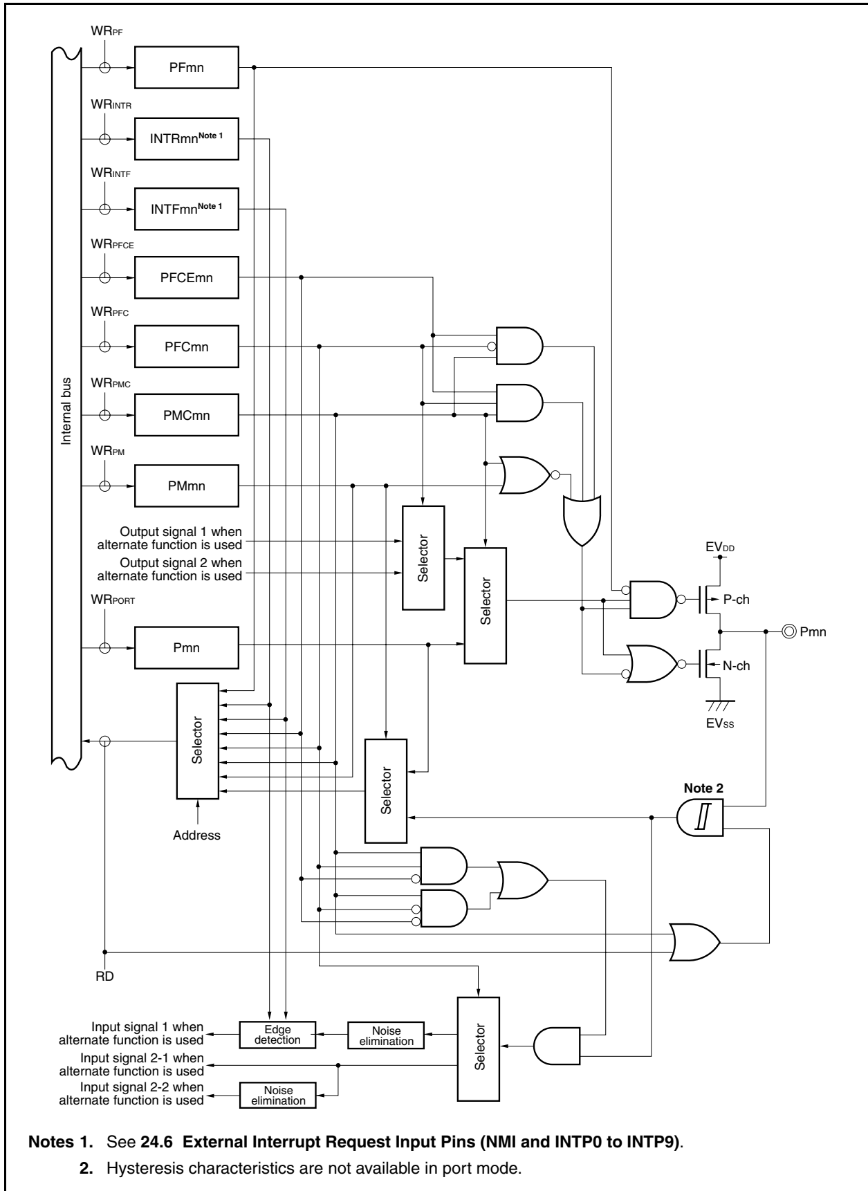
Figure 4-48. Block Diagram of Type U-20
