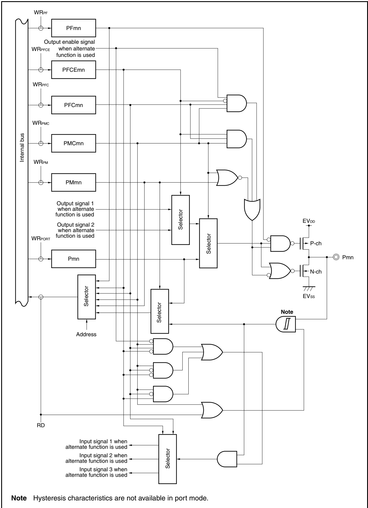
Figure 4-29. Block Diagram of Type U-1
