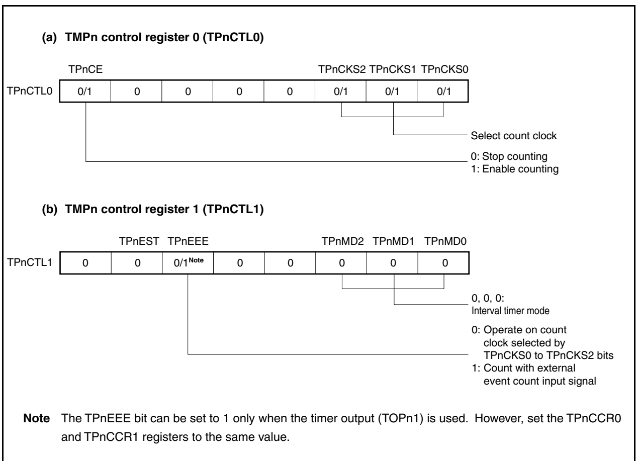
Figure 7-10. Register Setting for Interval Timer Mode Operation (1/3)
