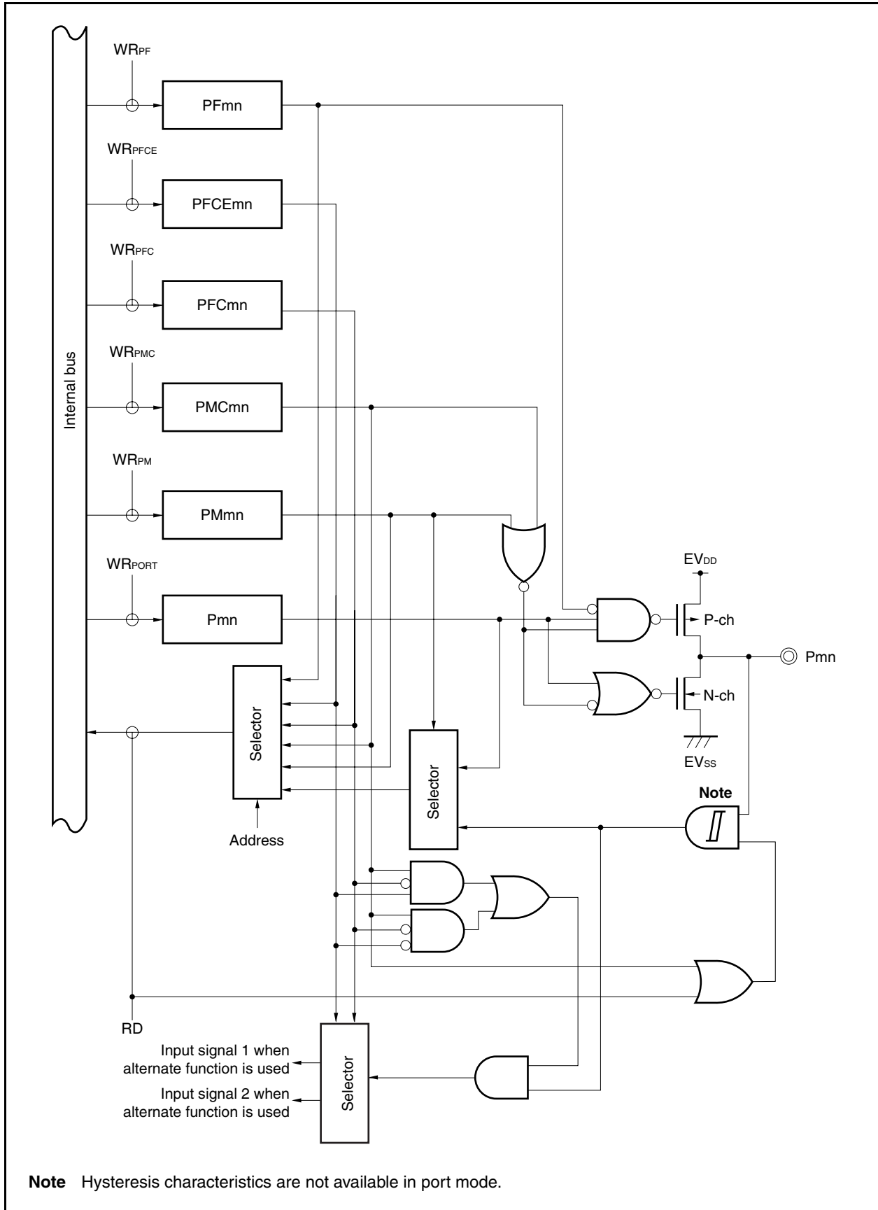
Figure 4-58. Block Diagram of Type U-30
