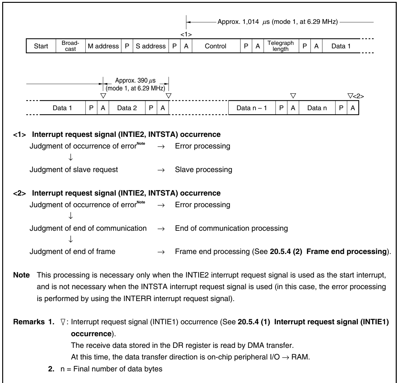
Figure 20-29. Slave Reception
