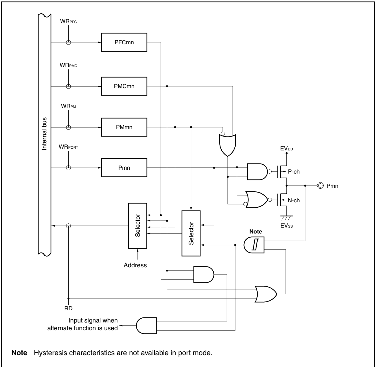
Figure 4-15. Block Diagram of Type F-1
