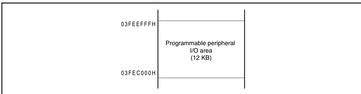
Figure 3-11. Programmable Peripheral I/O Area
