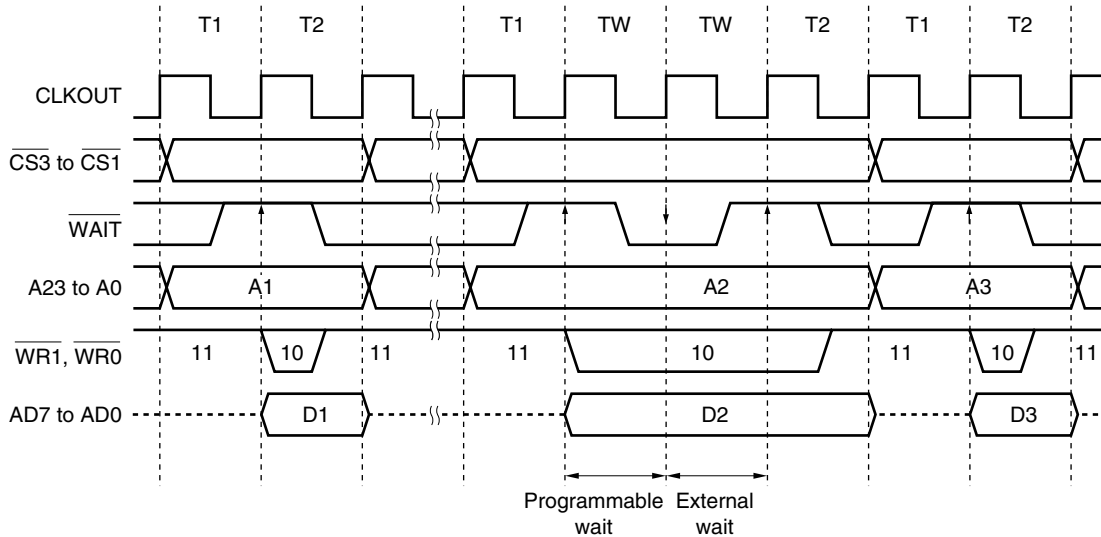
Figure 5-14. Separate Bus Write Timing (Bus Size: 8 Bits)
