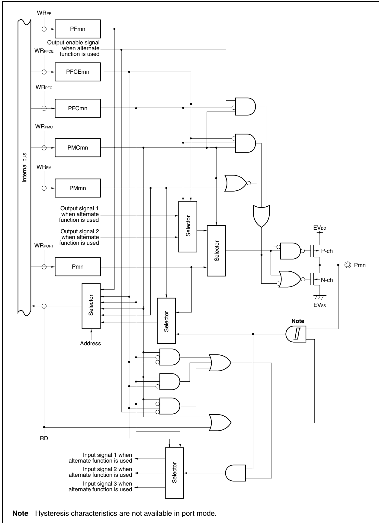
Figure 4-46. Block Diagram of Type U-18
