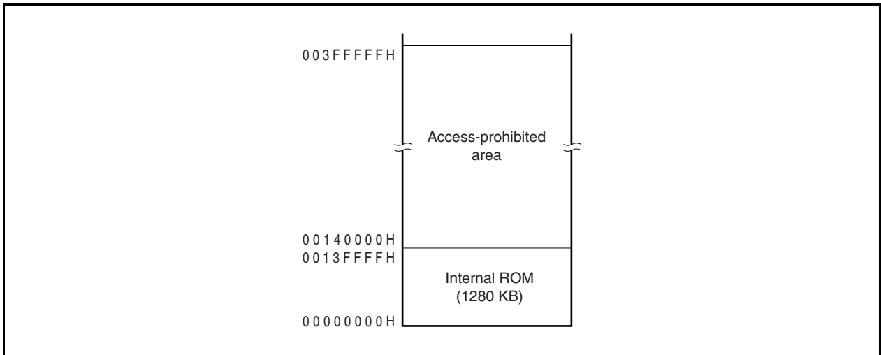
Figure 3-7. Internal ROM Area (1280 KB)
