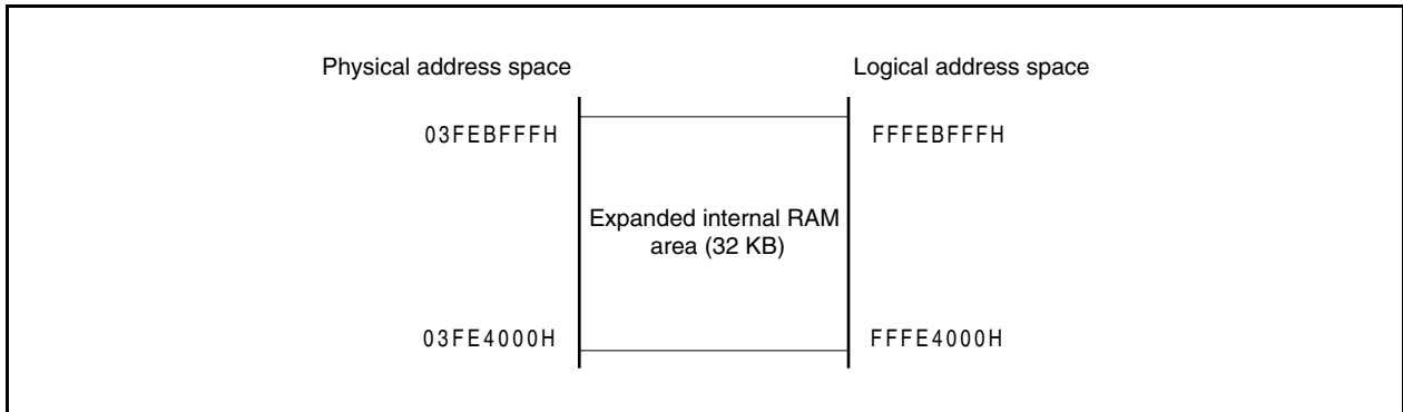
Figure 3-13. Expanded Internal RAM Area (32 KB)
