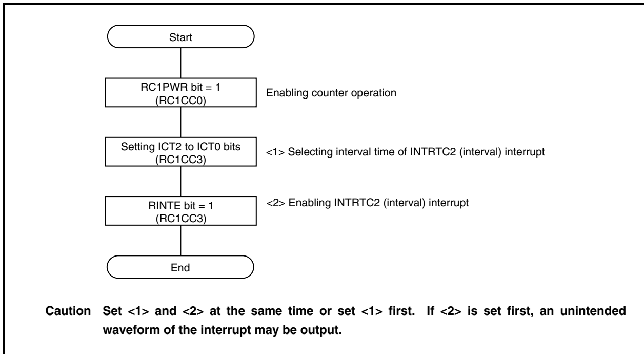
Figure 10-12. Setting of INTRTC2 Interrupt
