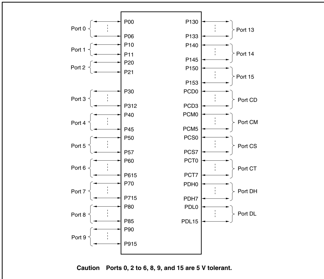
Figure 4-2. Port Configuration Diagram
