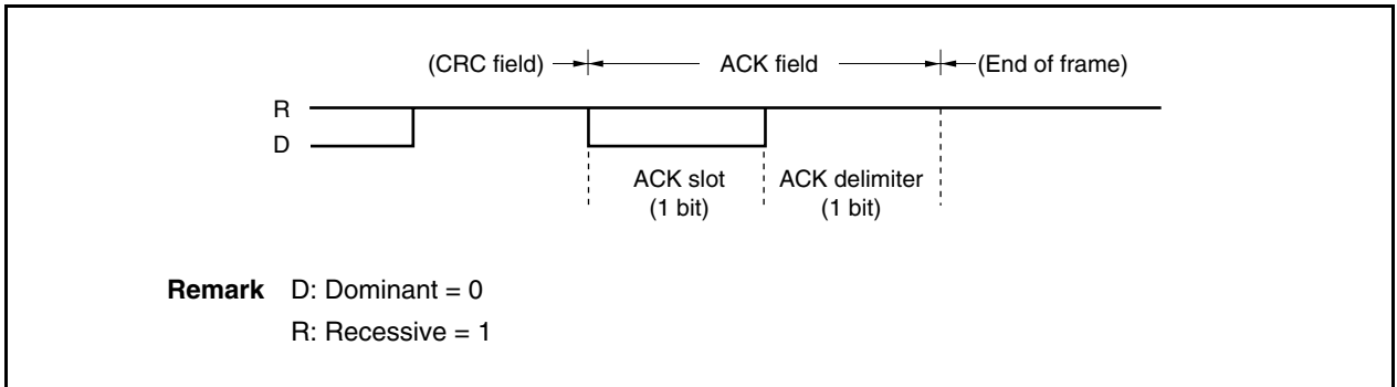
Figure 21-11. ACK Field
