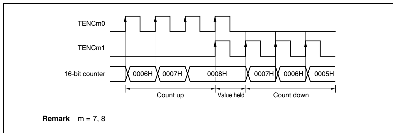
Figure 7-45. Operation Example (When Rising Edge Is Specified as Valid Edge of TENCM0 and TENCM1 Pins)
