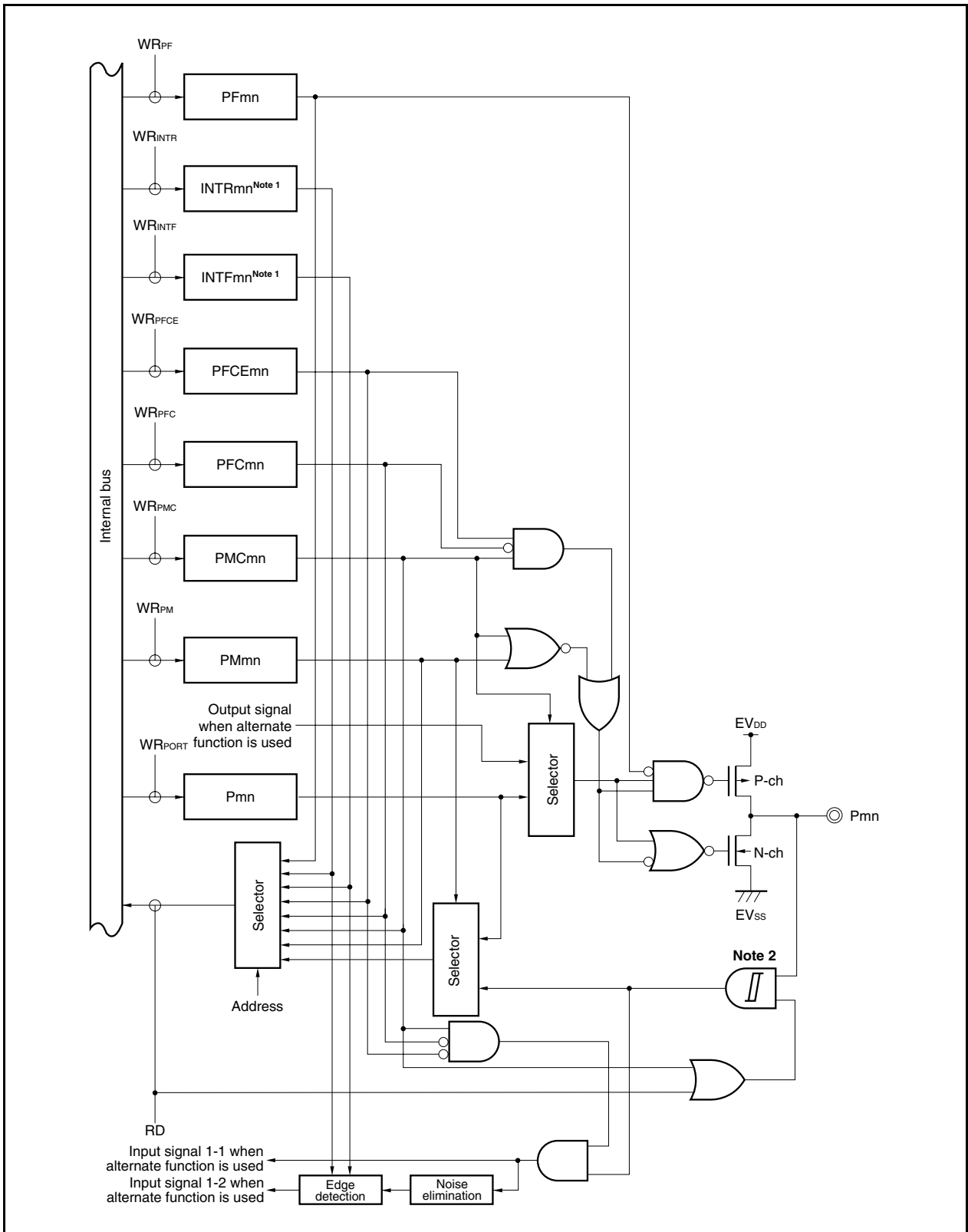
Figure 4-61. Block Diagram of Type U-33
