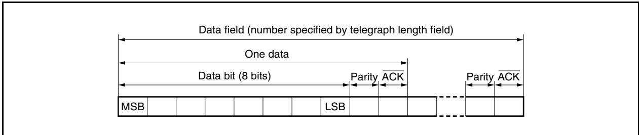
Figure 20-6. Data Field
