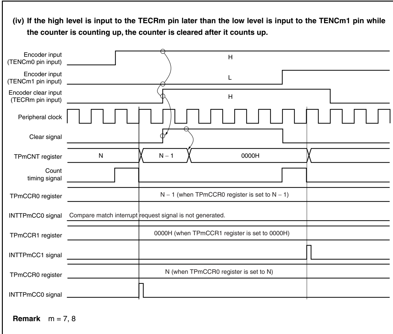
Figure 7-53. Operation Example (When TPmSCE Bit = 1, TPmZCL Bit = 1, TPmBCL Bit = 0, TPmACL Bit = 1, TPmUDS1 and TPmUDS0 Bits = 11, TECRm = High Level, TENCm1 = Low Level, and TENCm0 = High Level) (3/3)
