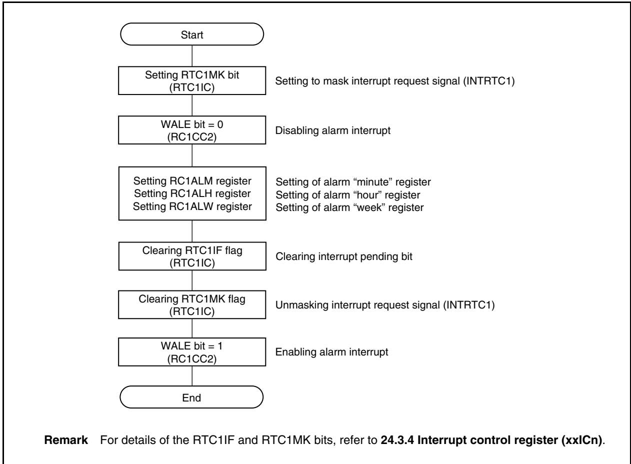
Figure 10-11. Changing Setting of INTRTC1 Interrupt During Clock Operation
