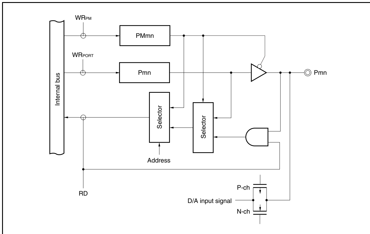
Figure 4-6. Block Diagram of Type B-1
