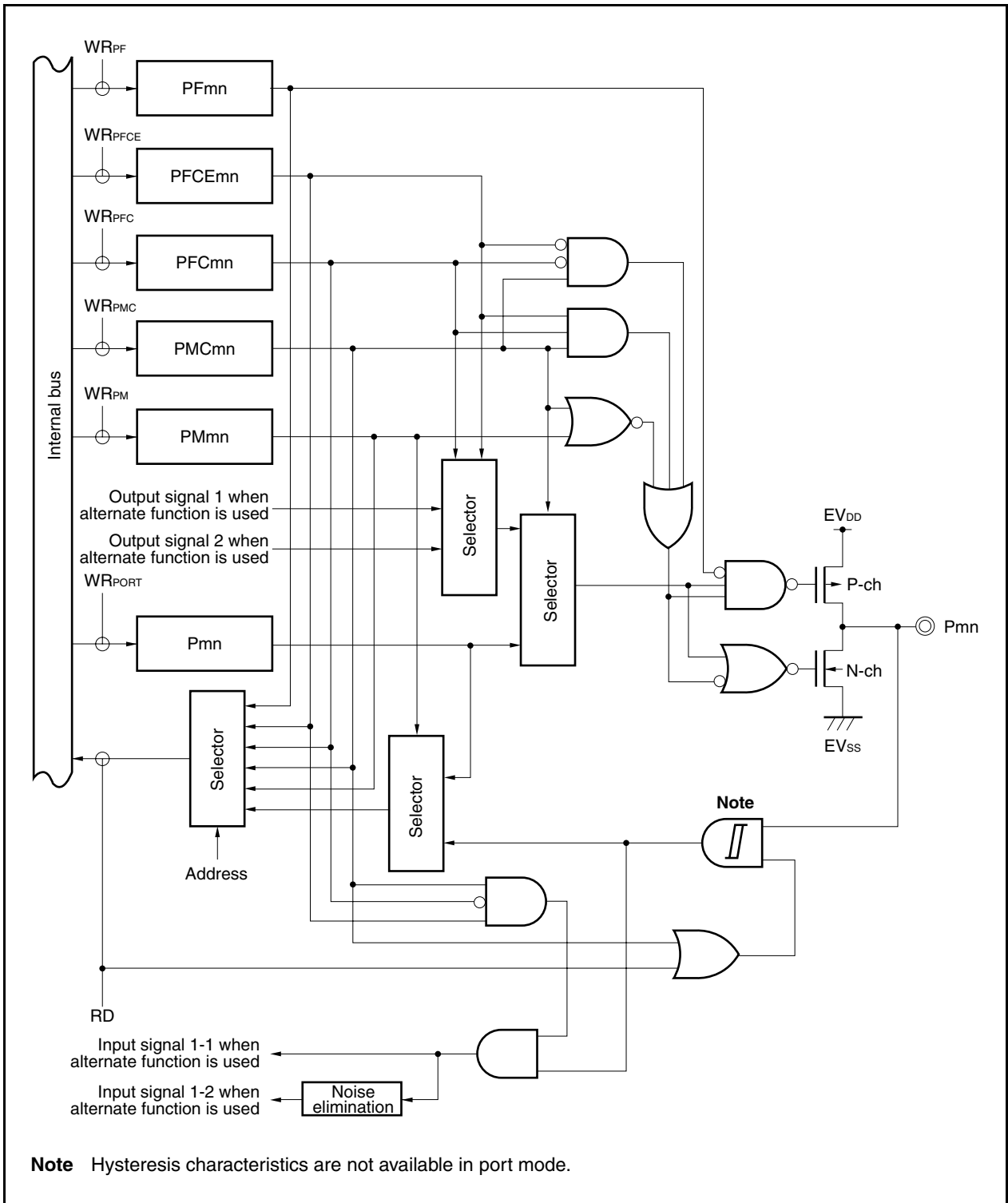
Figure 4-65. Block Diagram of Type U-37
