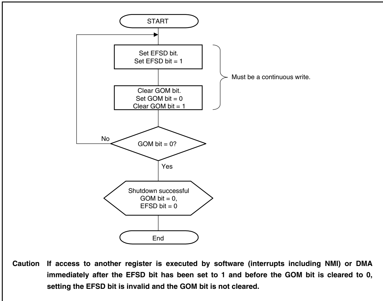
Figure 21-57. Forced Shutdown Process
