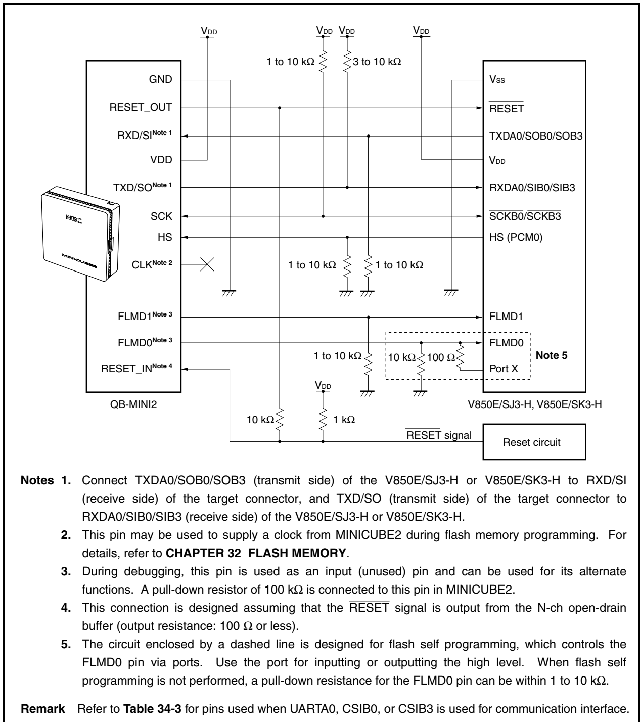
Figure 34-3. Circuit Connection Example When UARTA0/CSIB0/CSIB3 Is Used for Communication Interface
