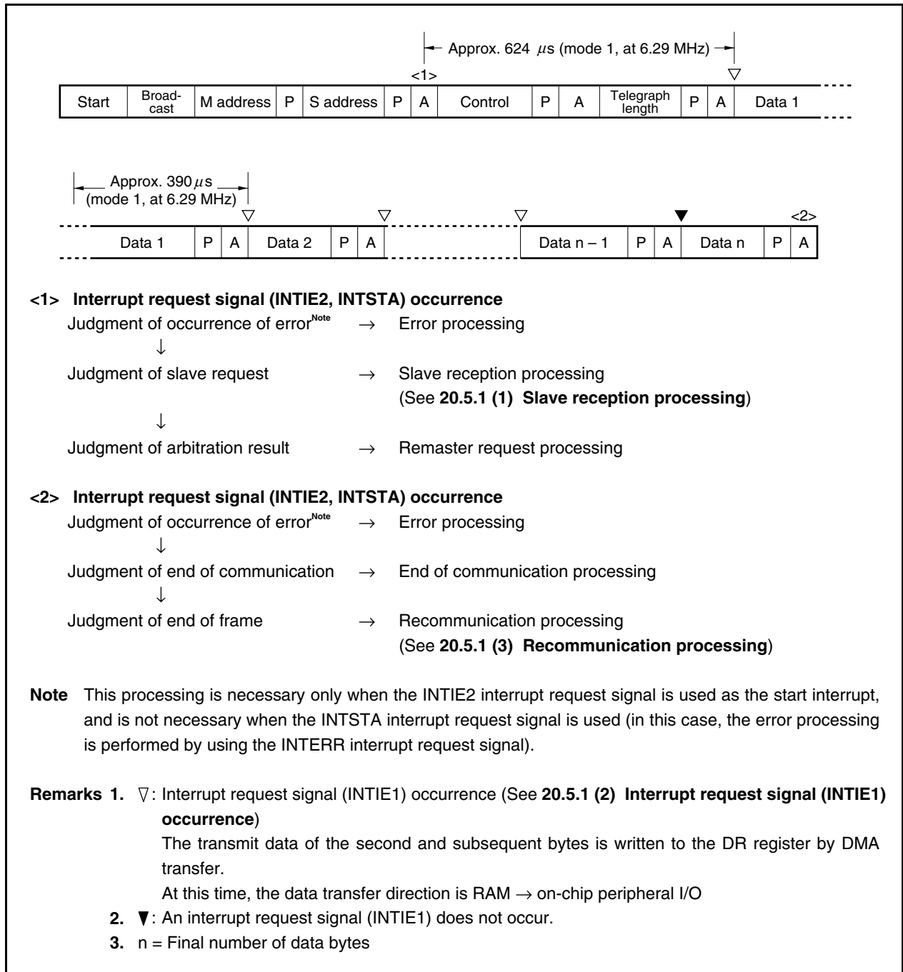
Figure 20-26. Master Transmission
