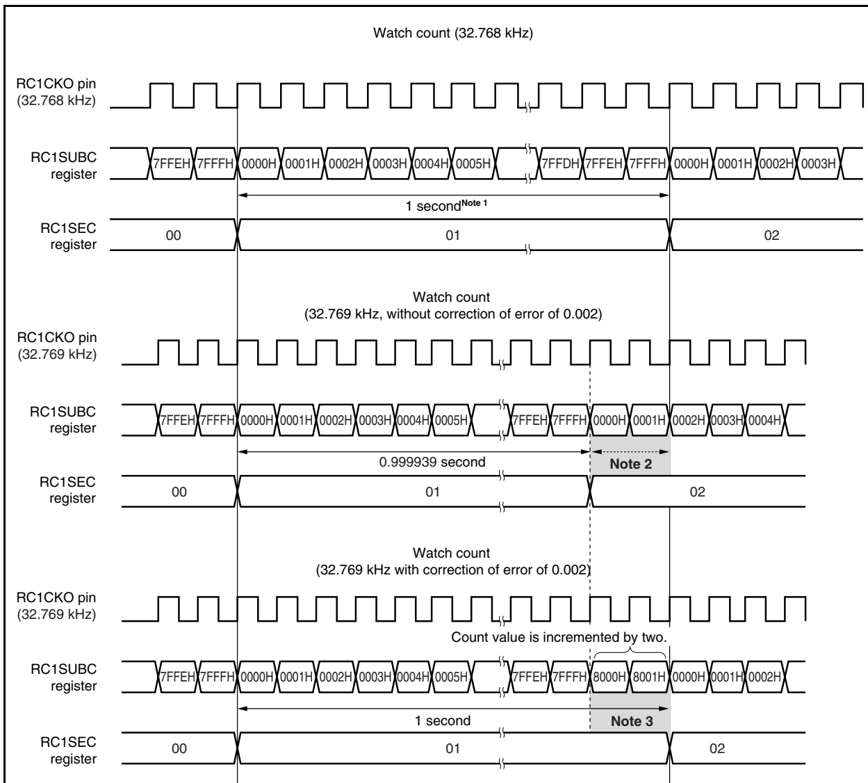
Figure 10-15. Example of Watch Error Correction
