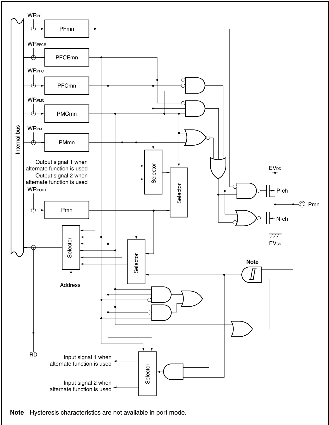
Figure 4-45. Block Diagram of Type U-17
