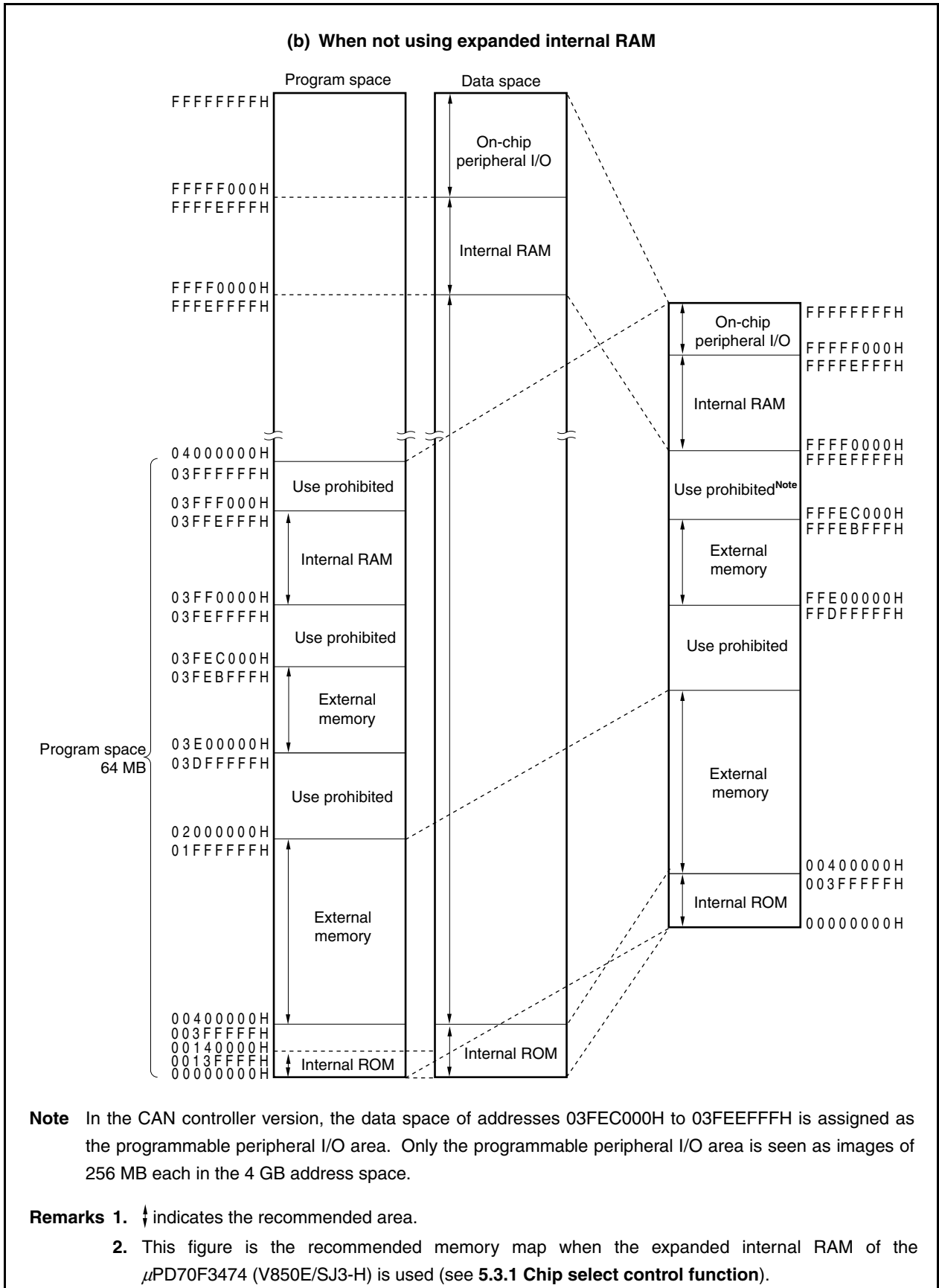
Figure 3-14. Recommended Memory Map (2/2)
