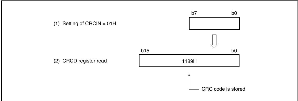
Figure 23-2. CRC Operation Circuit Operation Example (LSB First)
