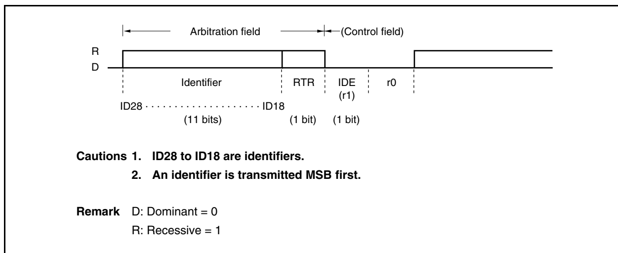
Figure 21-7. Arbitration Field (in Extended Format Mode)
