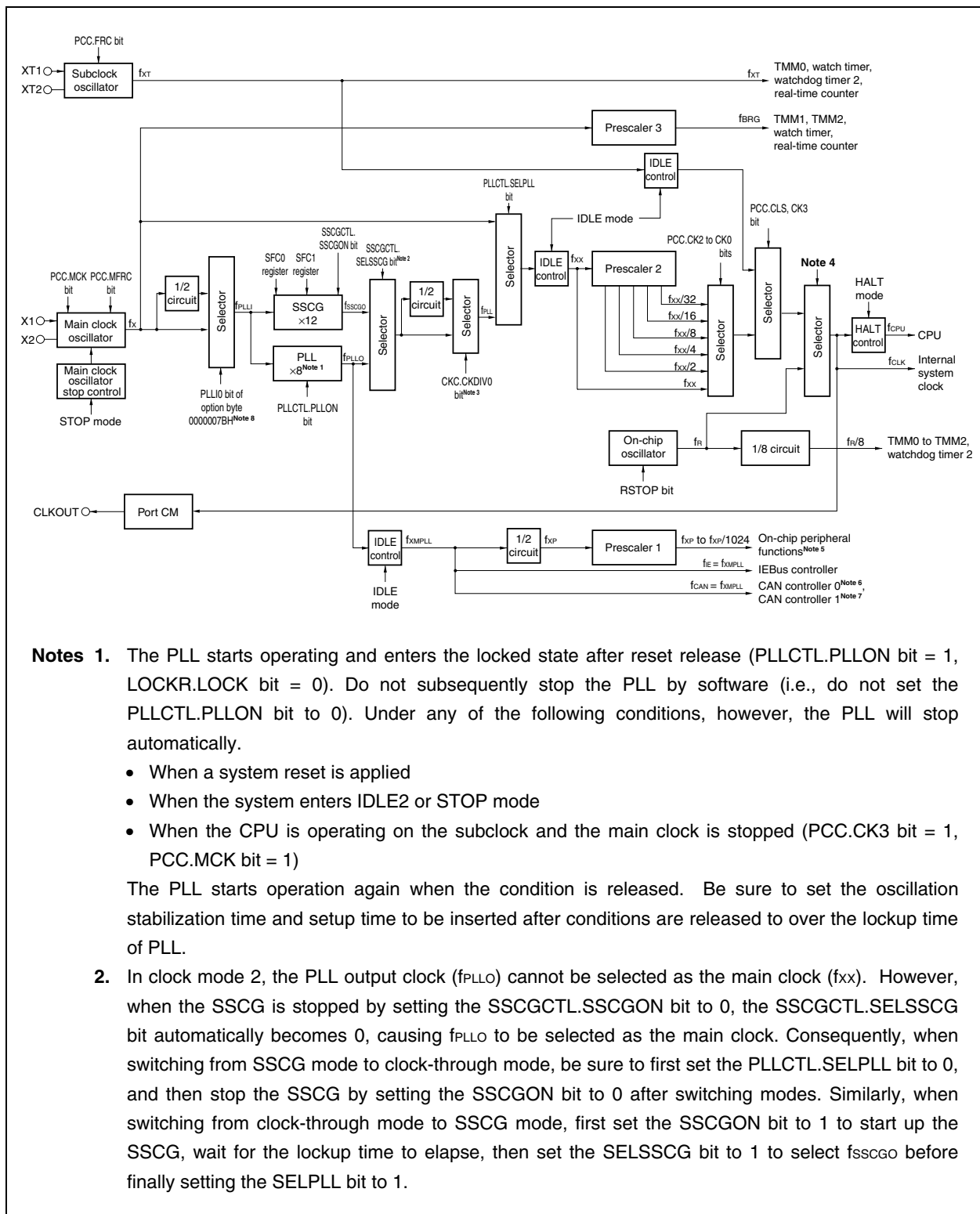
Figure 6-2. Clock Generation Circuit for Clock Mode 2 (1/2)
