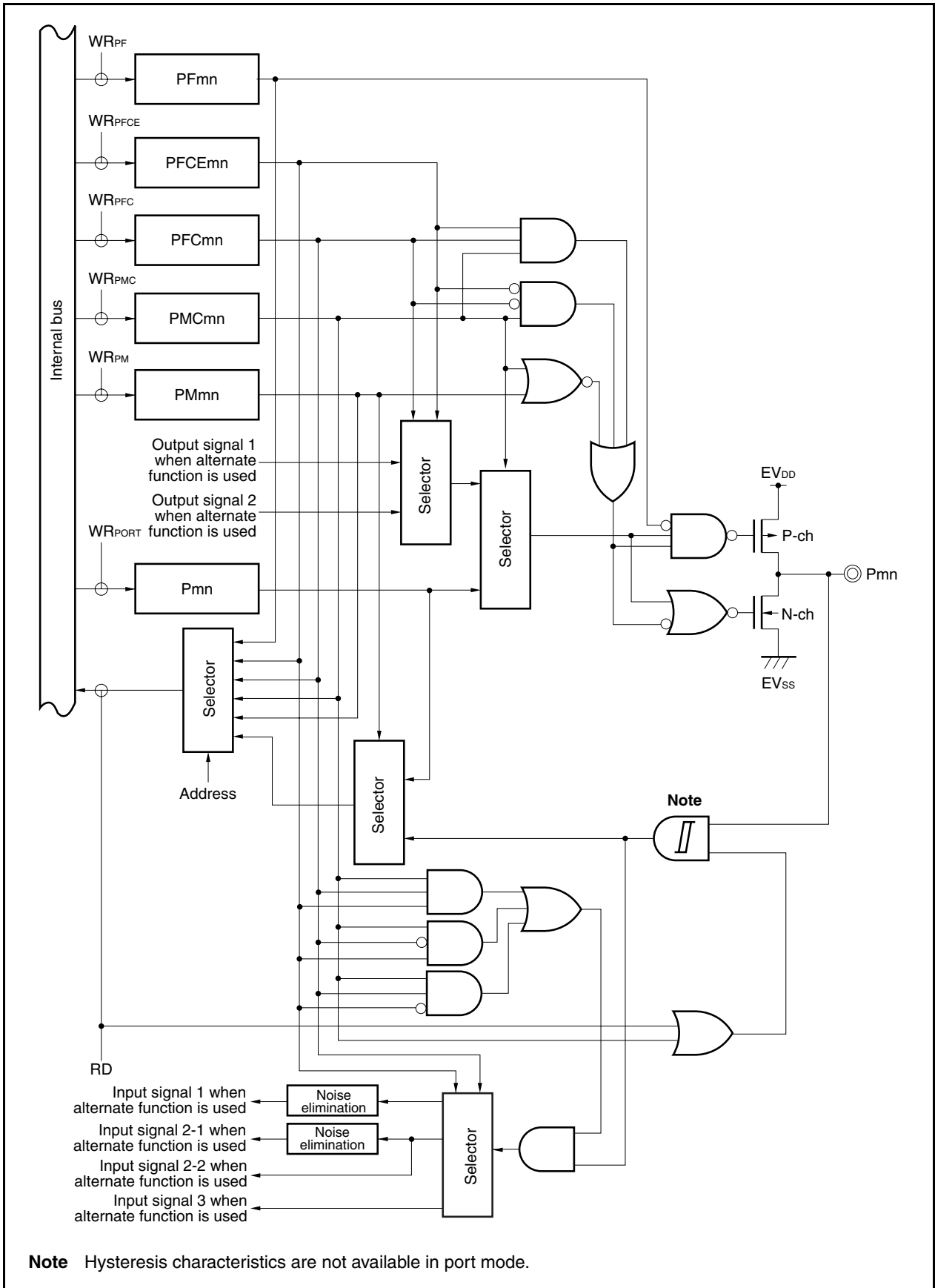
Figure 4-39. Block Diagram of Type U-11
