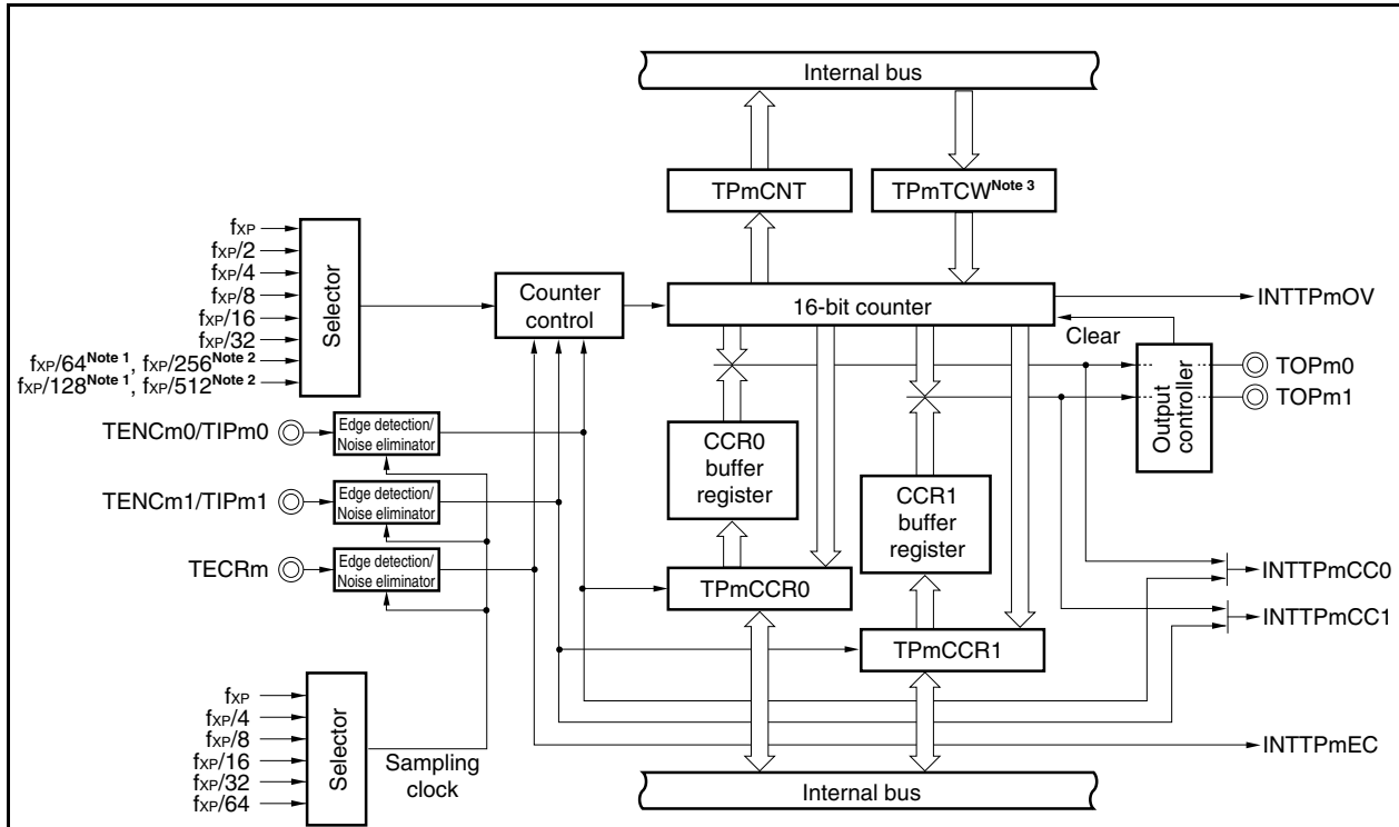
Figure 7-2. Block Diagram of TMP7 and TMP8
