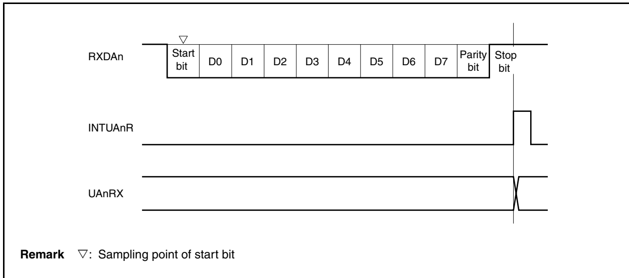
Figure 15-10. UART Reception
