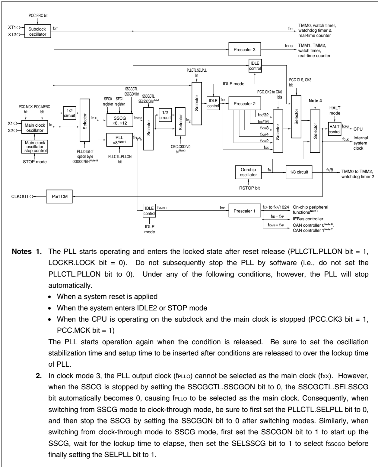
Figure 6-3. Clock Generation Circuit for Clock Mode 3 (1/2)
