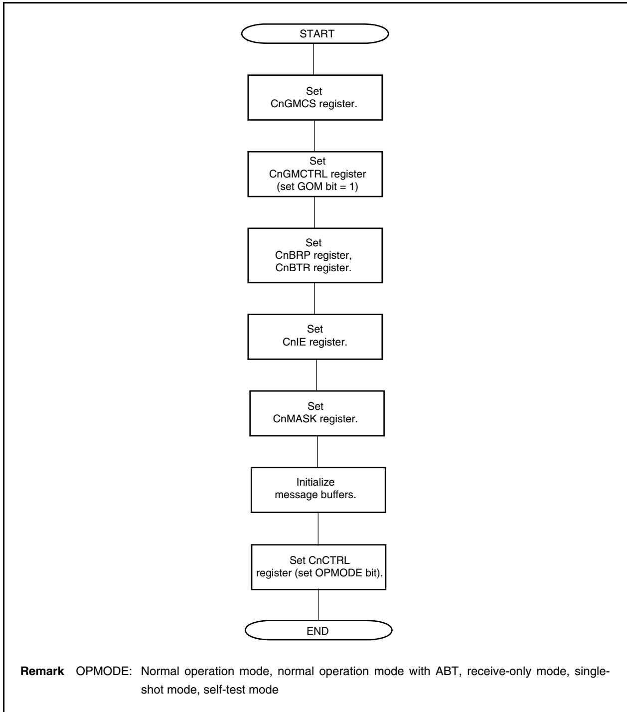
Figure 21-36. Initialization
