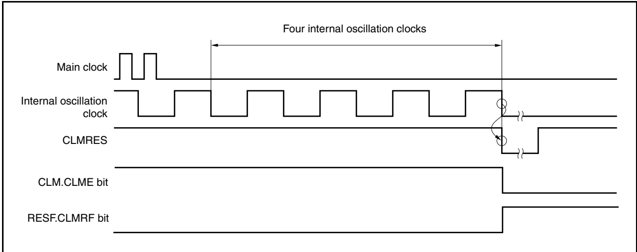
Figure 28-2. Reset Period Due to That Oscillation of Main Clock Is Stopped
