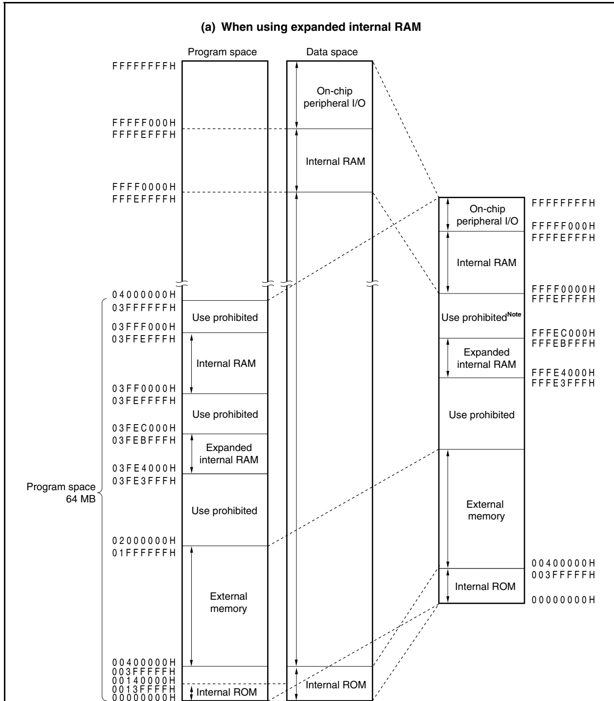
Figure 3-14. Recommended Memory Map (1/2)
