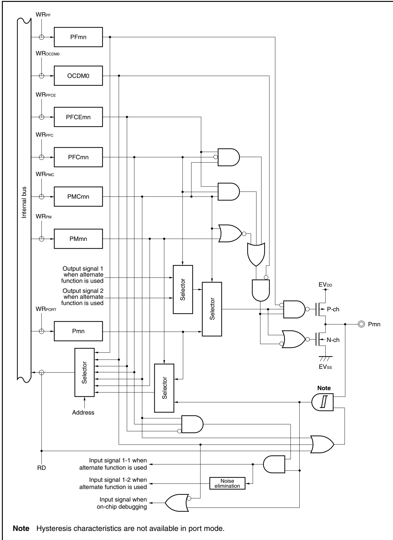
Figure 4-34. Block Diagram of Type U-6
