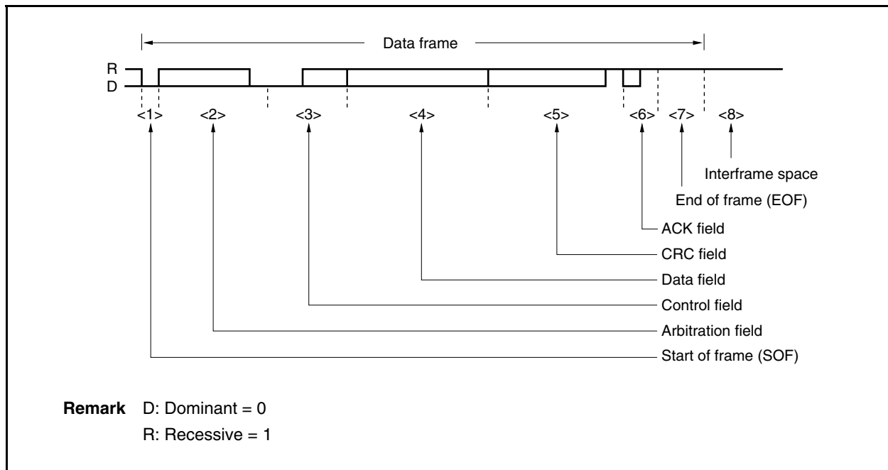
Figure 21-3. Data Frame
