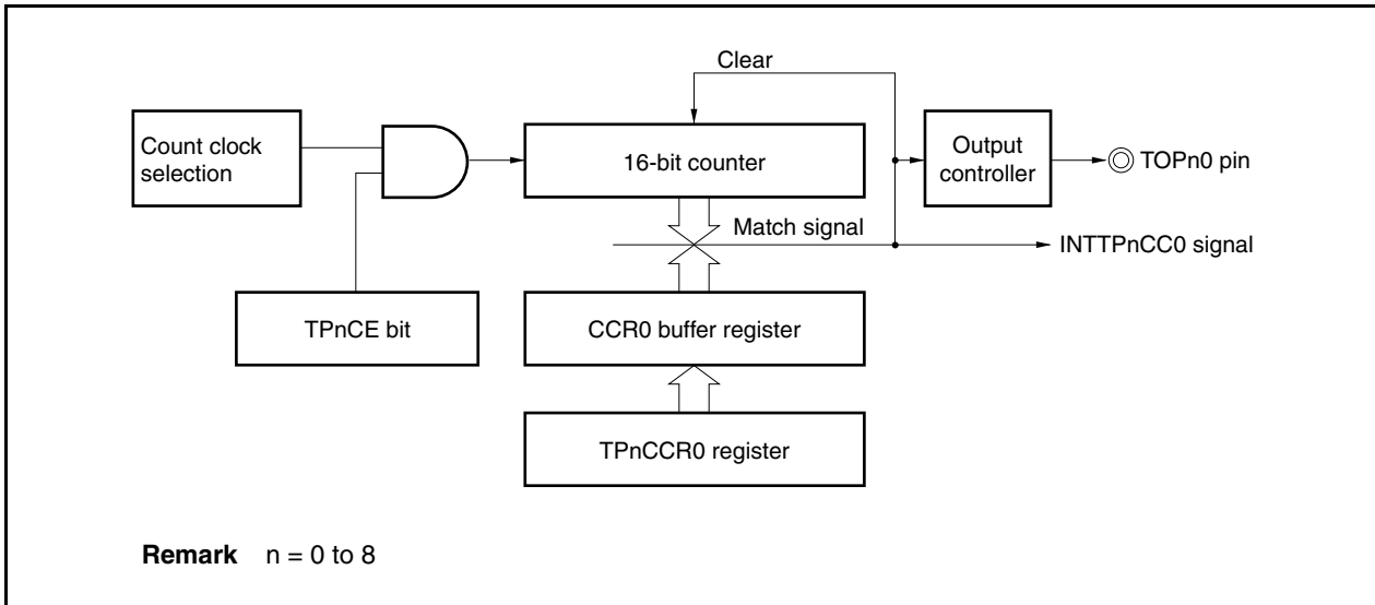
Figure 7-8. Configuration of Interval Timer
