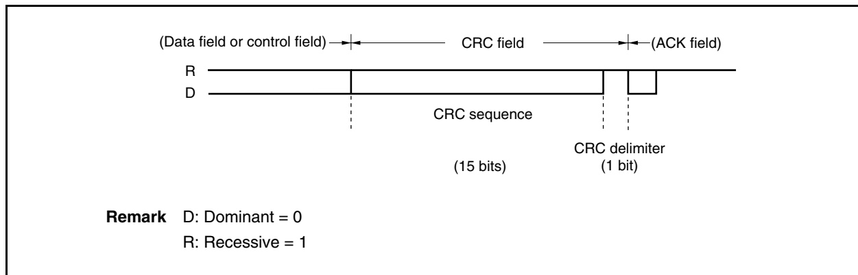
Figure 21-10. CRC Field
