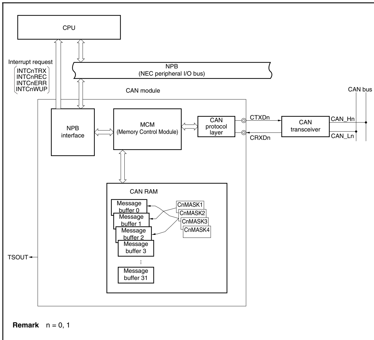
Figure 21-1. Block Diagram of CAN Module
