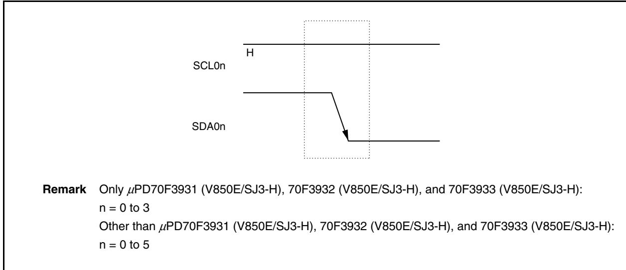
Figure 19-5. Start Condition
