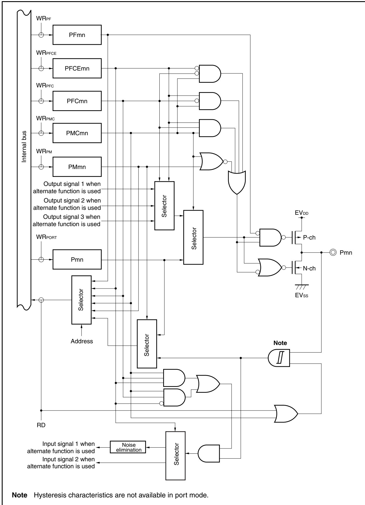
Figure 4-38. Block Diagram of Type U-10
