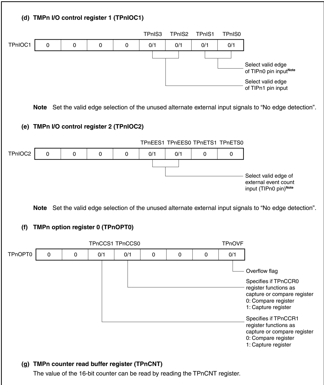
Figure 7-37. Register Setting in Free-Running Timer Mode (2/3)
