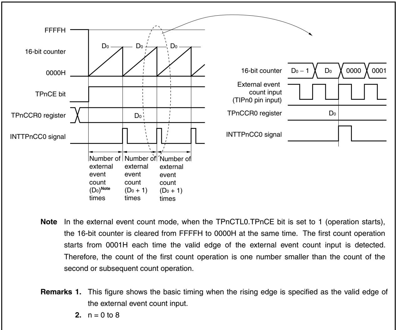
Figure 7-16. Basic Timing in External Event Count Mode
