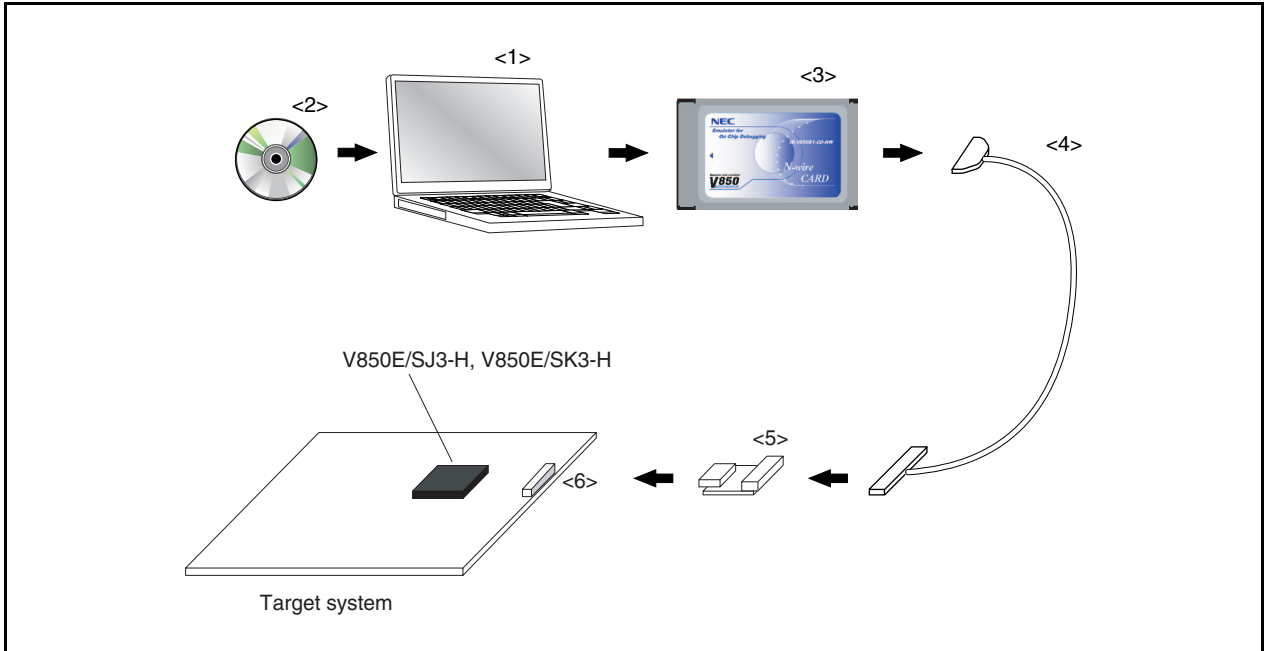
Figure A-3. System Configuration (IE-V850E1-CD-NW Used)
