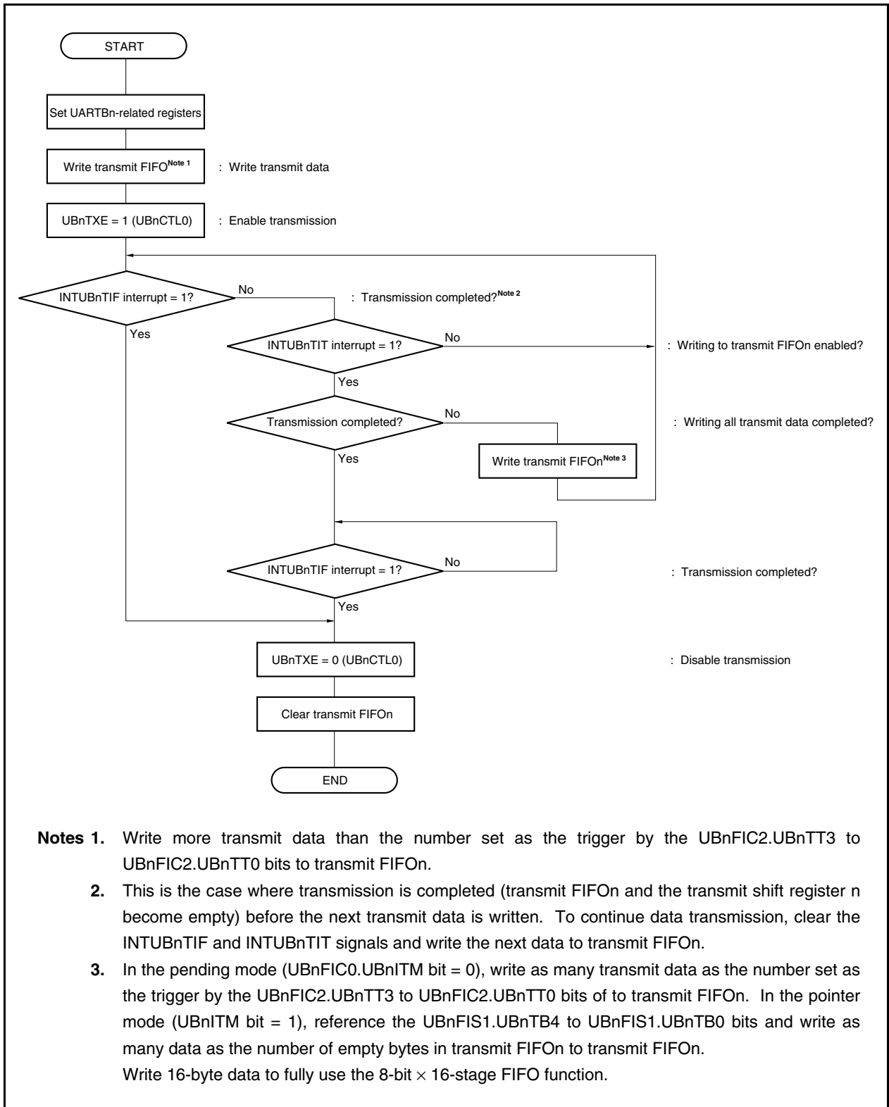
Figure 16-15. Example of Continuous Transmission Processing Flow in FIFO Mode (CPU Control)
