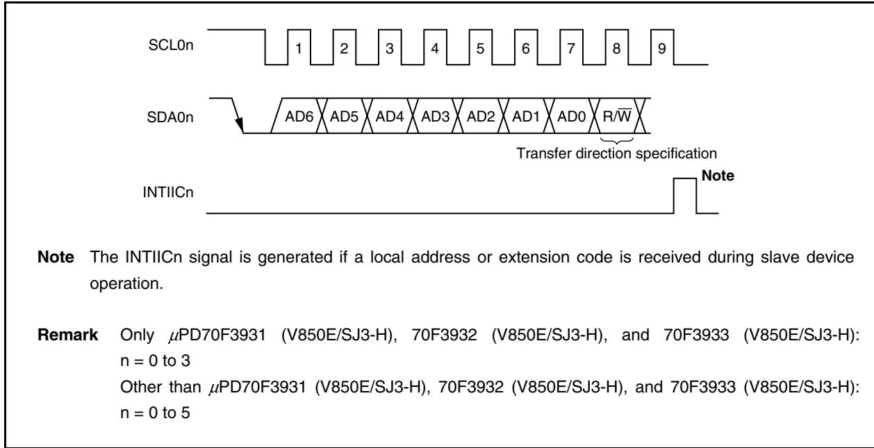
Figure 19-7. Transfer Direction Specification
