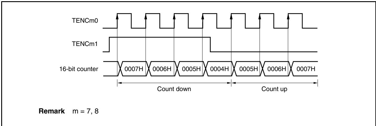
Figure 7-44. Operation Example (When Valid Edge of TENCm0 Pin Is Specified to Be Rising Edge and No Edge Is Specified as Valid Edge of TENCm1 Pin)
