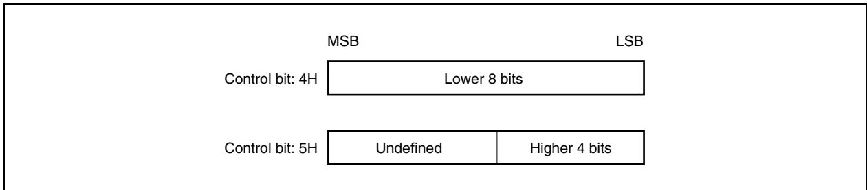
Figure 20-8. Configuration of Lock Address
