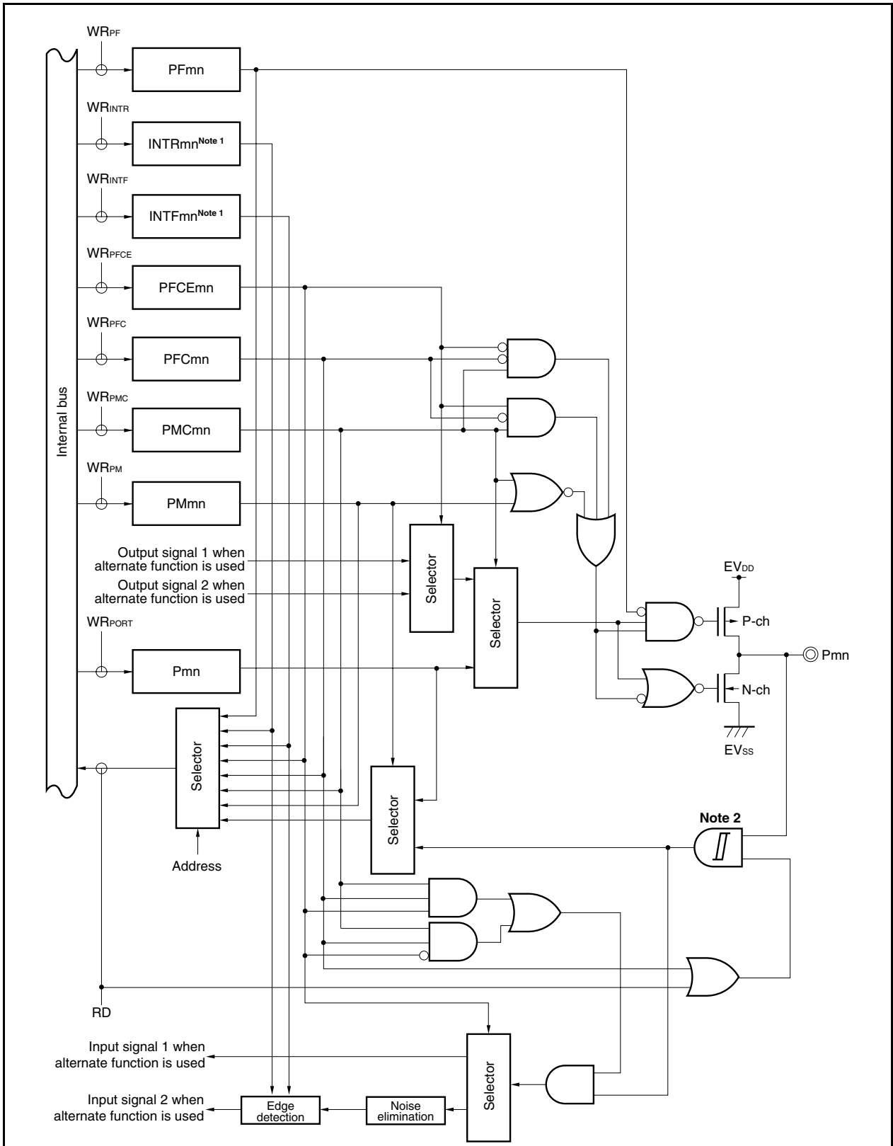
Figure 4-63. Block Diagram of Type U-35
