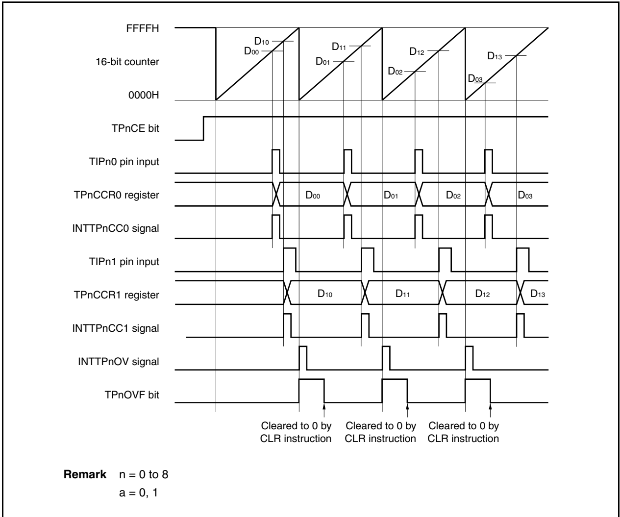
Figure 7-36. Basic Timing in Free-Running Timer Mode (Capture Function)
