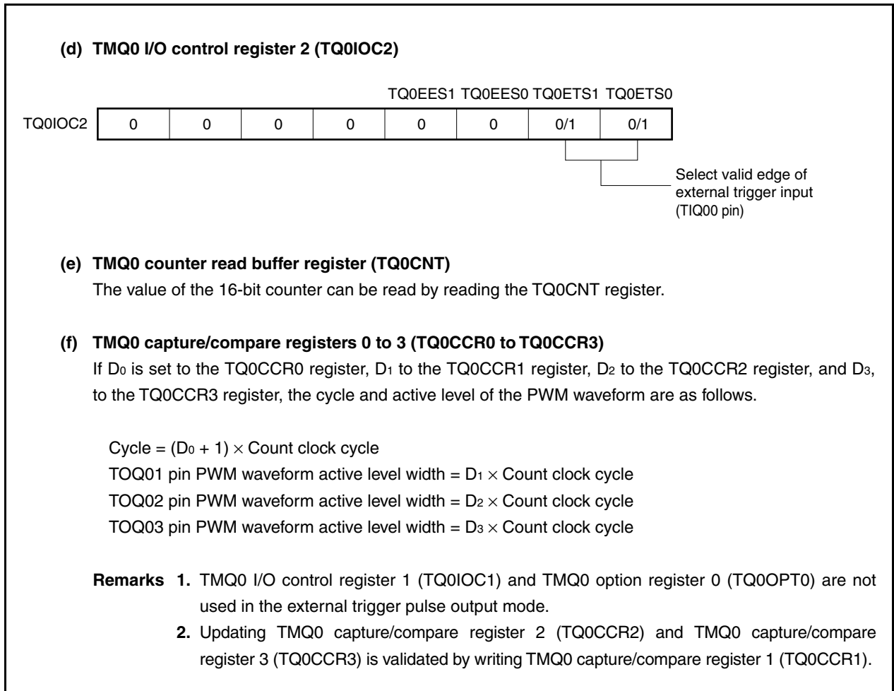
Figure 8-22. Setting of Registers in External Trigger Pulse Output Mode (3/3)
