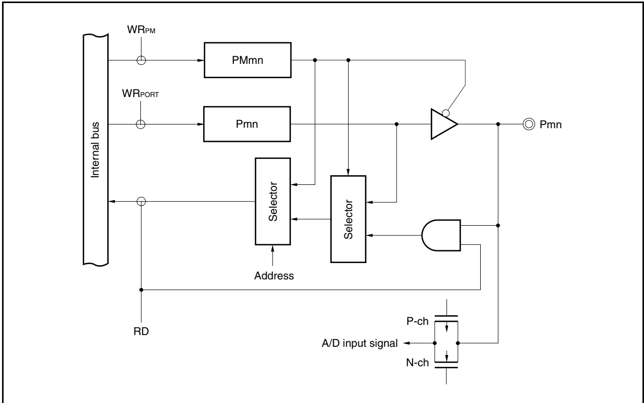
Figure 4-4. Block Diagram of Type A-1
