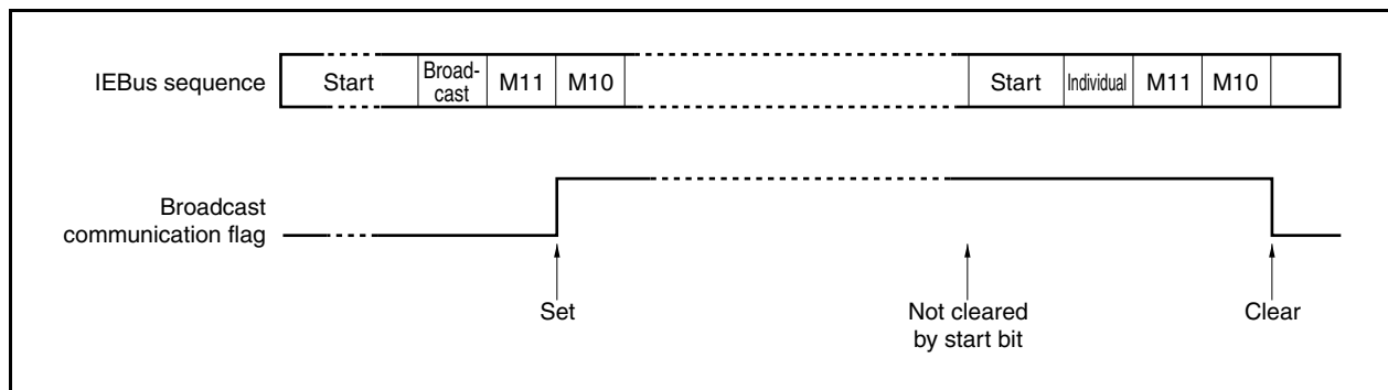
Figure 20-12. Example of Broadcast Communication Flag Operation
