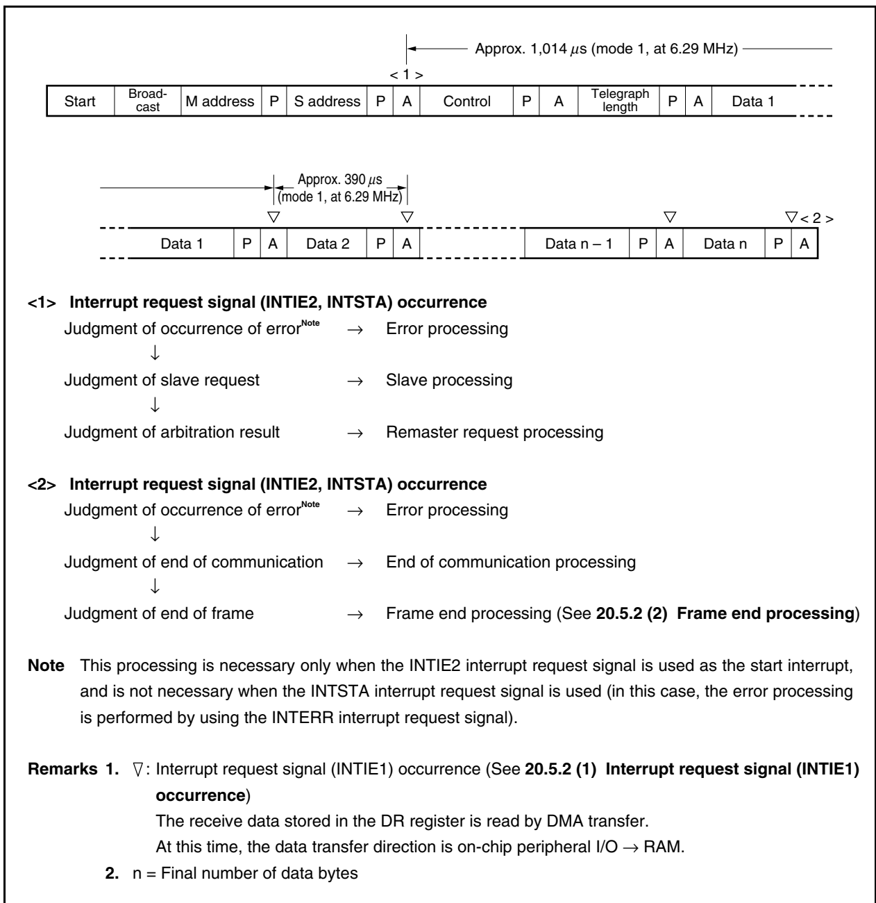
Figure 20-27. Master Reception
