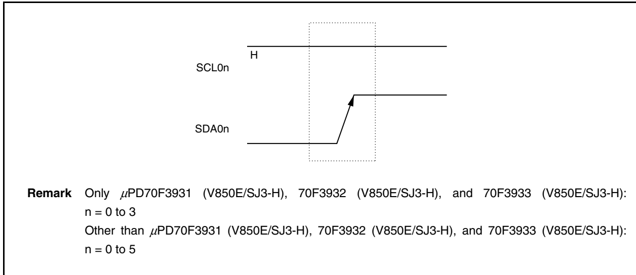
Figure 19-9. Stop Condition
