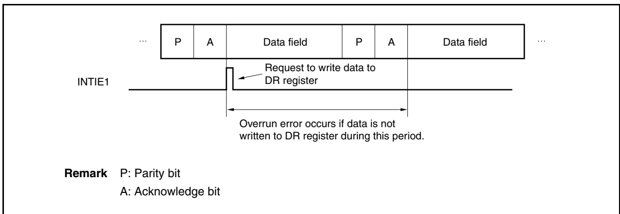
Figure 20-14. Timing of Overrun Error Occurrence
