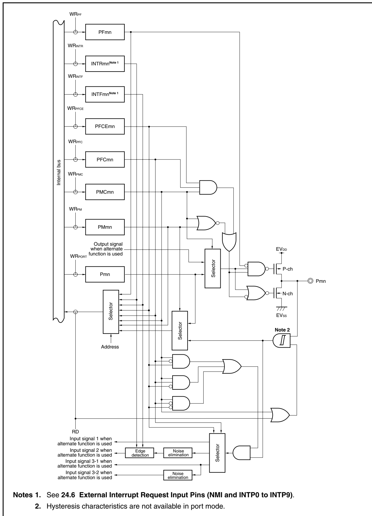
Figure 4-54. Block Diagram of Type U-26
