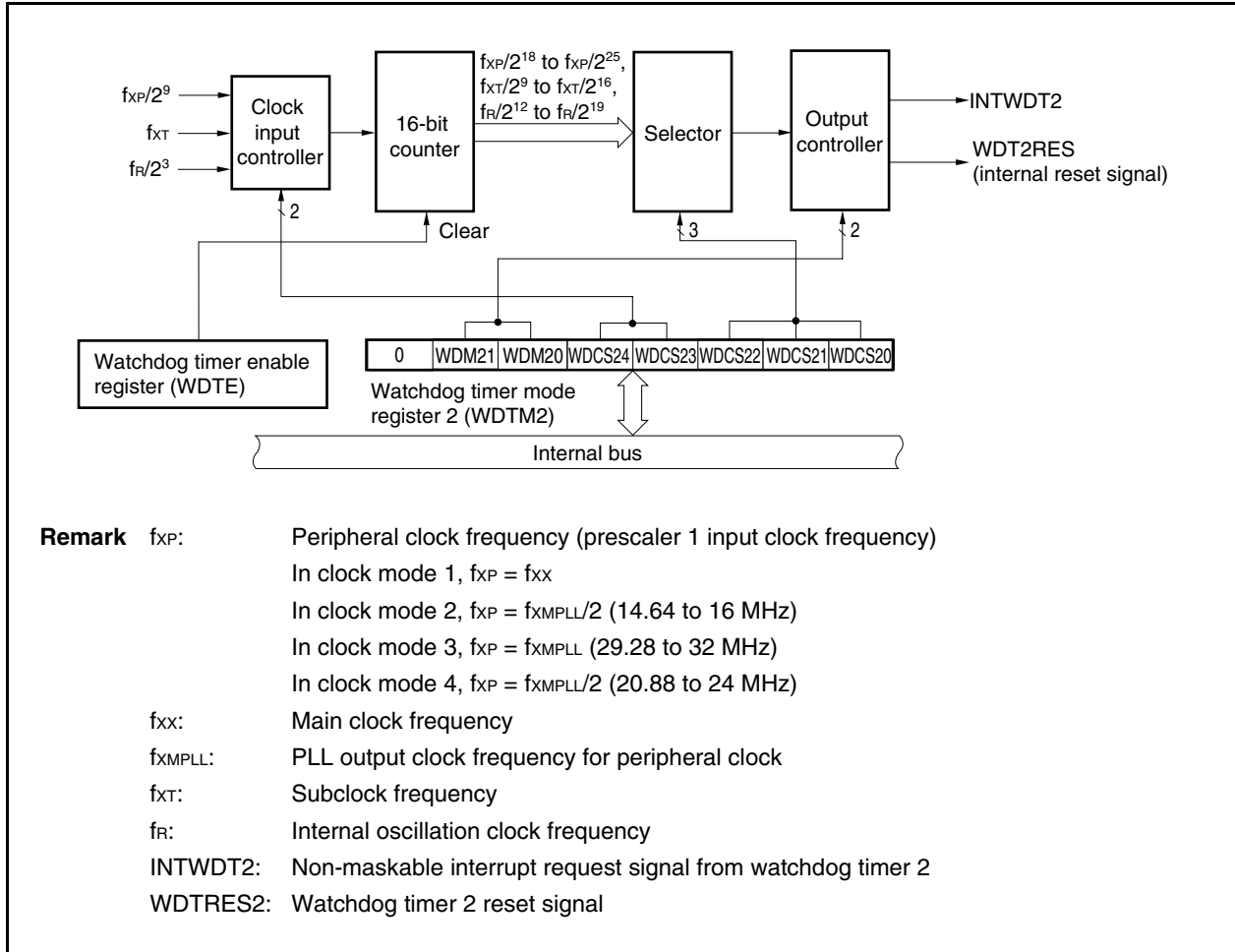
Figure 11-1. Block Diagram of Watchdog Timer 2
