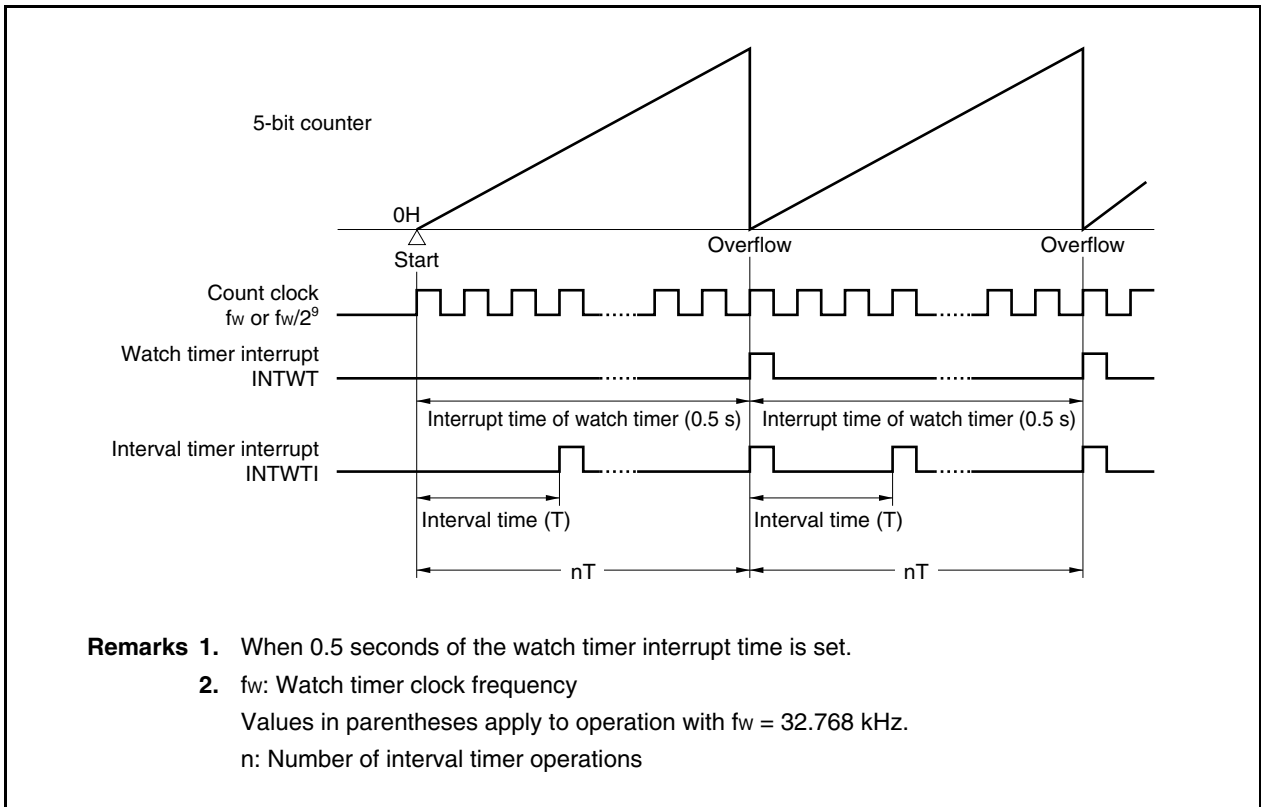
Figure 10-4. Operation Timing of Watch Timer/Interval Timer
