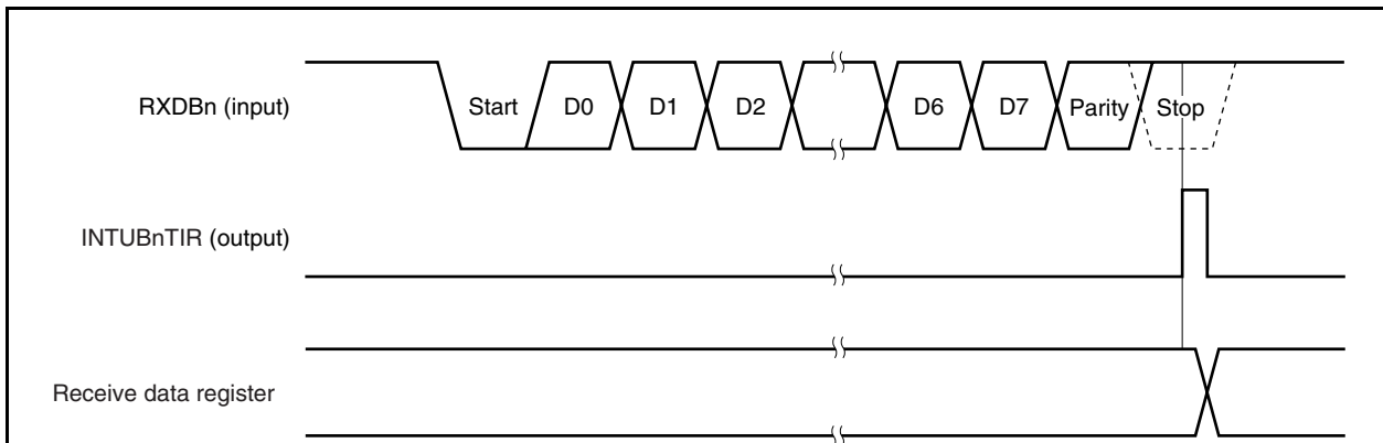
Figure 16-5. Timing of Asynchronous Serial Interface Reception Completion Interrupt Request Signal (INTUBnTIR)
