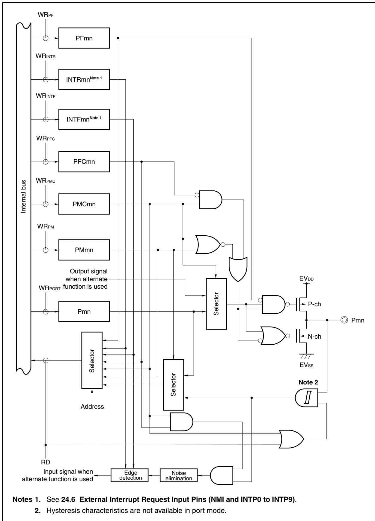
Figure 4-26. Block Diagram of Type N-2
