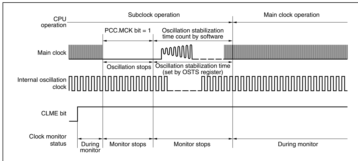
Figure 28-5. Operation When Main Clock Is Stopped (Arbitrary)
