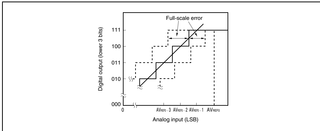
Figure 13-19. Full-Scale Error
