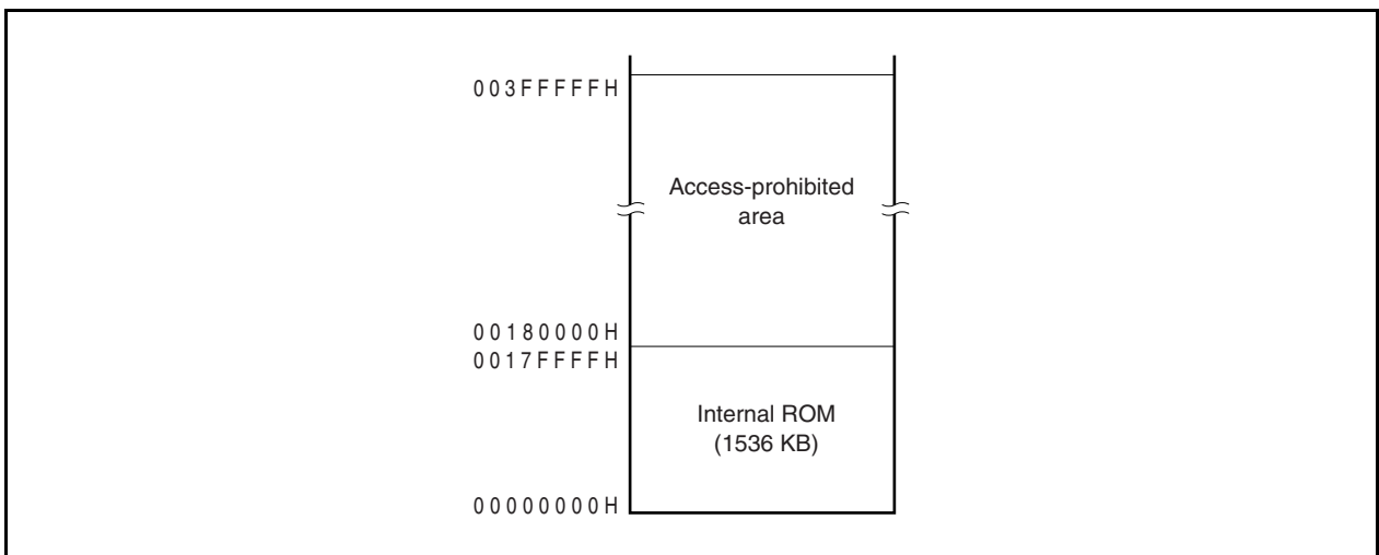
Figure 3-8. Internal ROM Area (1536 KB)
