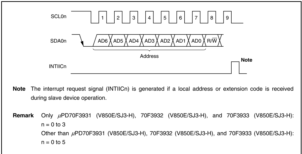
Figure 19-6. Address
