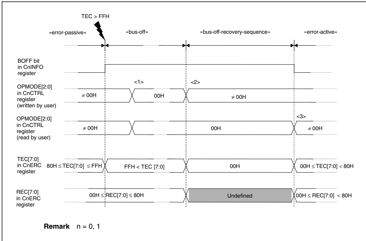
Figure 21-17. Recovery from Bus-off State Through Normal Recovery Sequence
