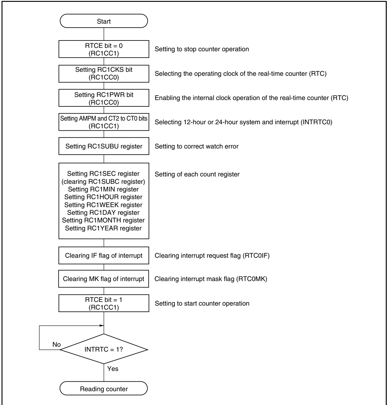
Figure 10-7. Initialization Procedure
