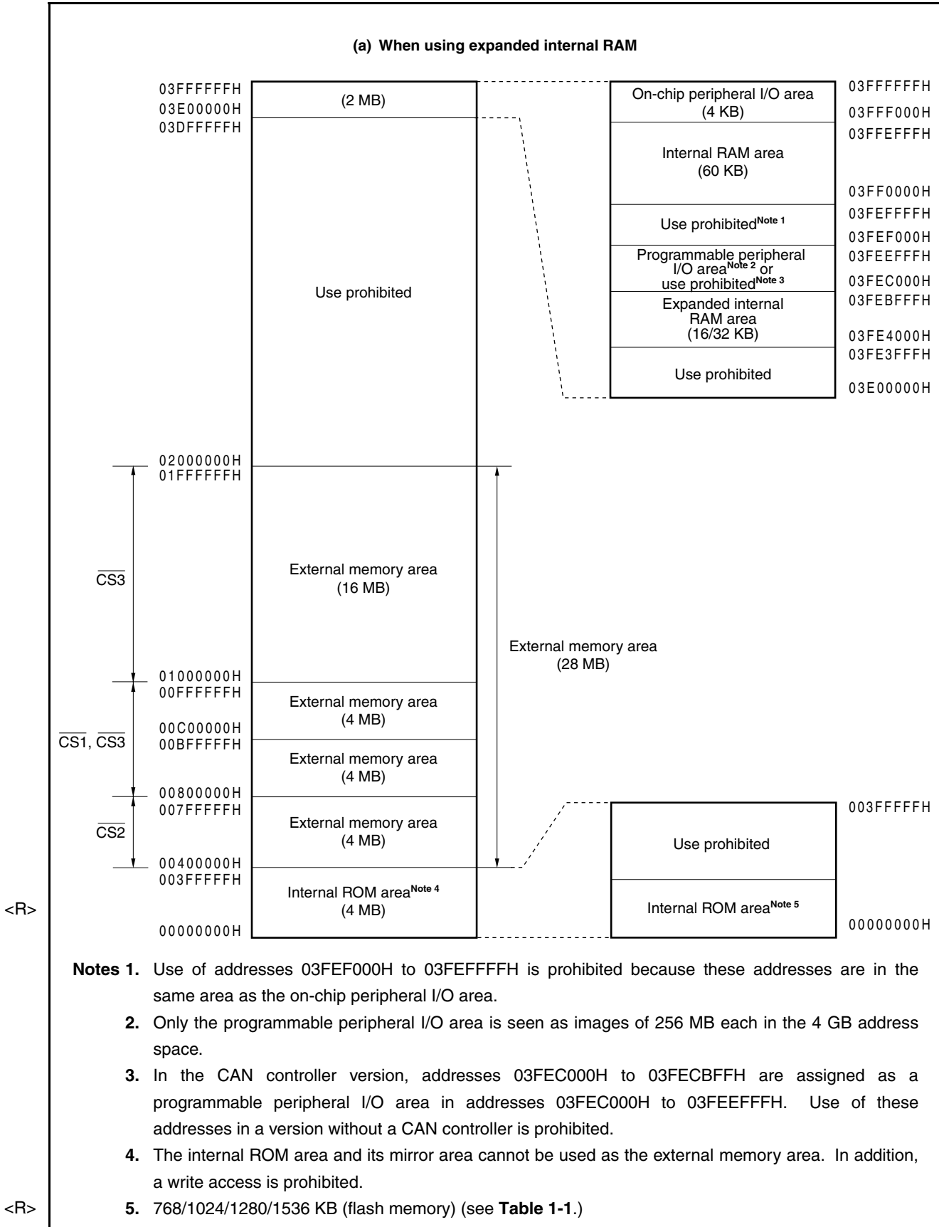
Figure 5-1. Data Memory Map: Physical Address (1/2)
