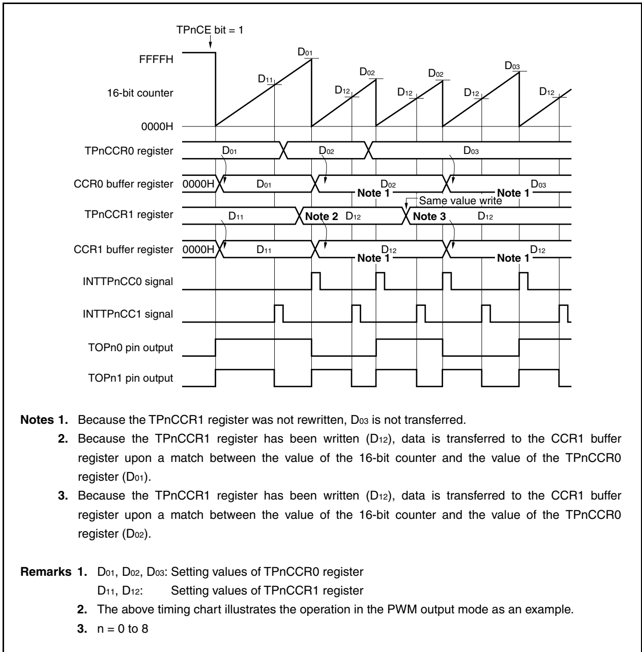
Figure 7-7. Timing of Batch Write
