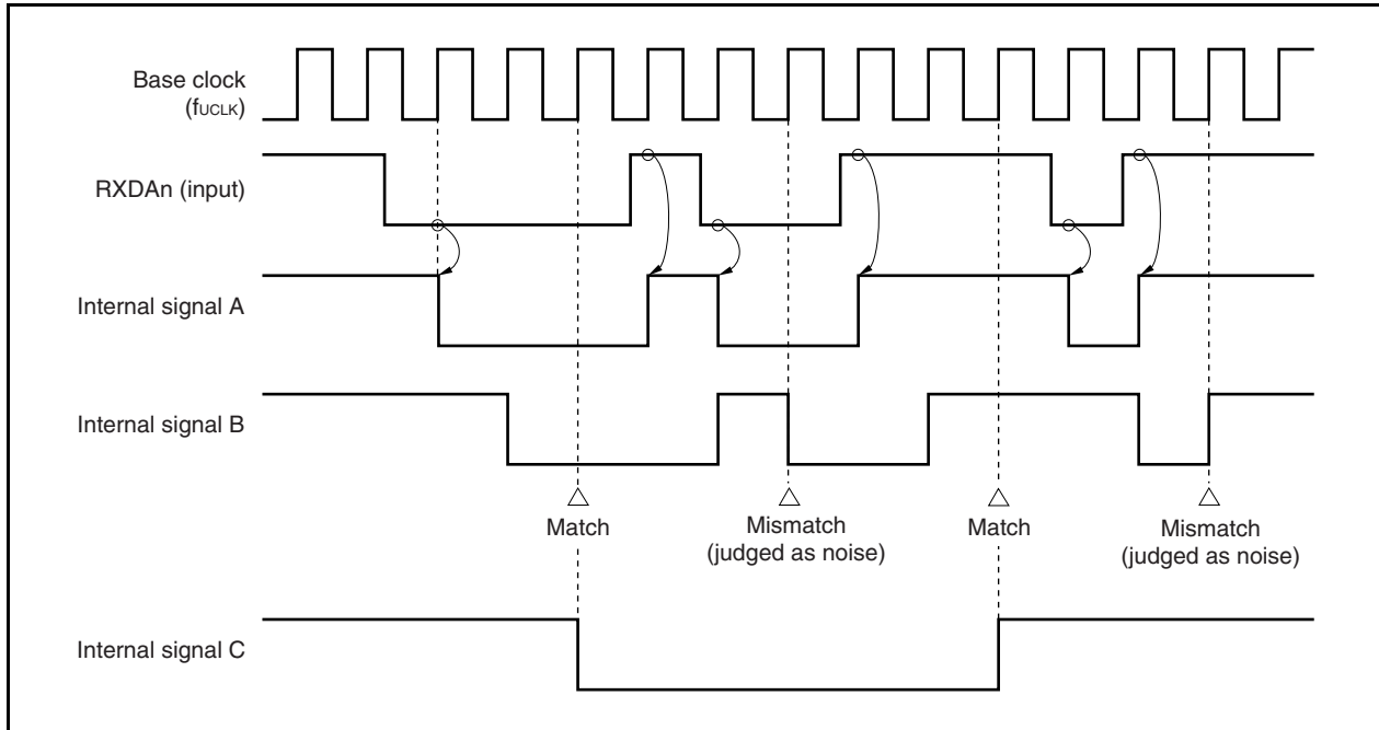
Figure 15-12. Timing of RXDAn Signal Judged as Noise
