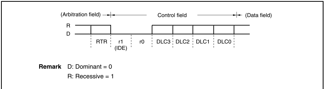
Figure 21-8. Control Field
