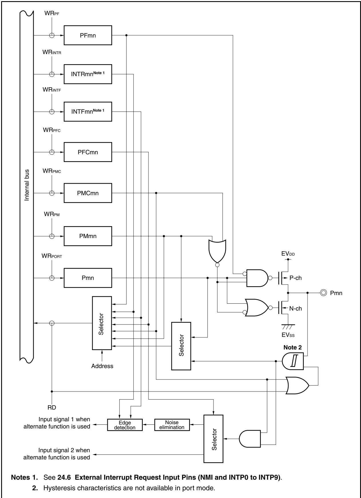
Figure 4-25. Block Diagram of Type N-1
