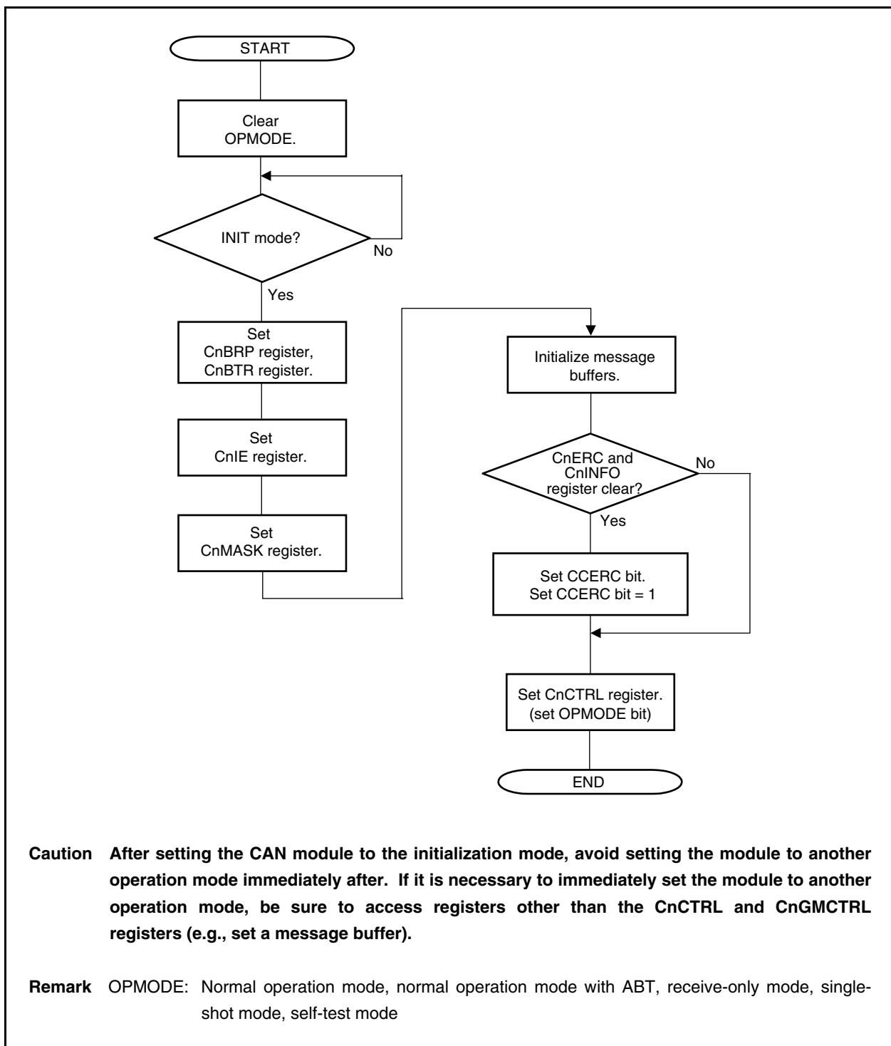
Figure 21-37. Re-initialization
