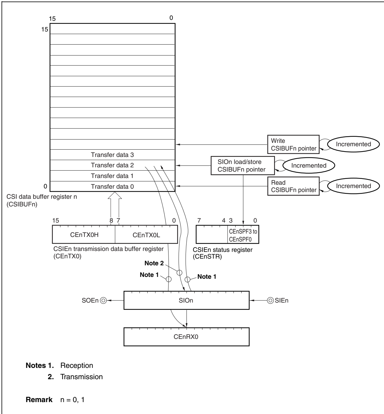
Figure 18-11. Continuous Mode
