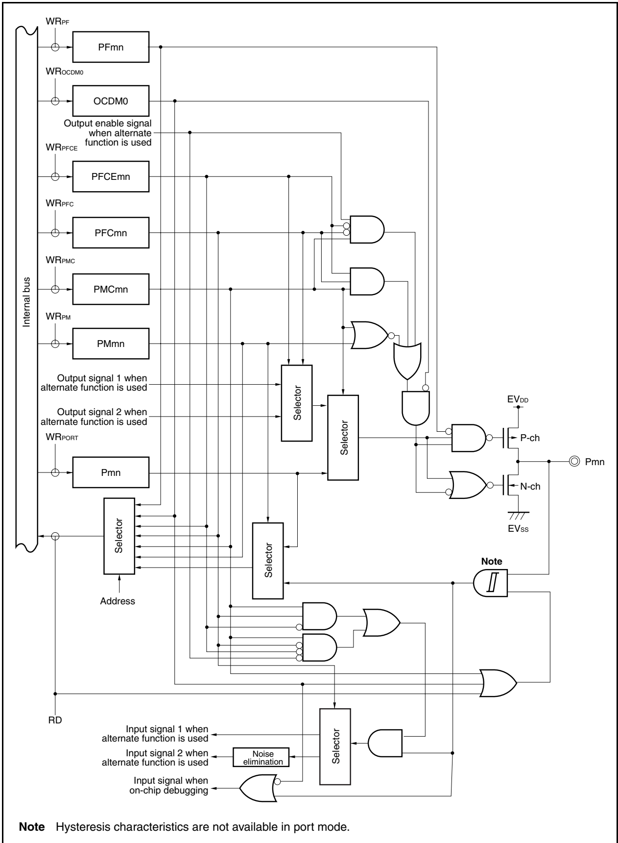
Figure 4-37. Block Diagram of Type U-9
