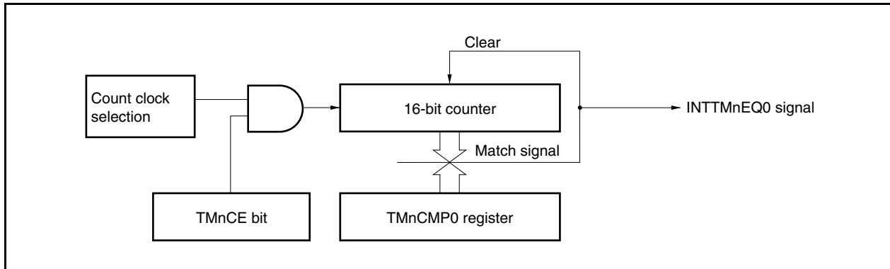
Figure 9-3. Configuration of Interval Timer
