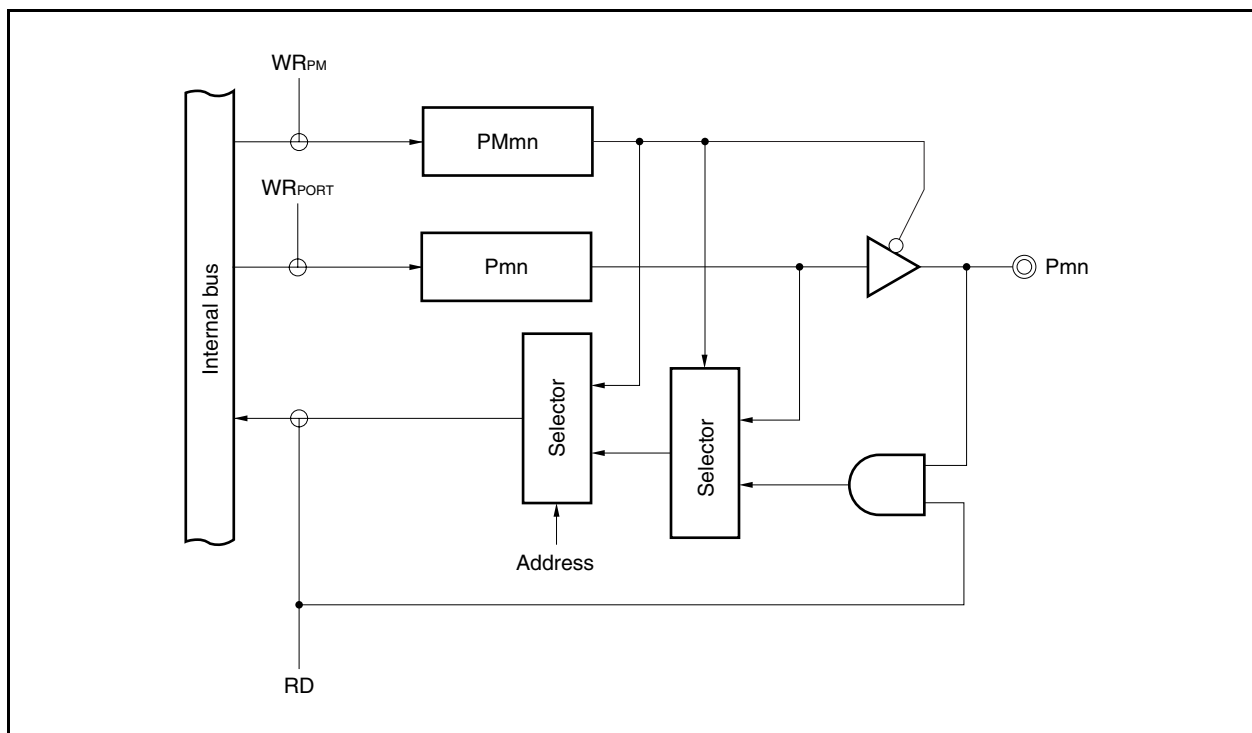
Figure 4-6. Block Diagram of Type B-1
