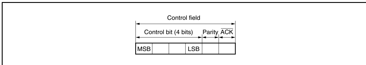
Figure 20-4. Control Field
