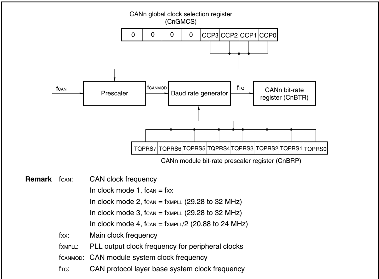
Figure 21-23. CAN Module Clock
