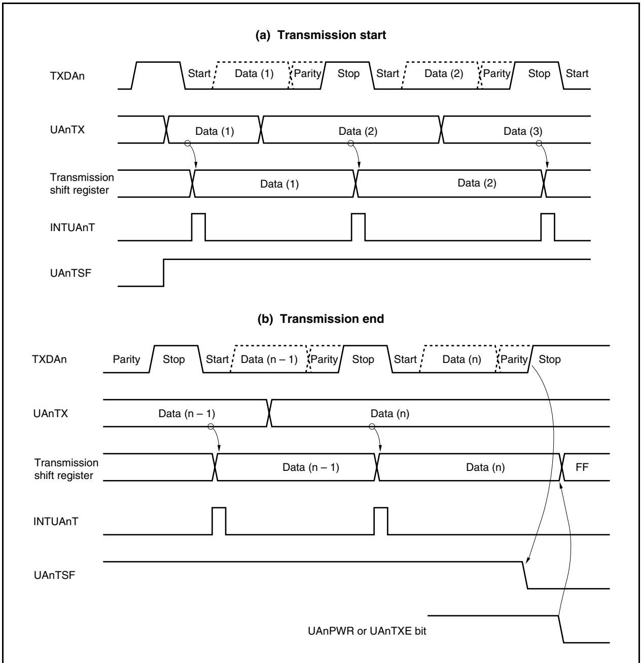
Figure 15-9. Continuous Transmission Operation Timing
