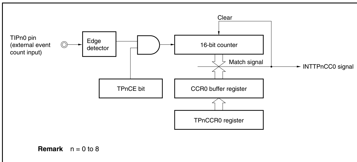
Figure 7-15. Configuration in External Event Count Mode
