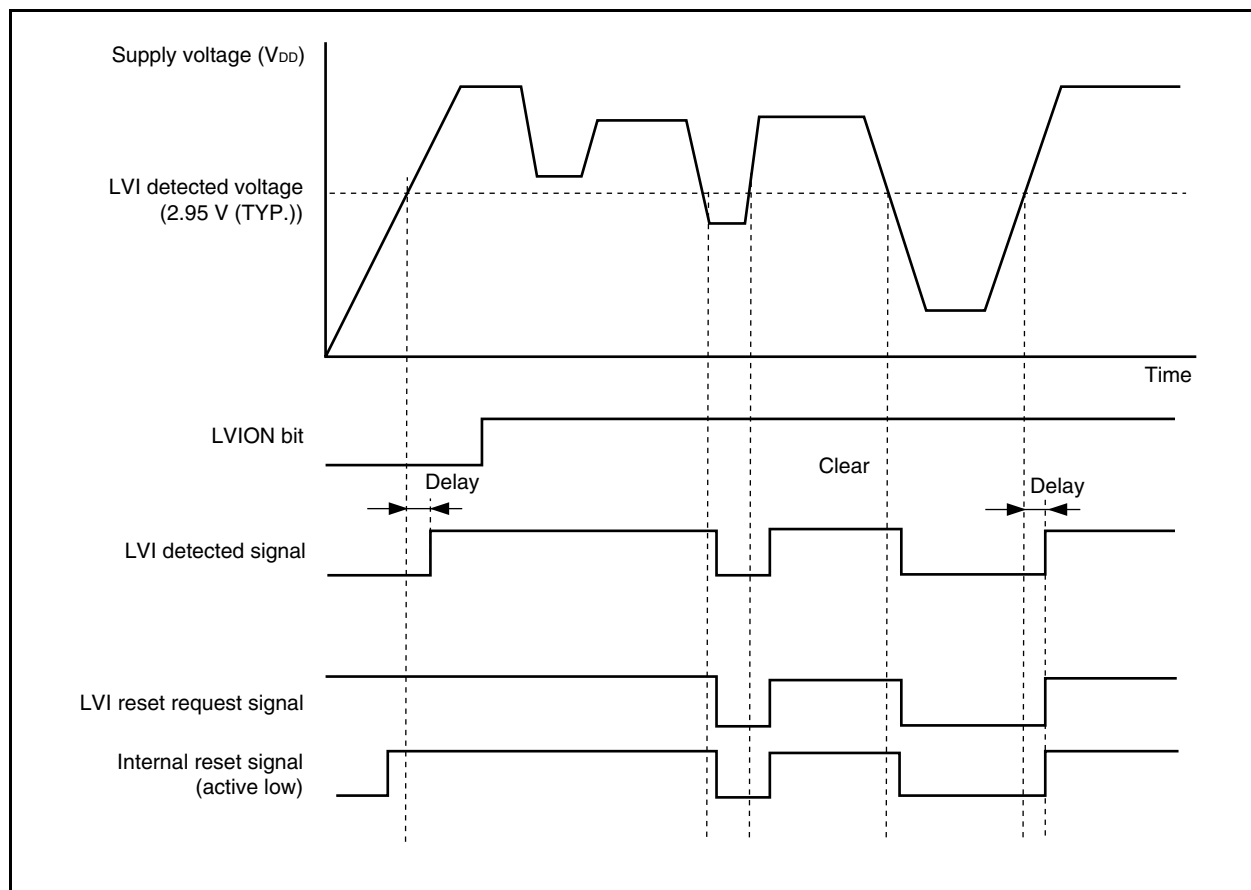
Figure 29-2. Operation Timing of Low-Voltage Detector (LVIMD Bit = 1)
