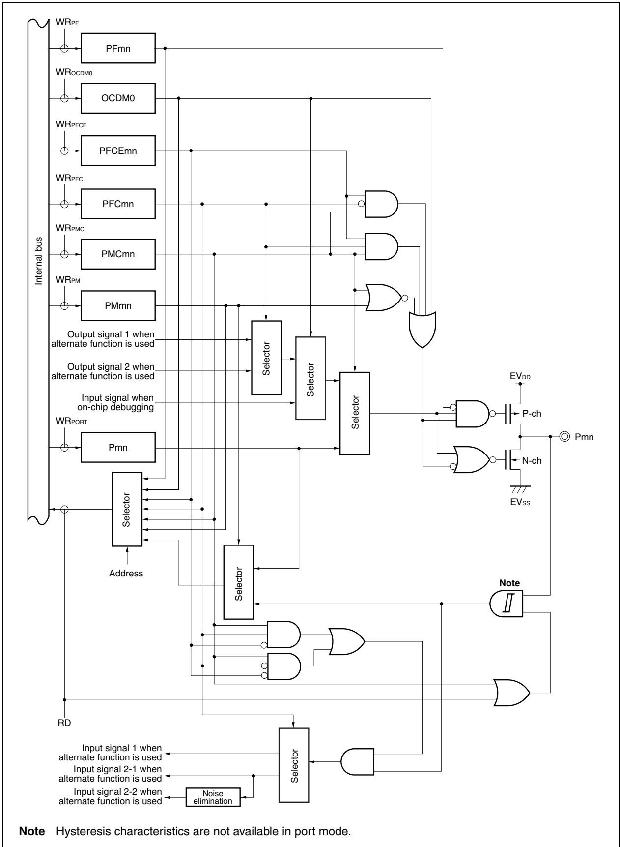
Figure 4-35. Block Diagram of Type U-7
