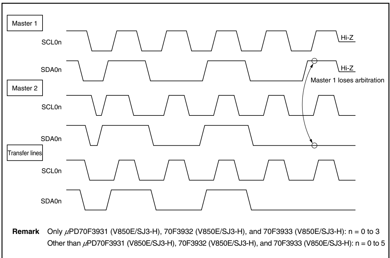
Figure 19-11. Arbitration Timing Example
