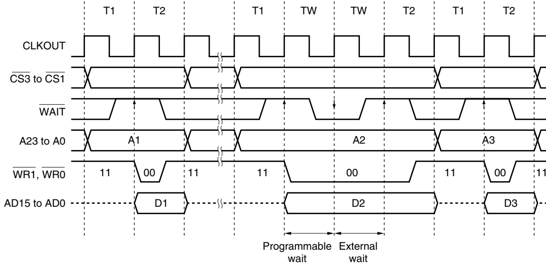
Figure 5-13. Separate Bus Write Timing (Bus Size: 16 Bits, 16-Bit Access)
