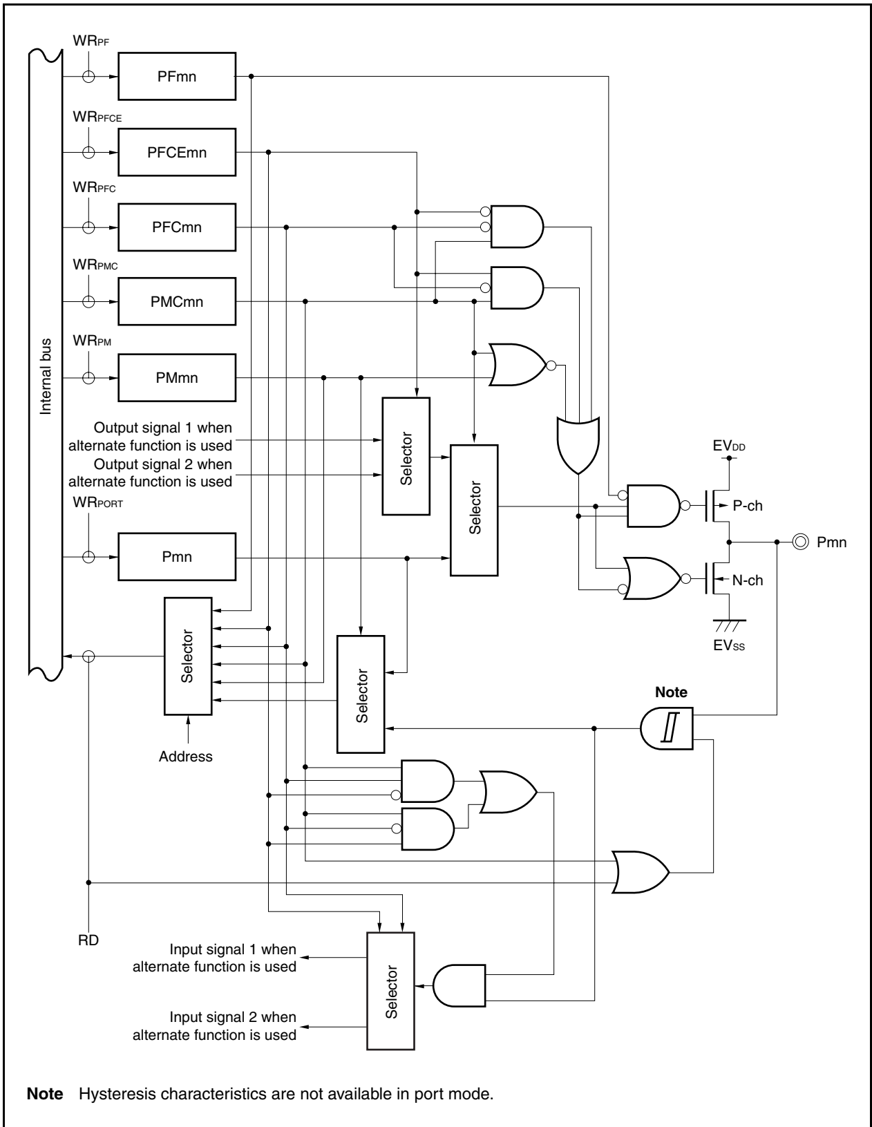
Figure 4-55. Block Diagram of Type U-27
