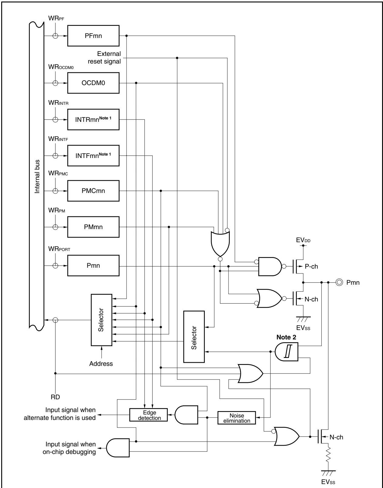
Figure 4-67. Block Diagram of Type AA-1
