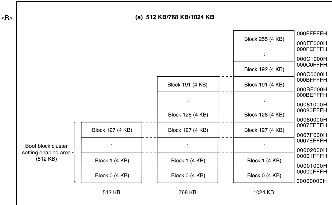
Figure 32-1. Flash Memory Mapping (1/2)
