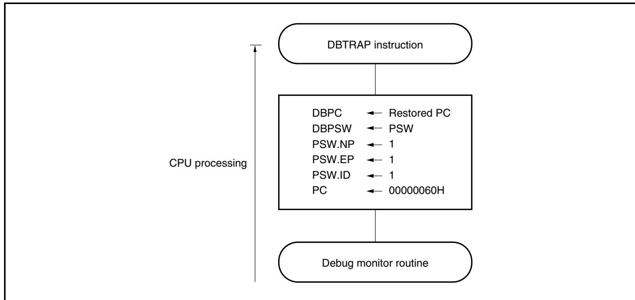
Figure 24-13. Debug Trap Processing Format
