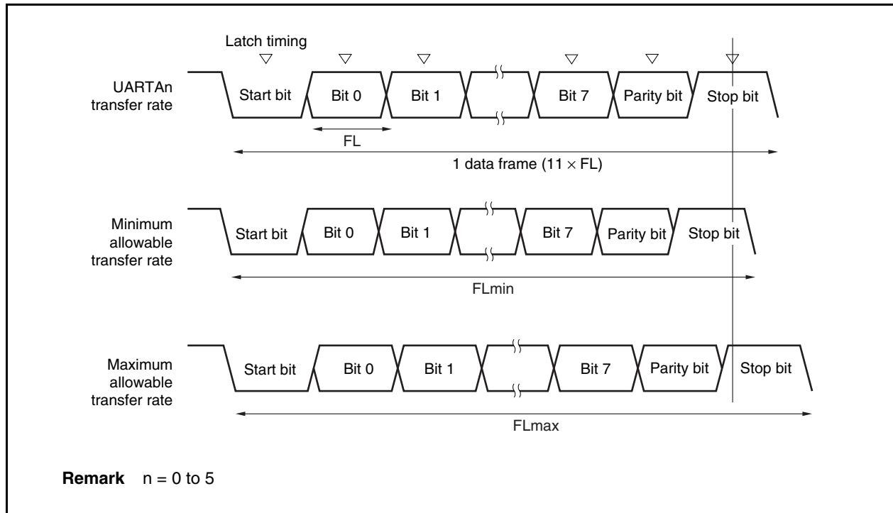
Figure 15-14. Allowable Baud Rate Range During Reception
