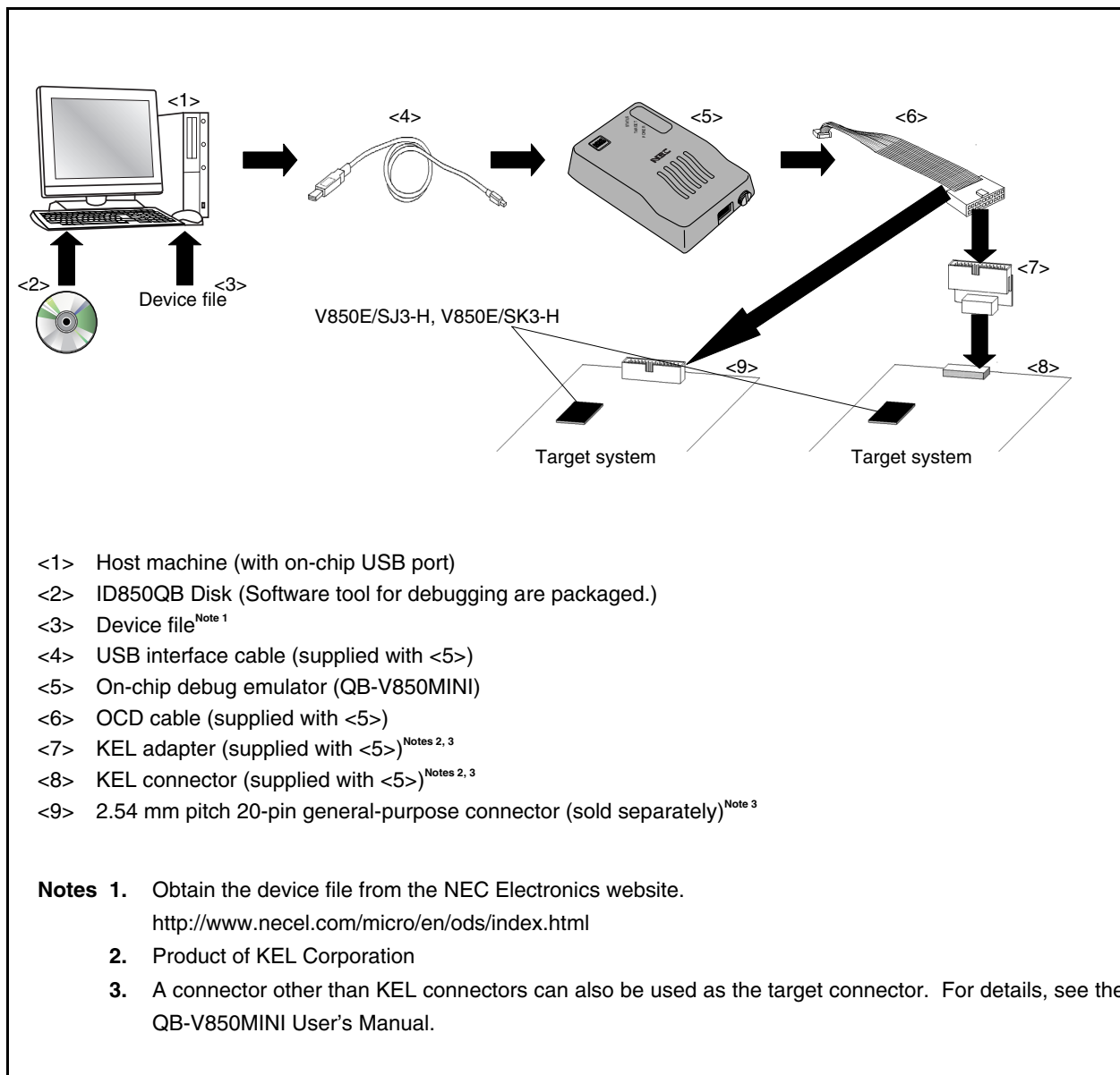
Figure A-4. System Configuration (QB-V850MINI Used)
