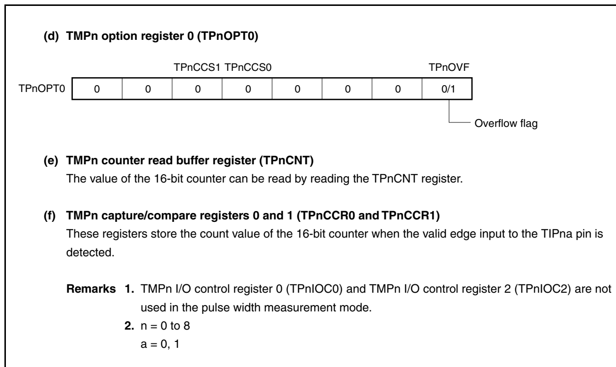
Figure 7-42. Register Setting in Pulse Width Measurement Mode (2/2)
