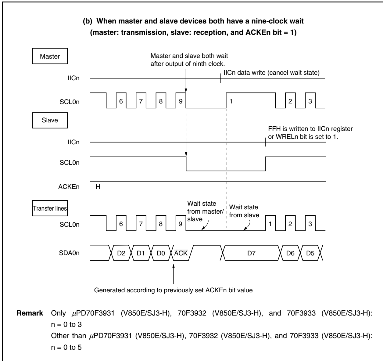
Figure 19-10. Wait State (2/2)
