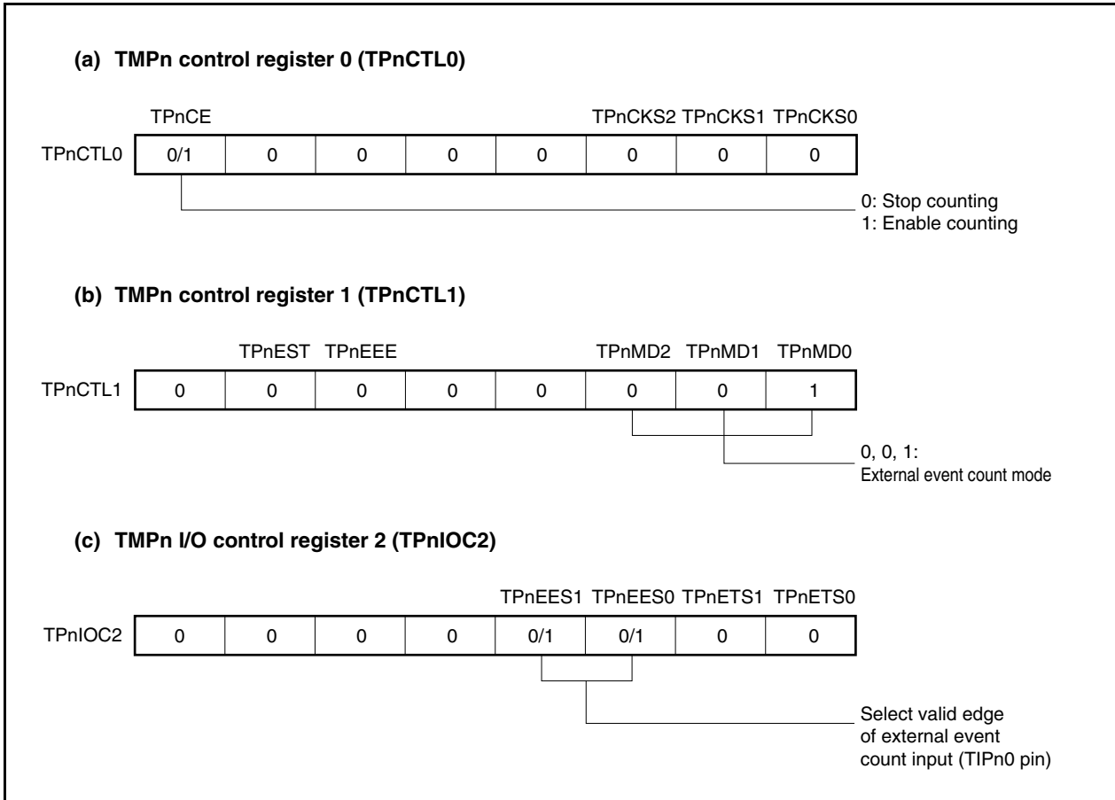
Figure 7-17. Register Setting for Operation in External Event Count Mode (1/2)
