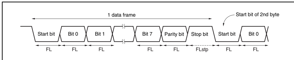
Figure 15-15. Transfer Rate During Continuous Transfer
