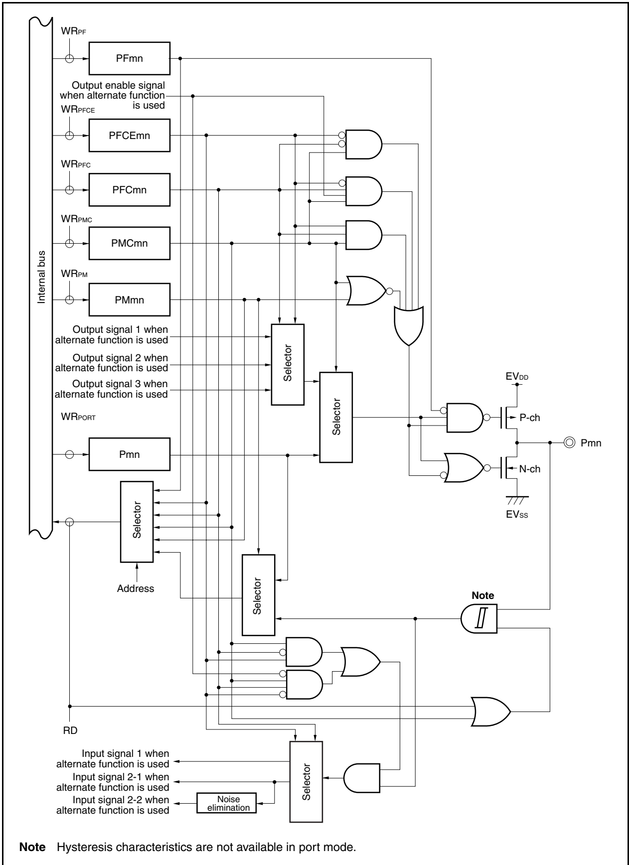
Figure 4-53. Block Diagram of Type U-25
