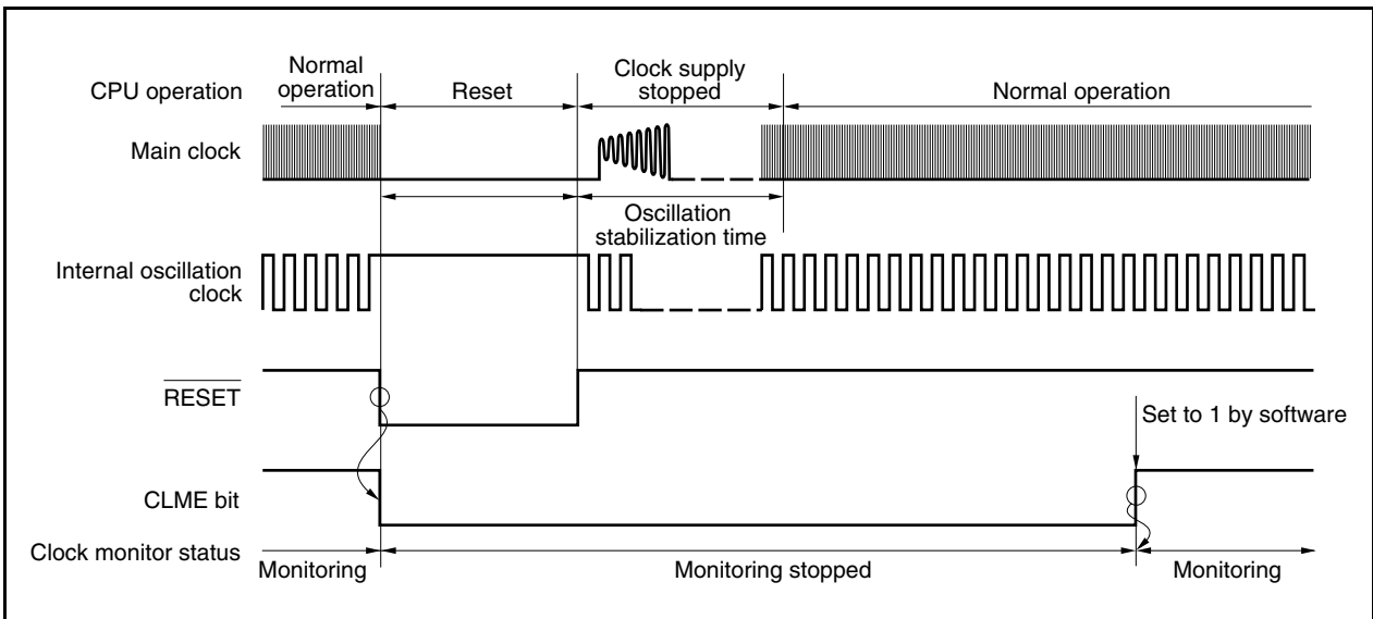
Figure 28-3. Clock Monitor Status After \overline{\text{RESET}} Input
