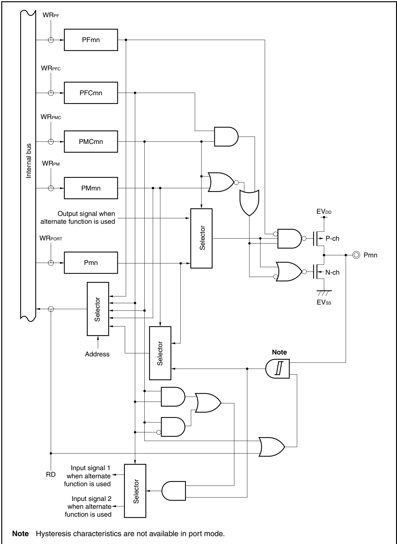
Figure 4-21. Block Diagram of Type G-5
