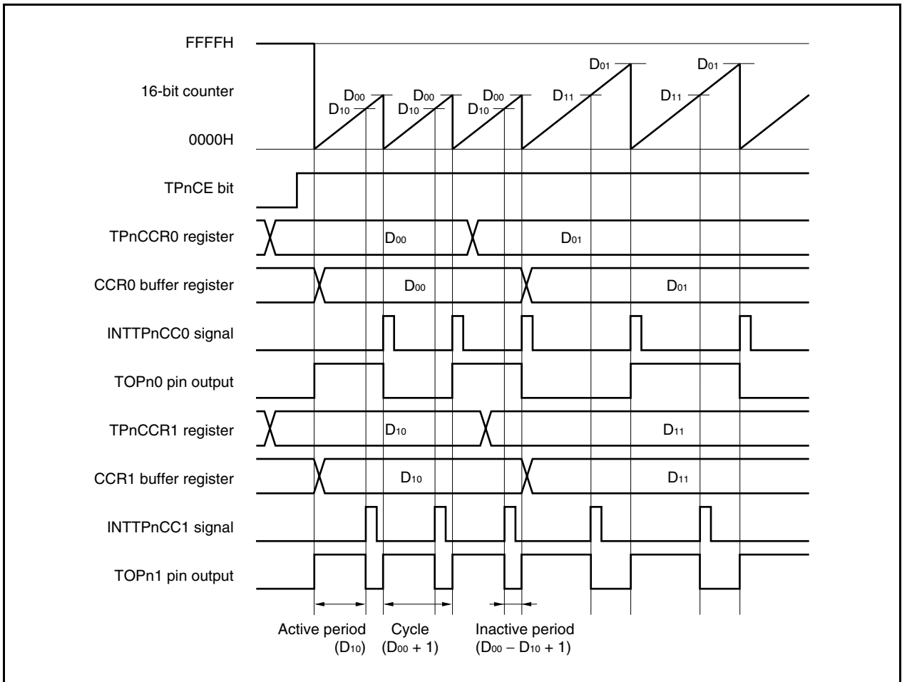
Figure 7-31. Basic Timing in PWM Output Mode
