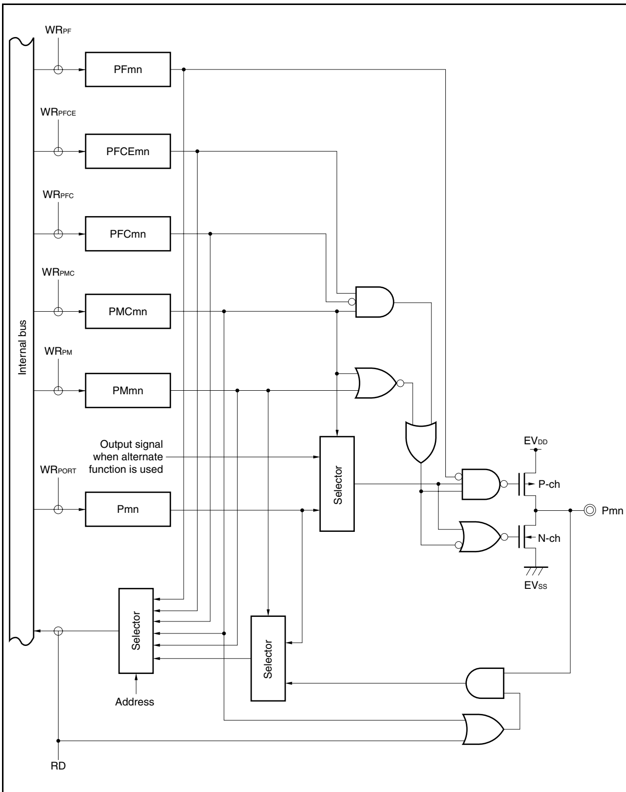
Figure 4-47. Block Diagram of Type U-19
