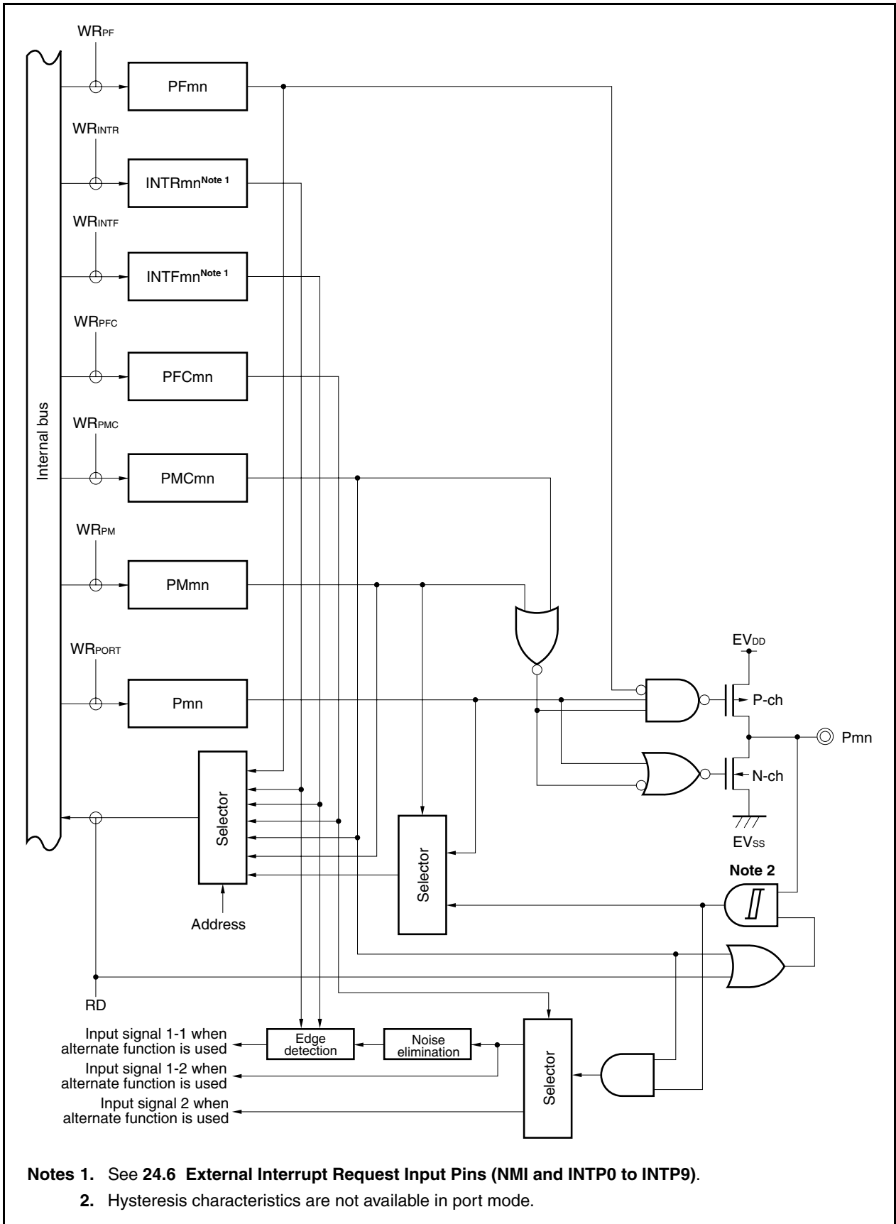
Figure 4-27. Block Diagram of Type N-3
