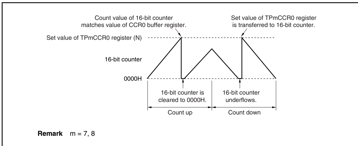
Figure 7-50. Operation Example (Count Operation in Range from 0000H to Set Value of TPmCCR0 Register)
