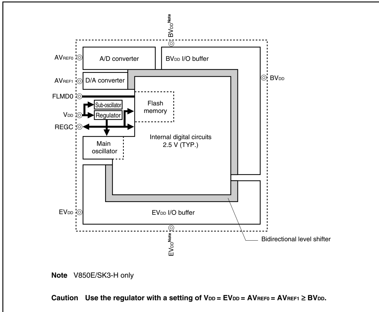
Figure 30-1. Regulator
