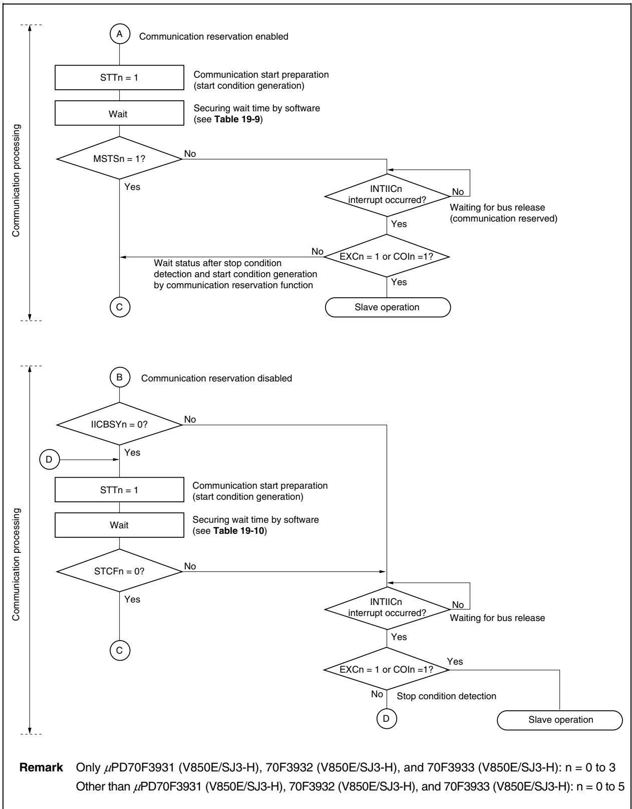
Figure 19-16. Master Operation in Multimaster System (2/3)
