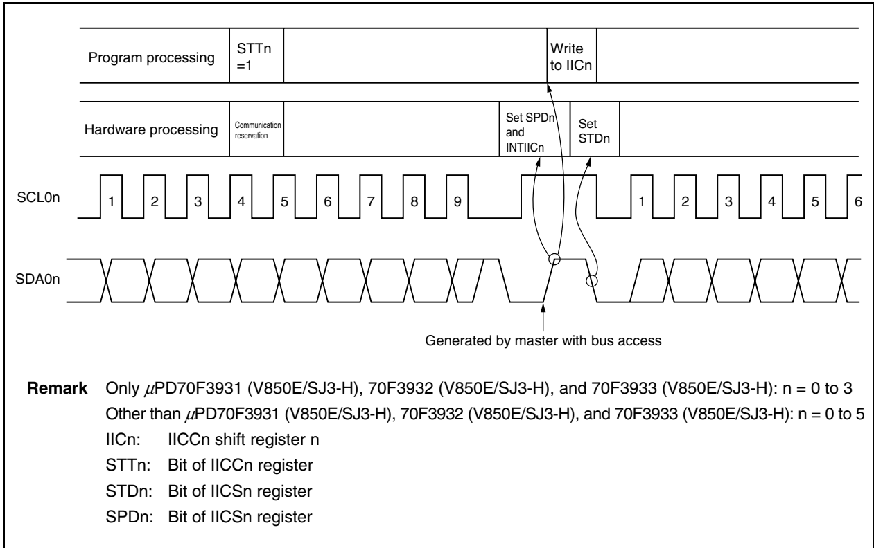
Figure 19-12. Communication Reservation Timing
