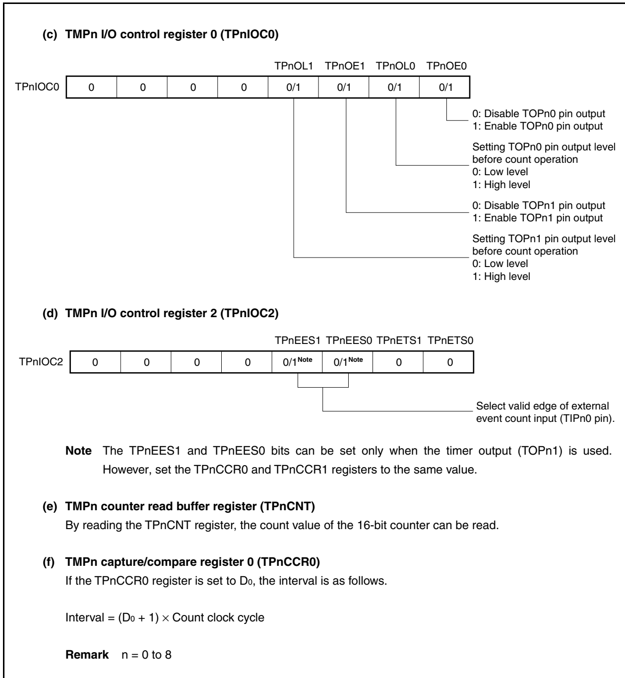
Figure 7-10. Register Setting for Interval Timer Mode Operation (2/3)
