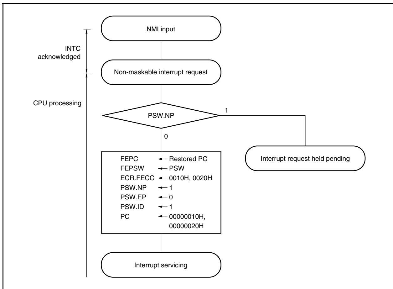
Figure 24-2. Servicing Configuration of Non-Maskable Interrupt
