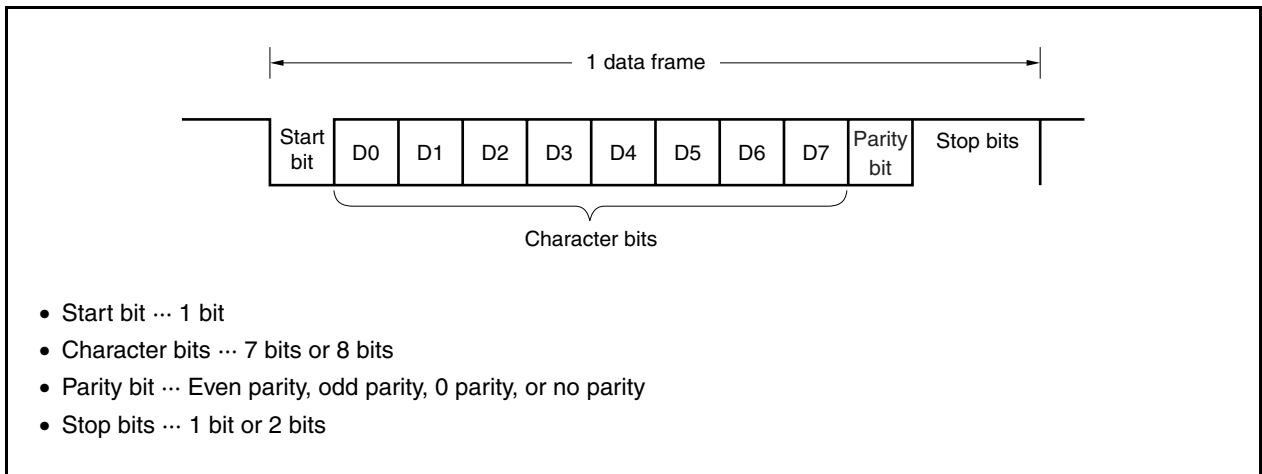
Figure 16-2. Asynchronous Serial Interface Transmit/Receive Data Format (LSB-First Transfer)
