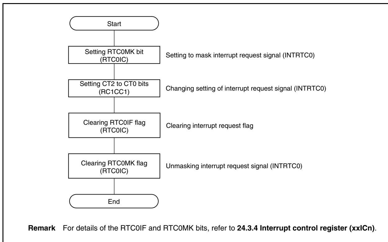
Figure 10-10. Changing Setting of INTRTC0 Interrupt During Clock Operation
