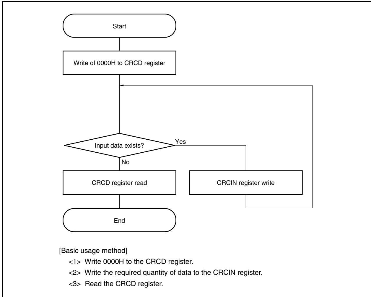
Figure 23-3. CRC Operation Flow
