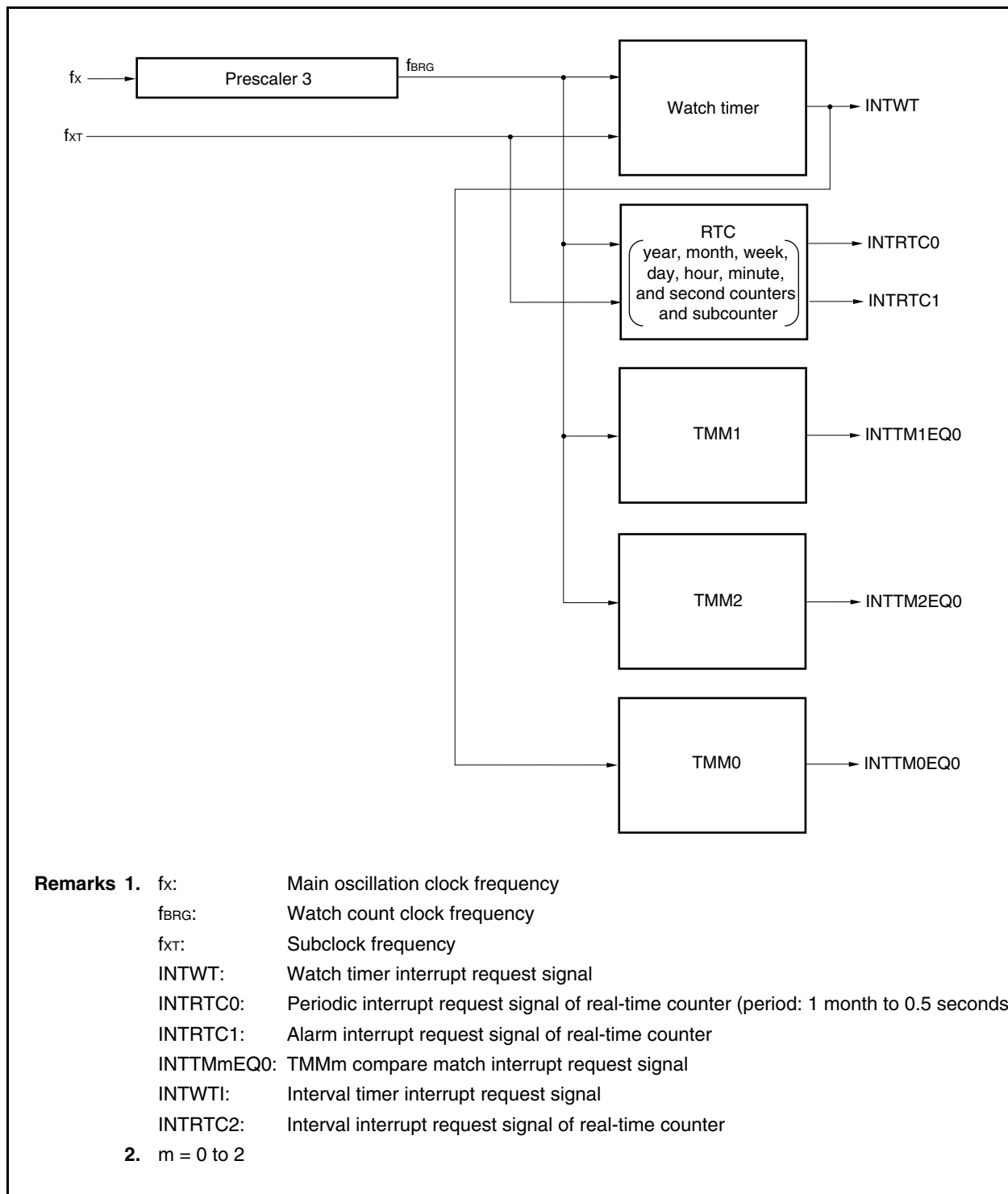
Figure 10-1. Block Diagram of Watch Function
