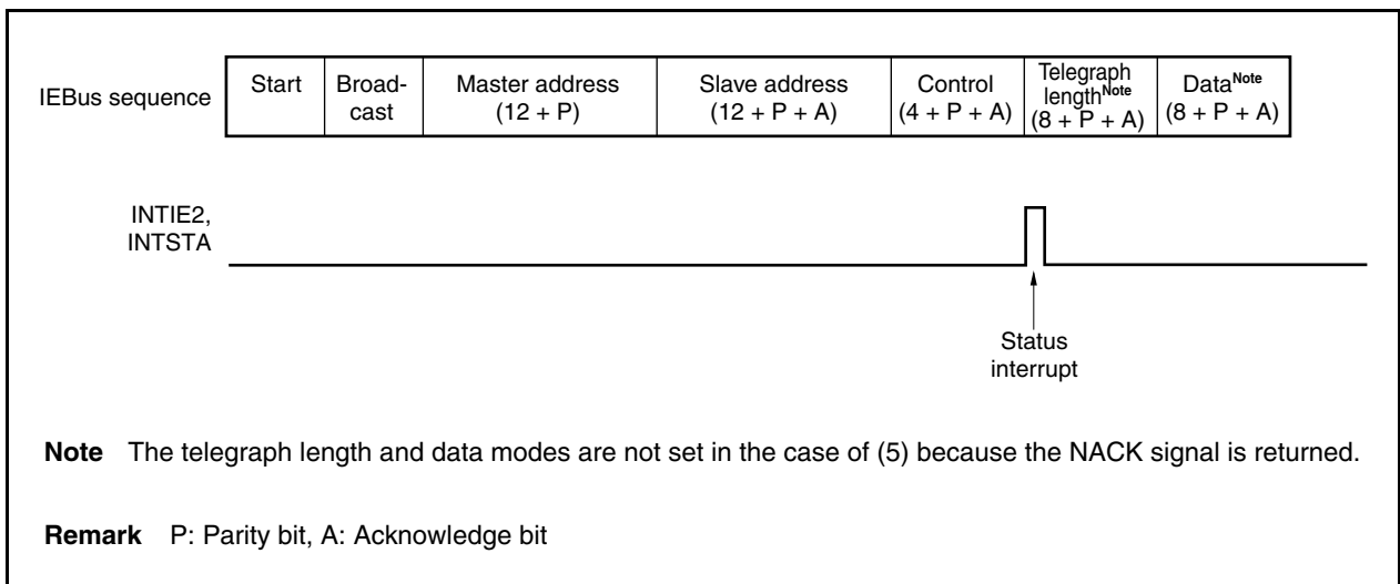
Figure 20-18. Timing of INTIE2 and INTSTA Interrupt Request Signal Generation in Locked State (for (4) and (5))
