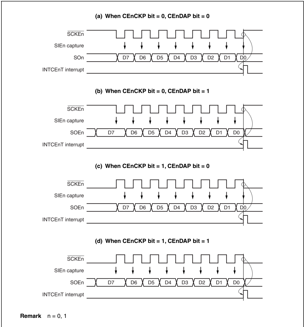
Figure 18-7. Clock Timing
