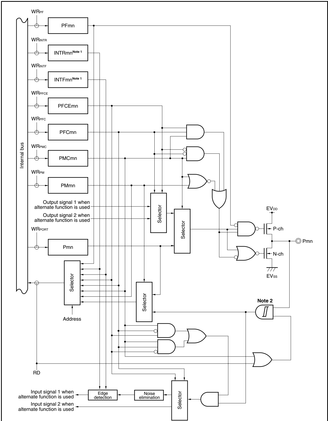
Figure 4-43. Block Diagram of Type U-15
