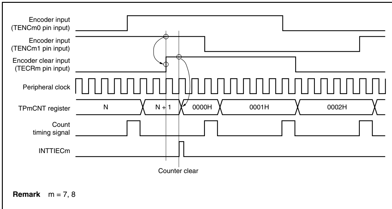
Figure 7-52. Operation Example (When TPmSCE Bit = 0, TPmESC1 and TPmECS0 Bits = 01, and TPmUDS1 and TPmUDS0 Bits = 11)
