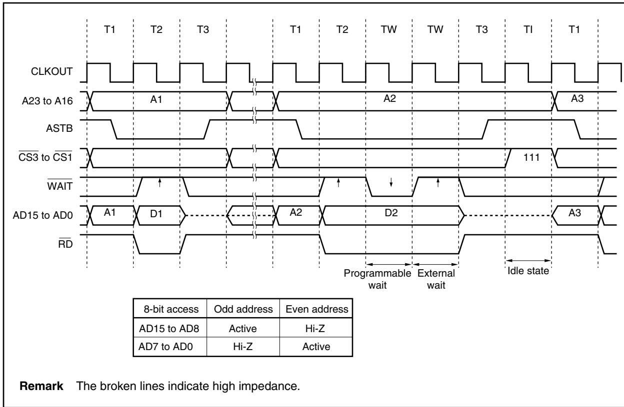
Figure 5-6. Multiplexed Bus Read Timing (Bus Size: 16 Bits, 16-Bit Access)
