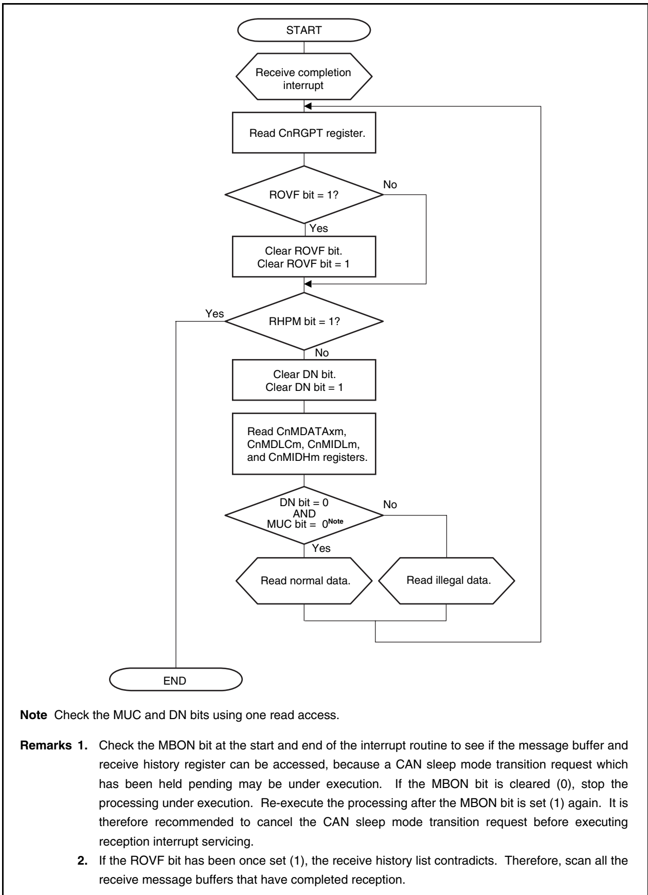
Figure 21-50. Reception via Interrupt (Using CnRGPT Register)
