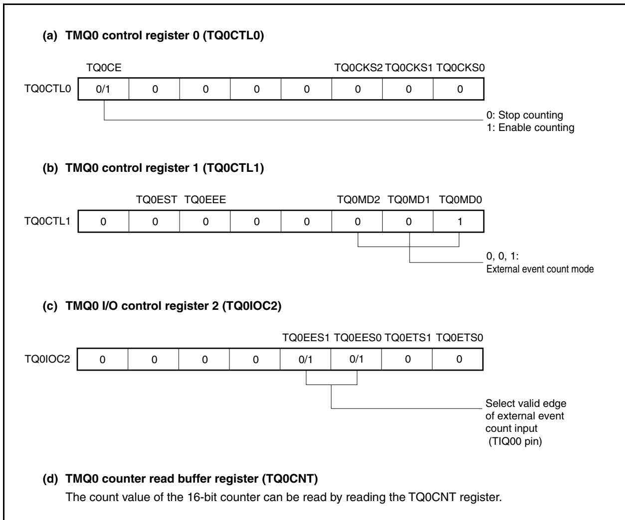
Figure 8-15. Register Setting for Operation in External Event Count Mode (1/2)
