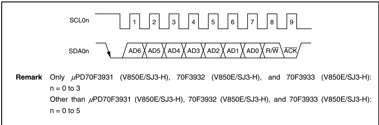
Figure 19-8. \overline{\text{ACK}}
