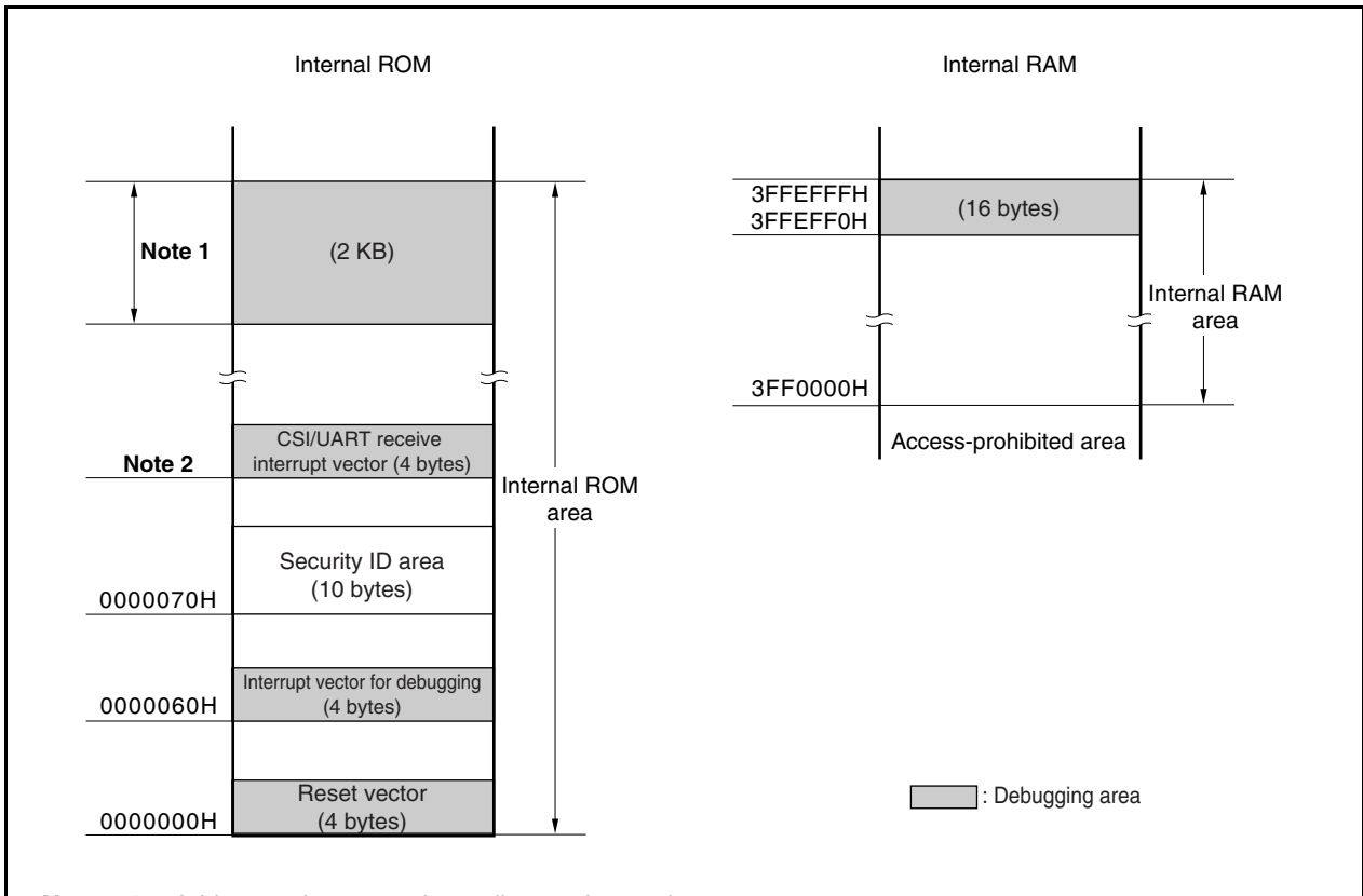
Figure 34-4. Memory Spaces Where Debug Monitor Programs Are Allocated
