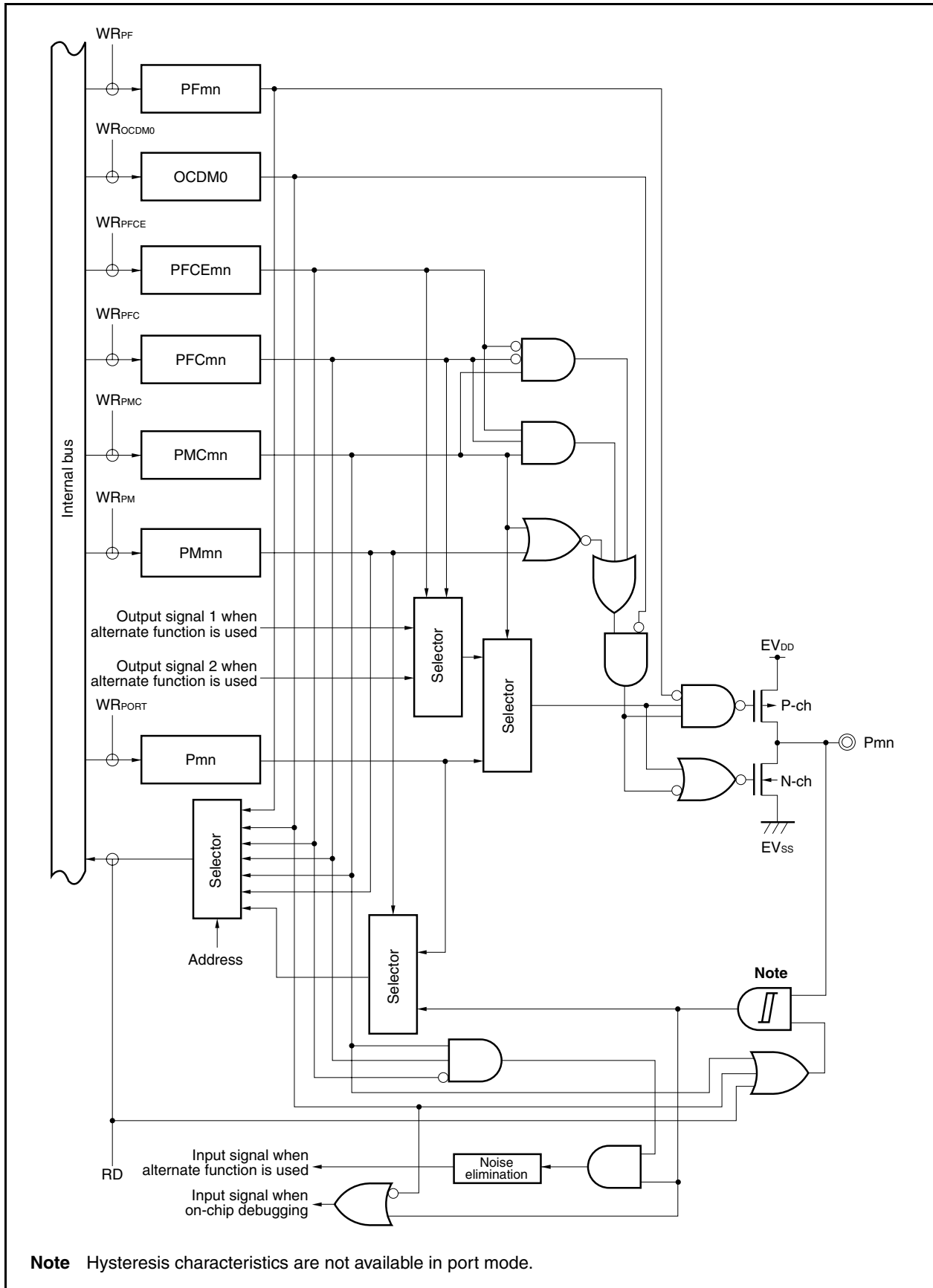
Figure 4-36. Block Diagram of Type U-8
