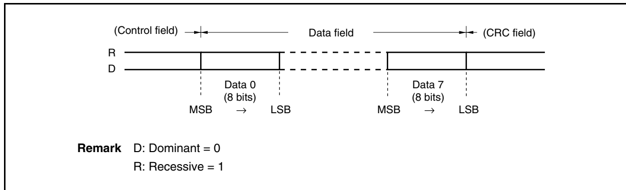
Figure 21-9. Data Field
