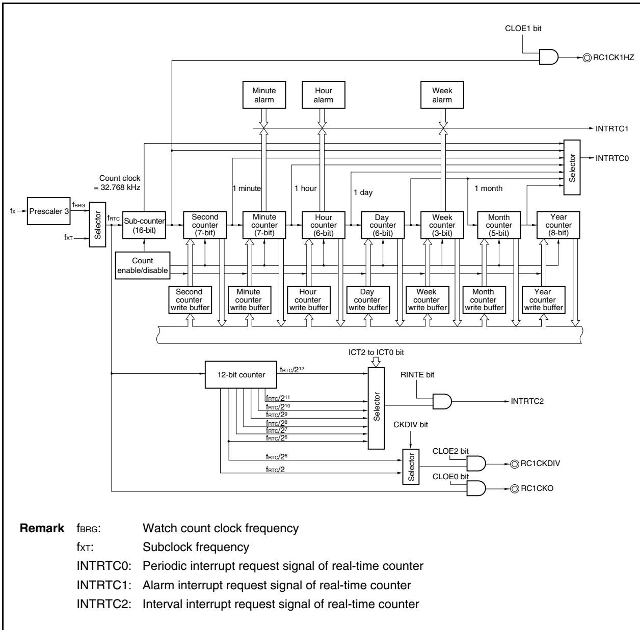
Figure 10-6. Block Diagram of Real-Time Counter
