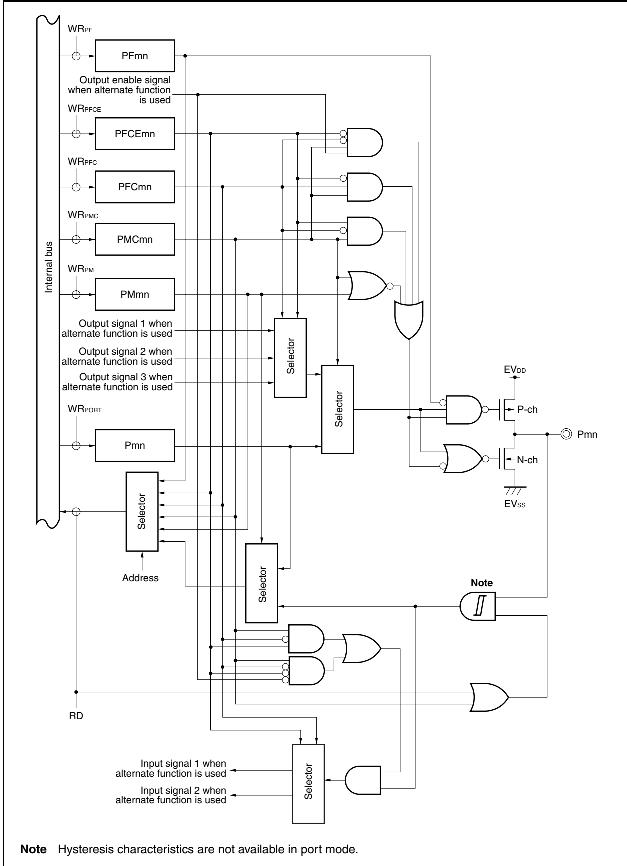
Figure 4-56. Block Diagram of Type U-28
