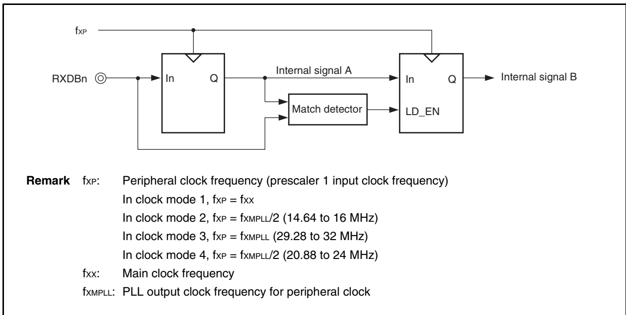
Figure 16-6. Noise Filter Circuit
