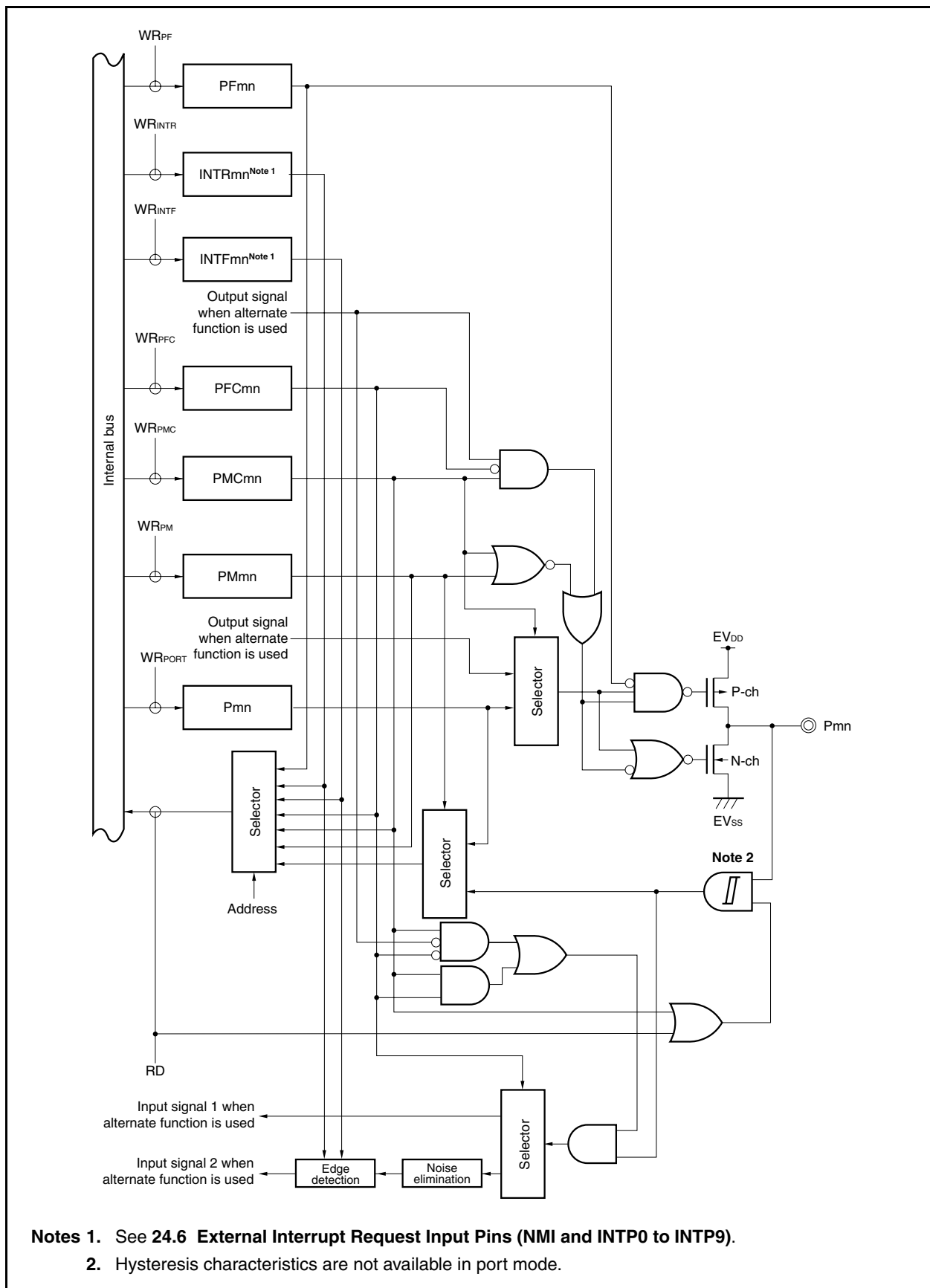
Figure 4-28. Block Diagram of Type N-4
