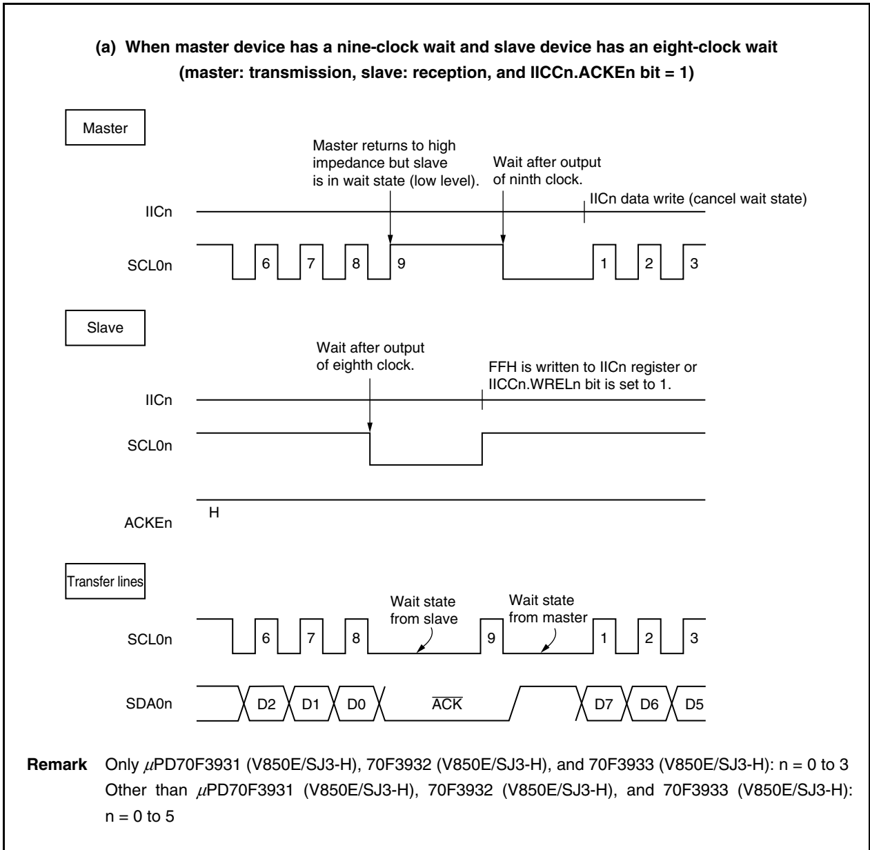
Figure 19-10. Wait State (1/2)
